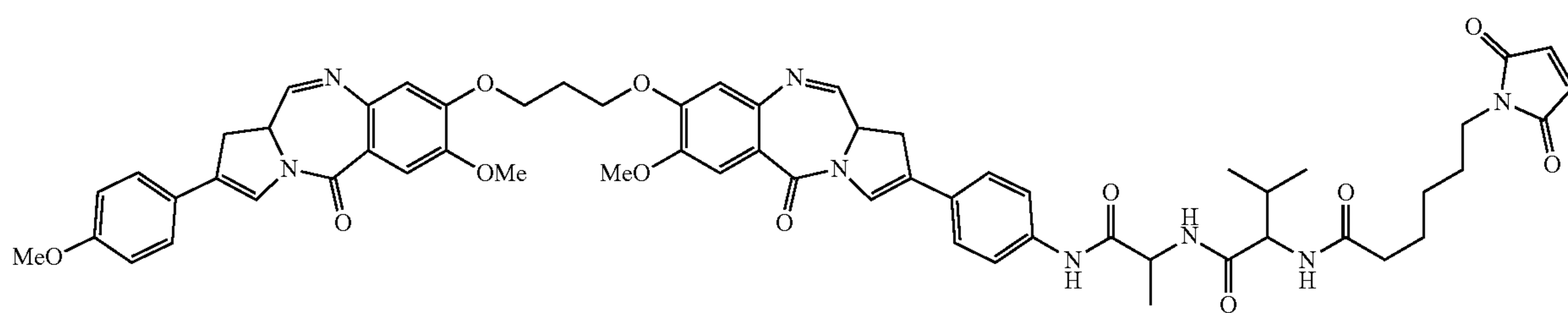
Imine mono-sulfo talirine (isomer 1)
