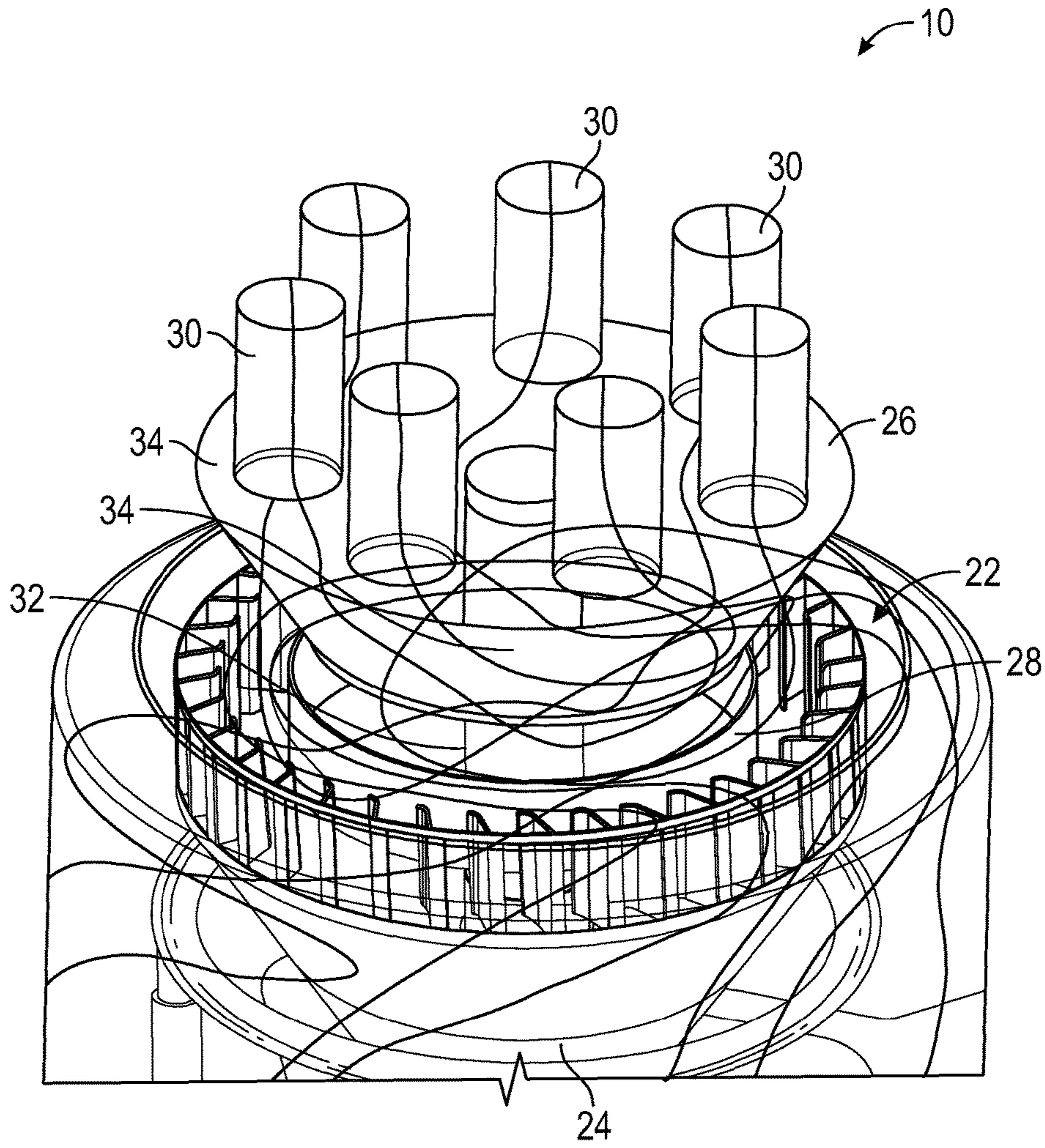
FIG. 3 (Prior Art)
