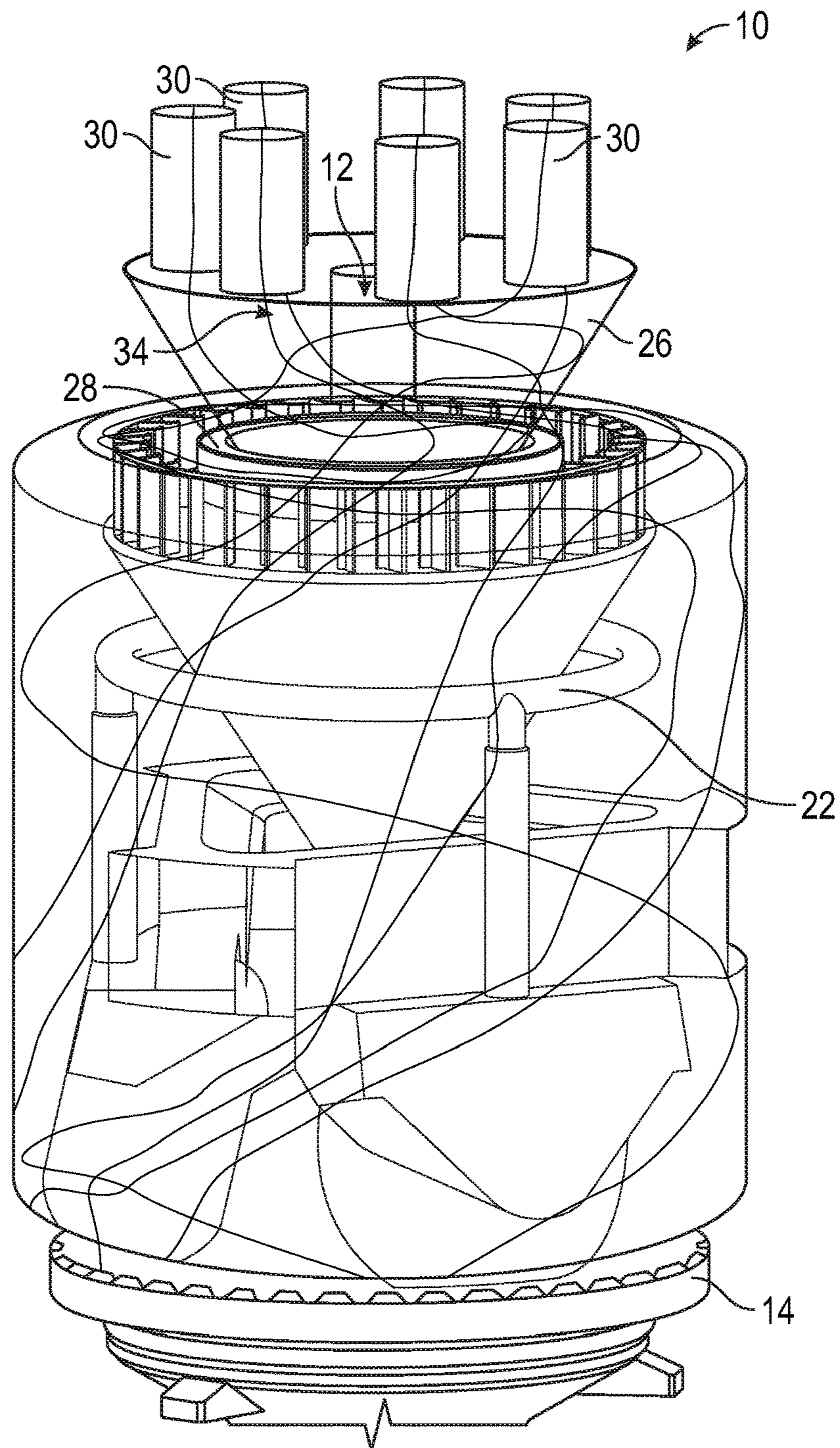
FIG. 2 (Prior Art)
