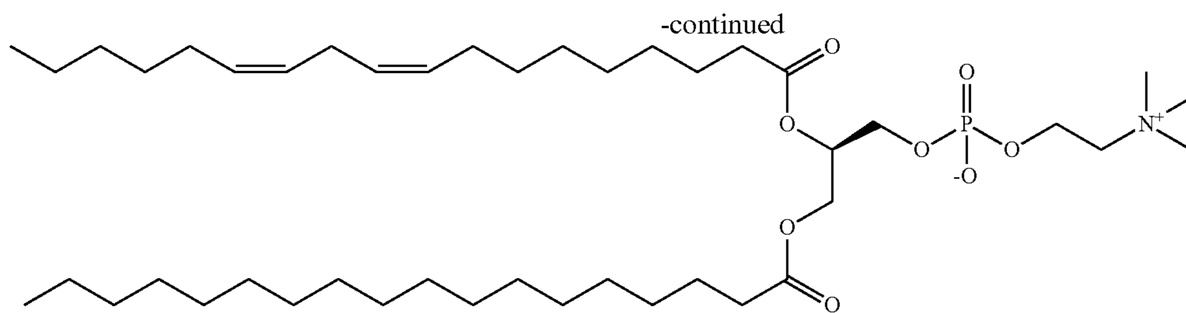
(R)-2-(((9Z,12Z)-octadeca-9,12-dienoyl)oxy)-3-(stearoyloxy)propyl 2-(trimethylammonio)ethyl phosphate ("MPC15")
