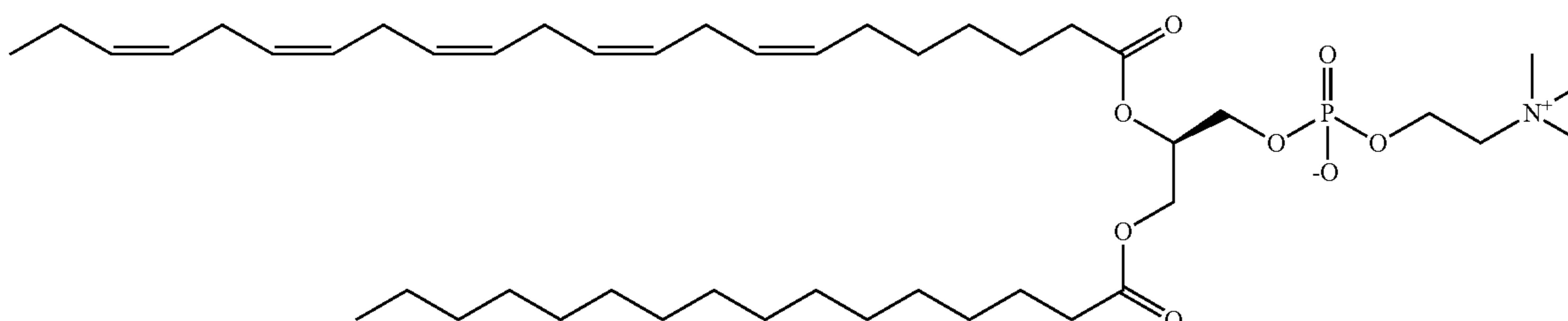
(R)-2-((7Z,10Z,13Z,16Z,19Z)-docosa-7,10,13,16,19-pentaenoyl)oxy-3-(palmitoyloxy)propyl 2-(trimethylammonio)ethyl phosphate ("MPC7")
