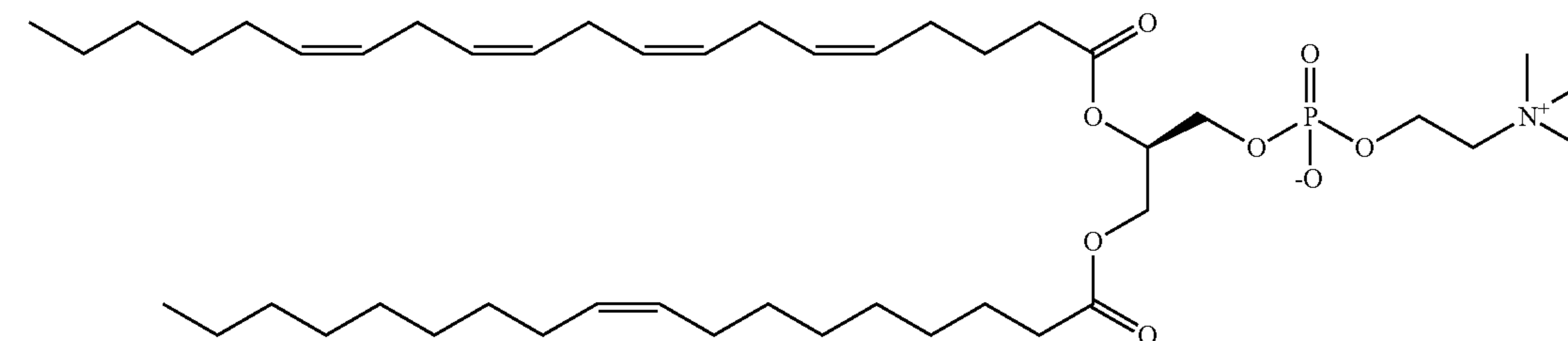
(R)-2-((5Z,8Z,11Z,14Z)-icosa-5,8,11,14-tetraenoyl)oxyoxy-3-(oleoyloxy)propyl 2-(trimethylammonio)ethyl phosphate ("MPC8")
