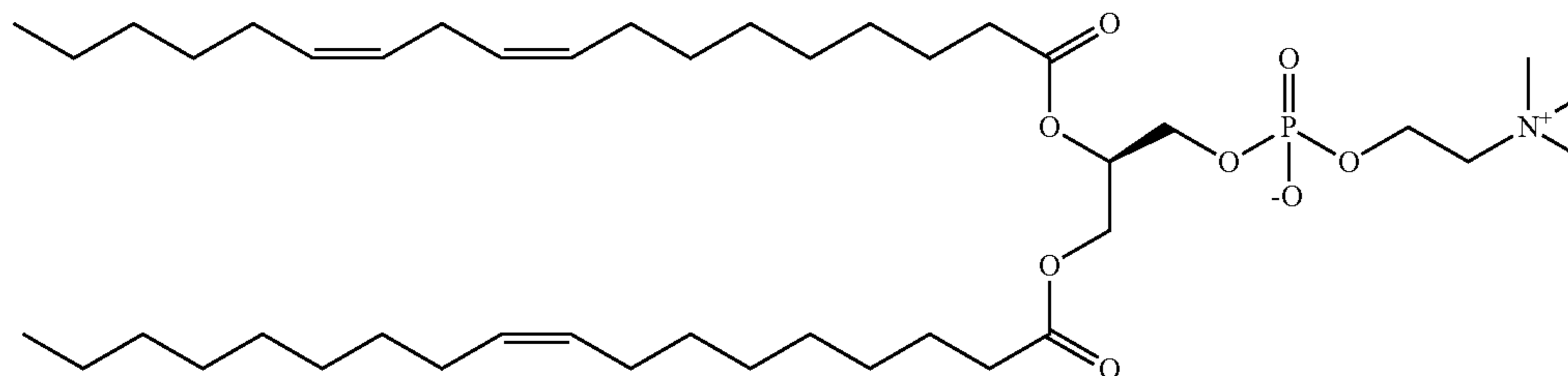
(R)-2-(((9Z,12Z)-octadeca-9,12-dienoyl)oxy)-3-(oleoyloxy)propyl 2-(trimethylammonio)ethyl phosphate ("MPC11")
