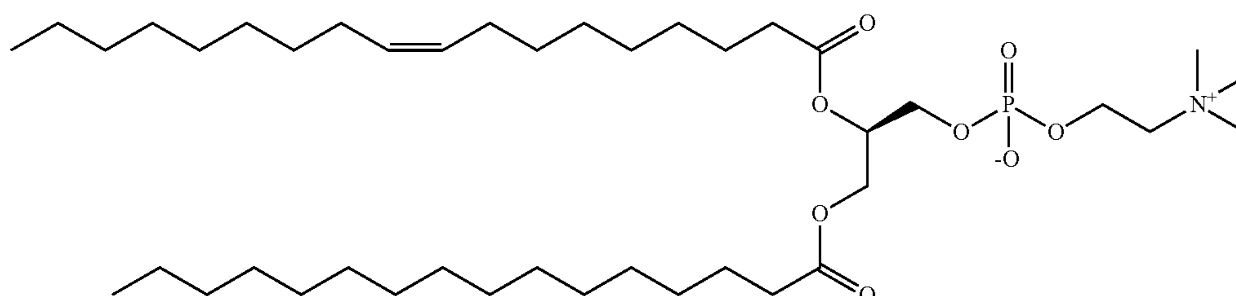
(R)-2-(oleoyloxy)-3-(palmitoyloxy)propyl 2-(trimethylammonio)ethyl phosphate ("MPC14")
