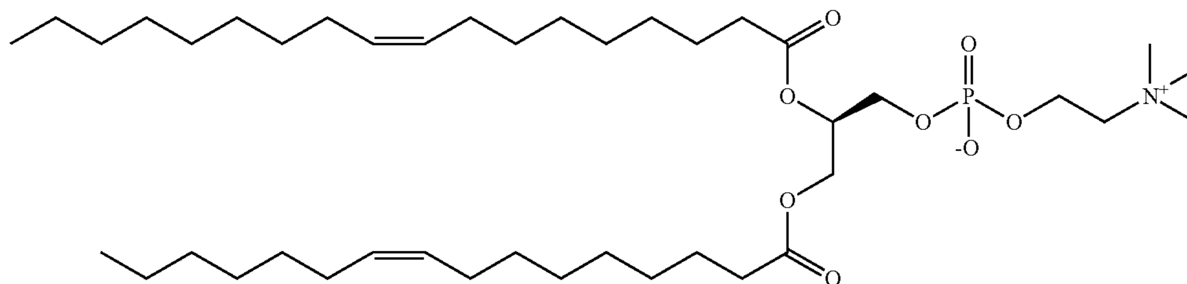
(R)-2-((Z)-octadeca-9-enoyl)oxy)-3-((Z)-hexadec-9-enoyl)oxy)propyl 2-(trimethylammonio)ethyl phosphate ("MPC10")
