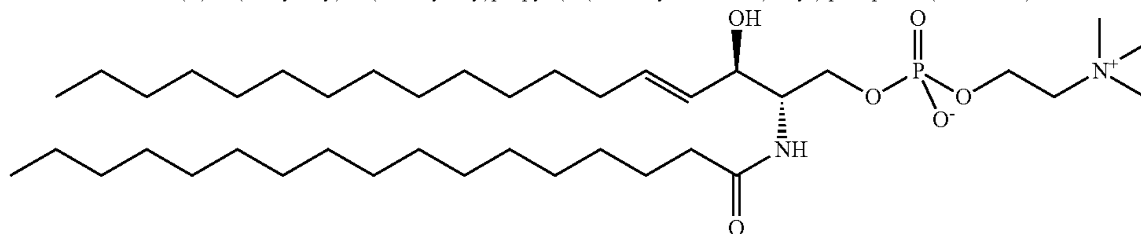
(2S,3R,E)-2-heptadecanamido-3-hydroxyoctadec-4-en-1-yl 2-(trimethylammonio)ethyl phosphate ("SPH1")
