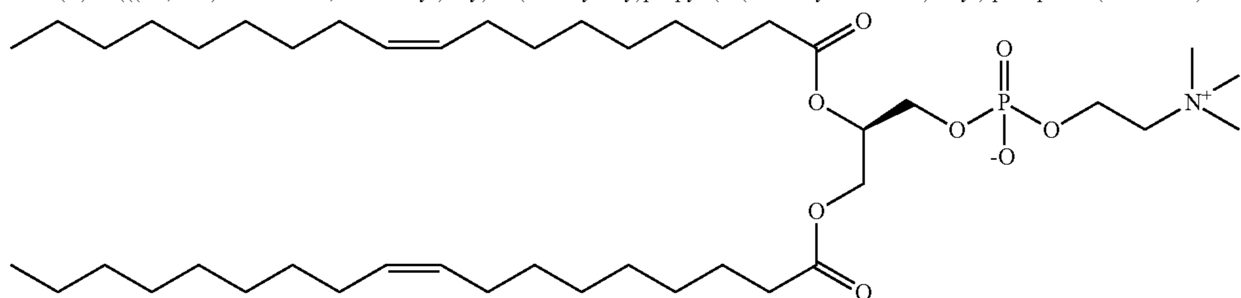
(R)-2,3-bis(oleoyloxy)propyl 2-(trimethylammonio)ethyl phosphate ("MPC16")
