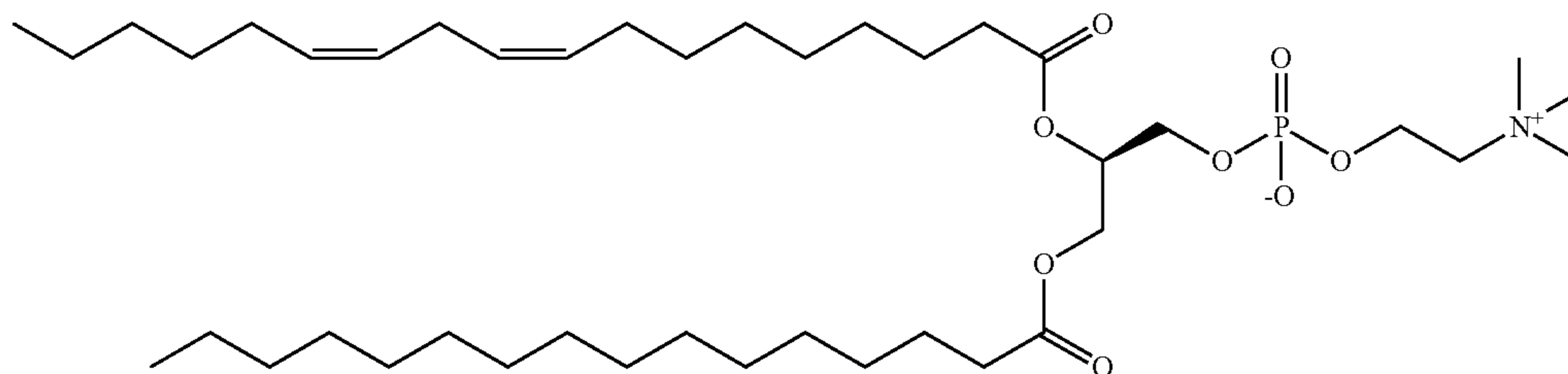
(R)-2-(((9Z,12Z)-octadeca-9,12-dienoyl)oxy)-3-(palmitoyloxy)propyl 2-(trimethylammonio)ethyl phosphate ("MPC9")
