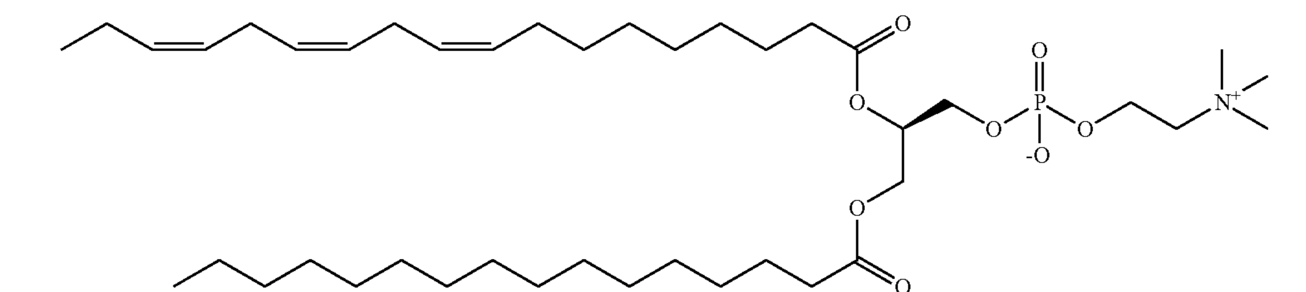
(R)-2-((9Z,12Z,15Z)-octadeca-9,12,15-trienoyl)oxy-3-((Z)-hexadec-9-enoyl)propyl 2-(trimethylammonio)ethyl phosphate ("MPC3")
