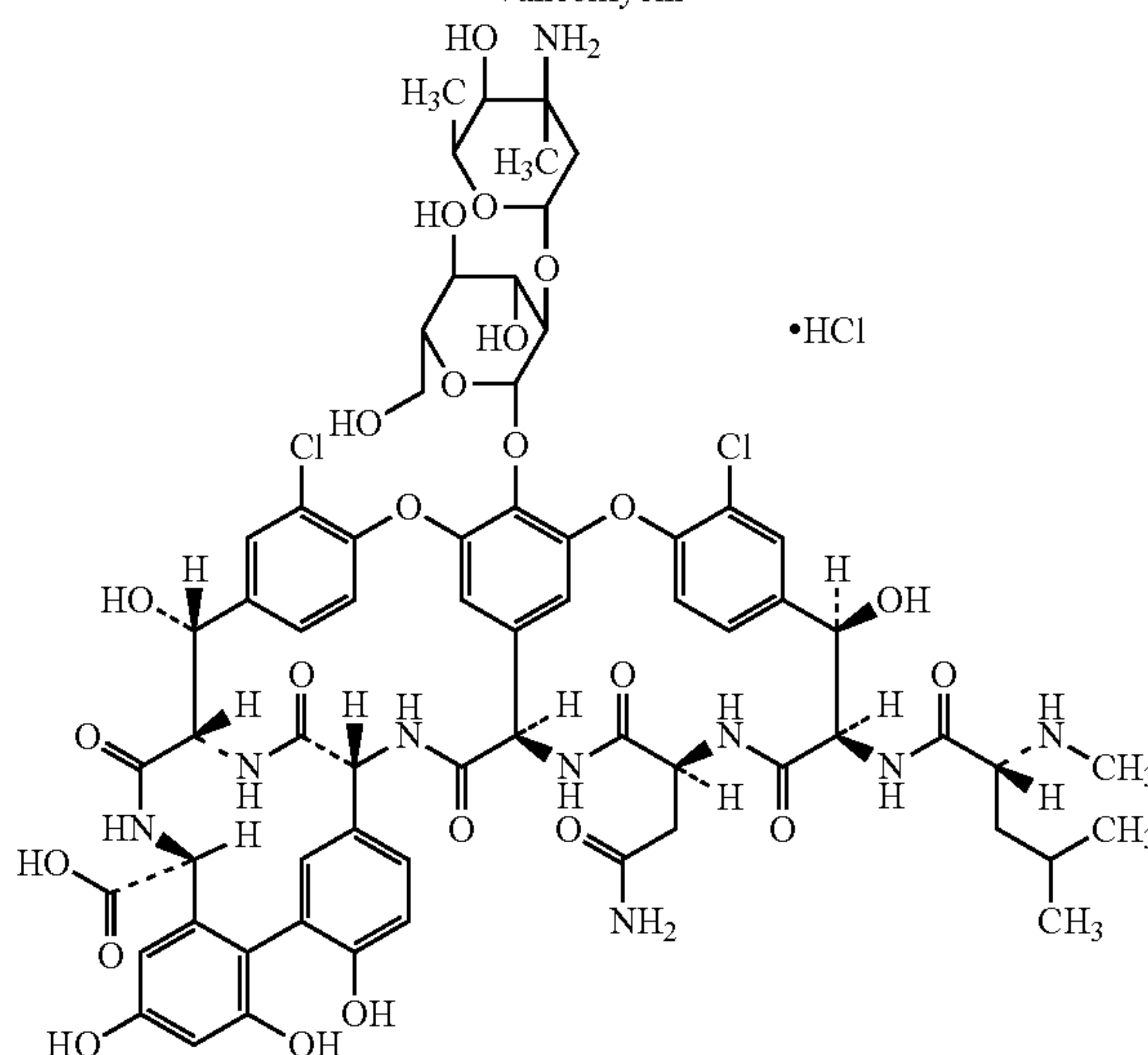
Vancomycin hydrochloride
