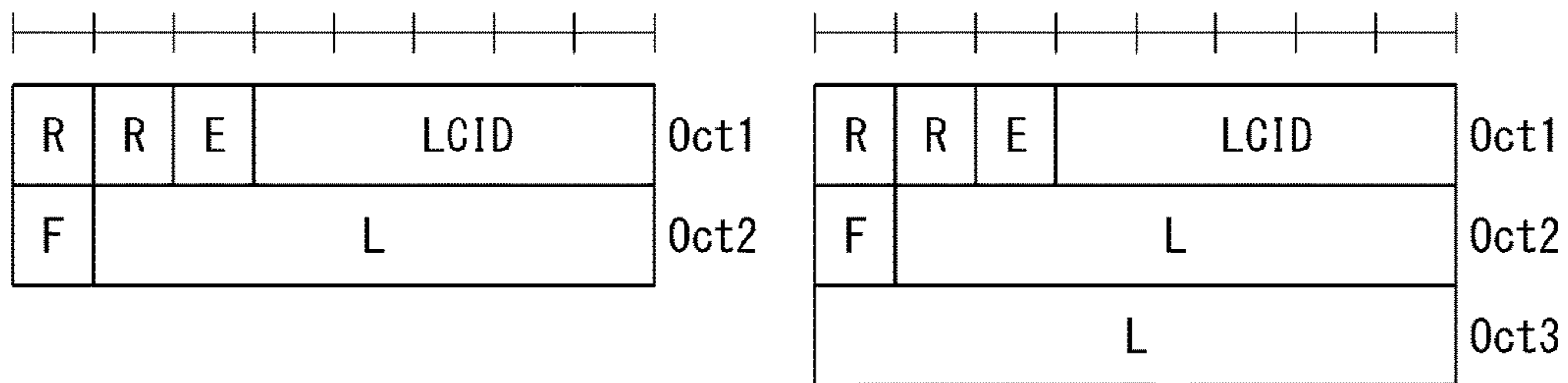
(a) R/R/E/LCID/F/L sub-header with 7-bit Lfield
