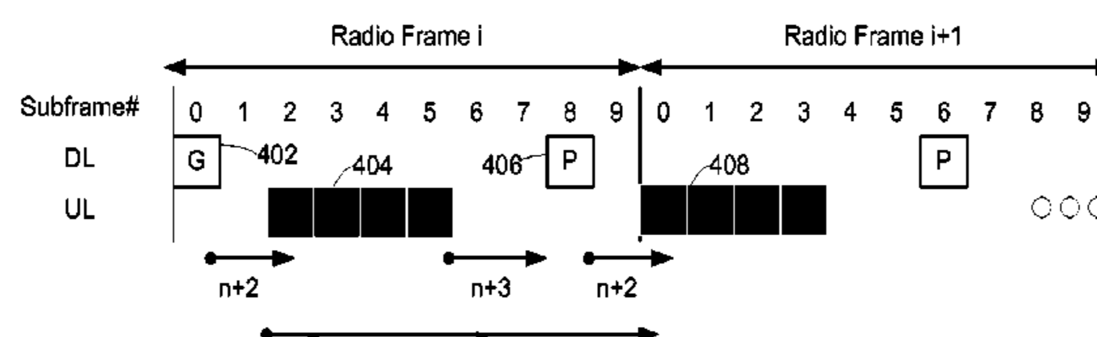
TTI bundling (size 4): re-transmission delay every 8 subframes for co-existence with legacy Synchronous HARQ / UE's
