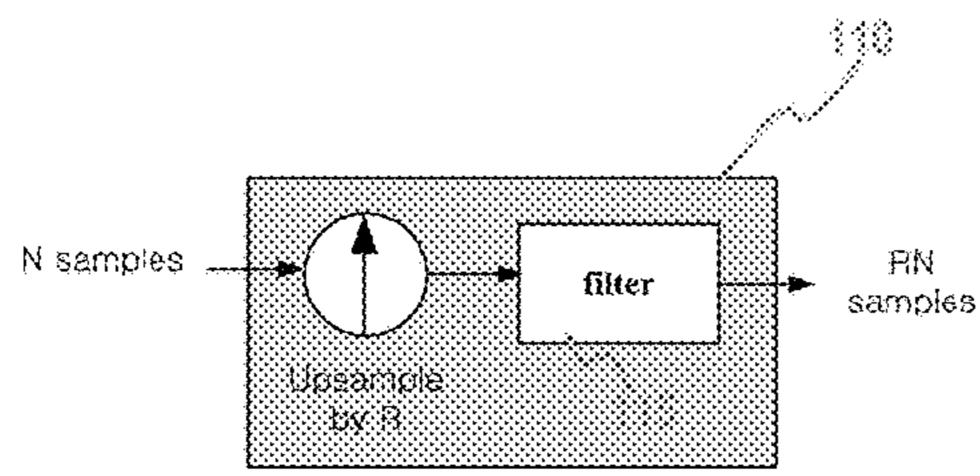
Interpolator
