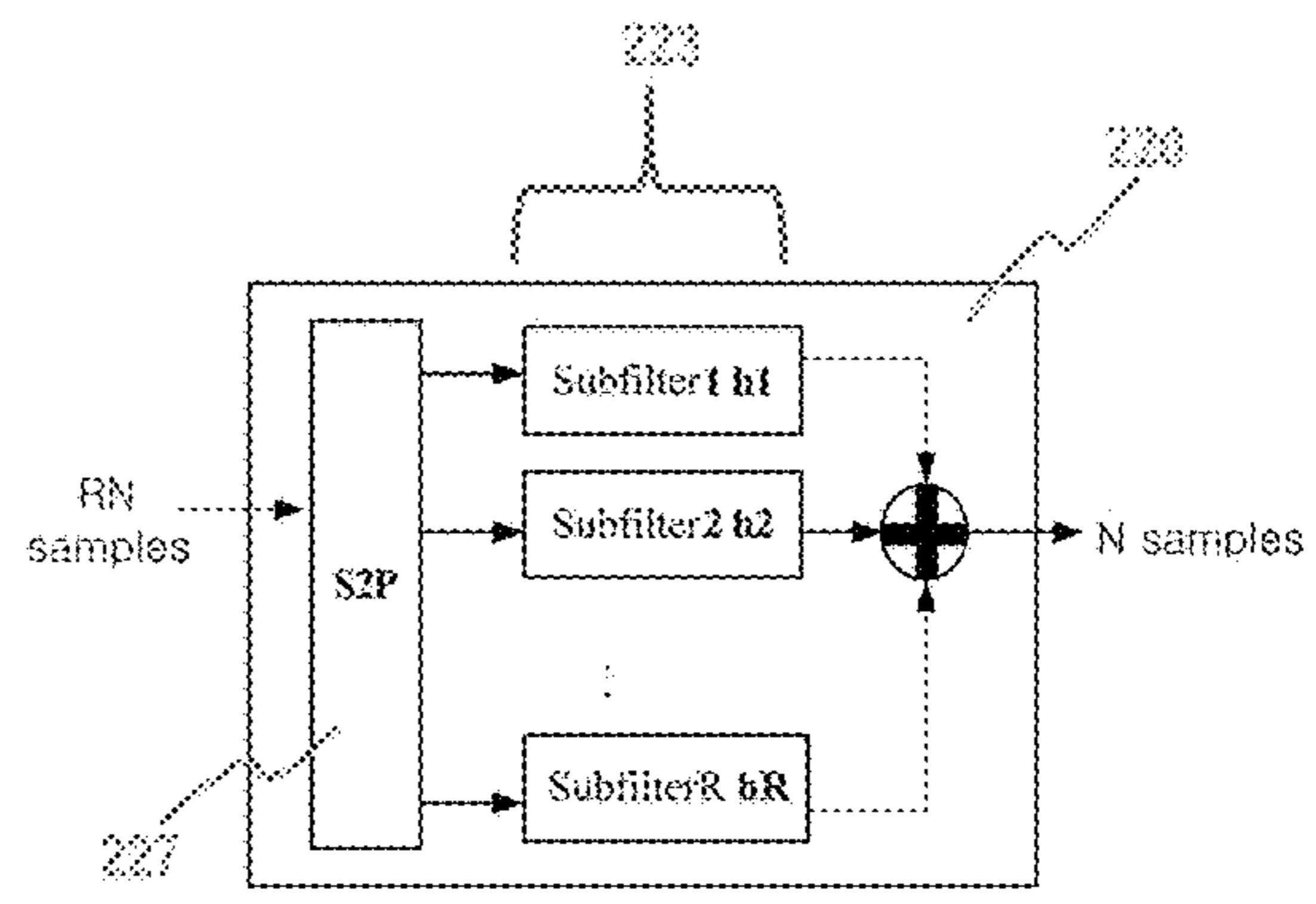
Polyphase Decimator
