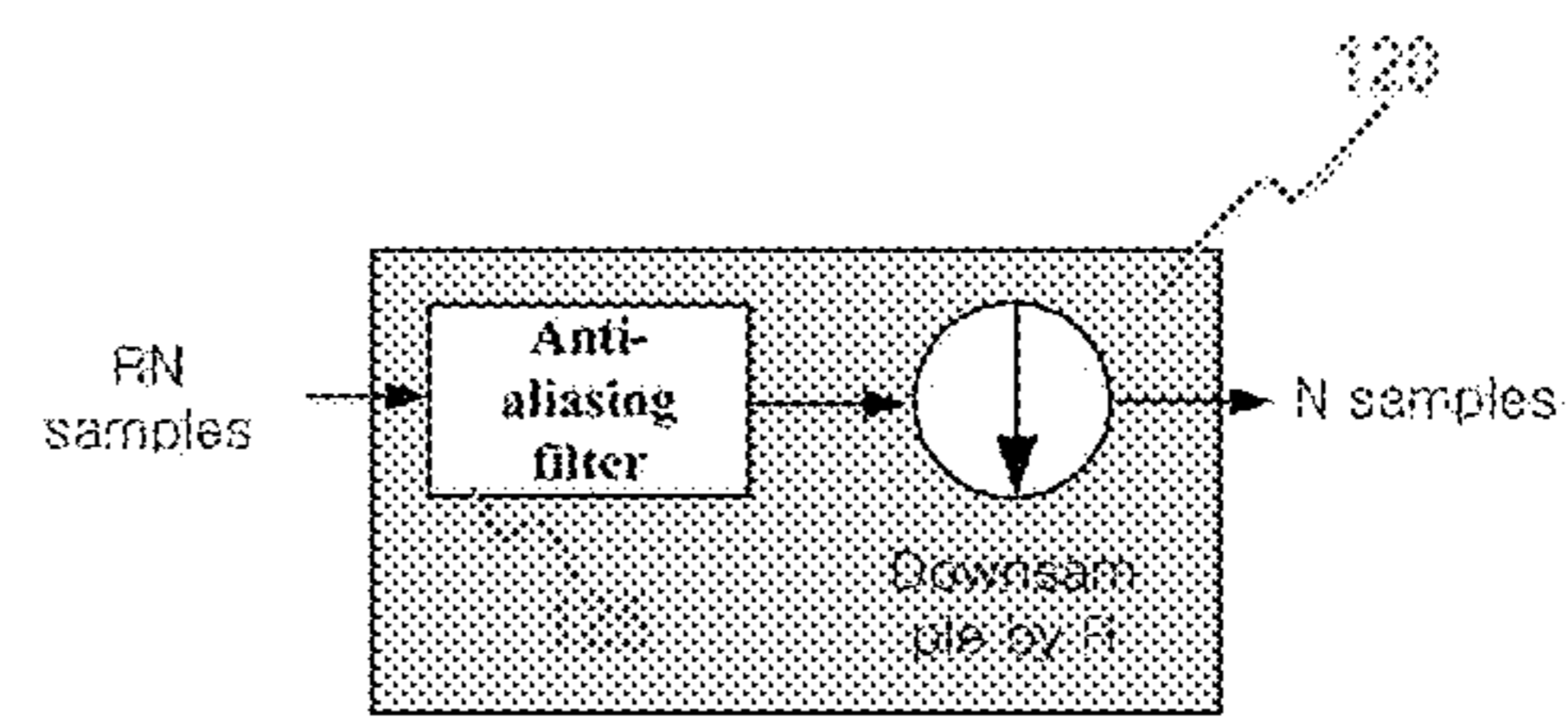
Decimator
