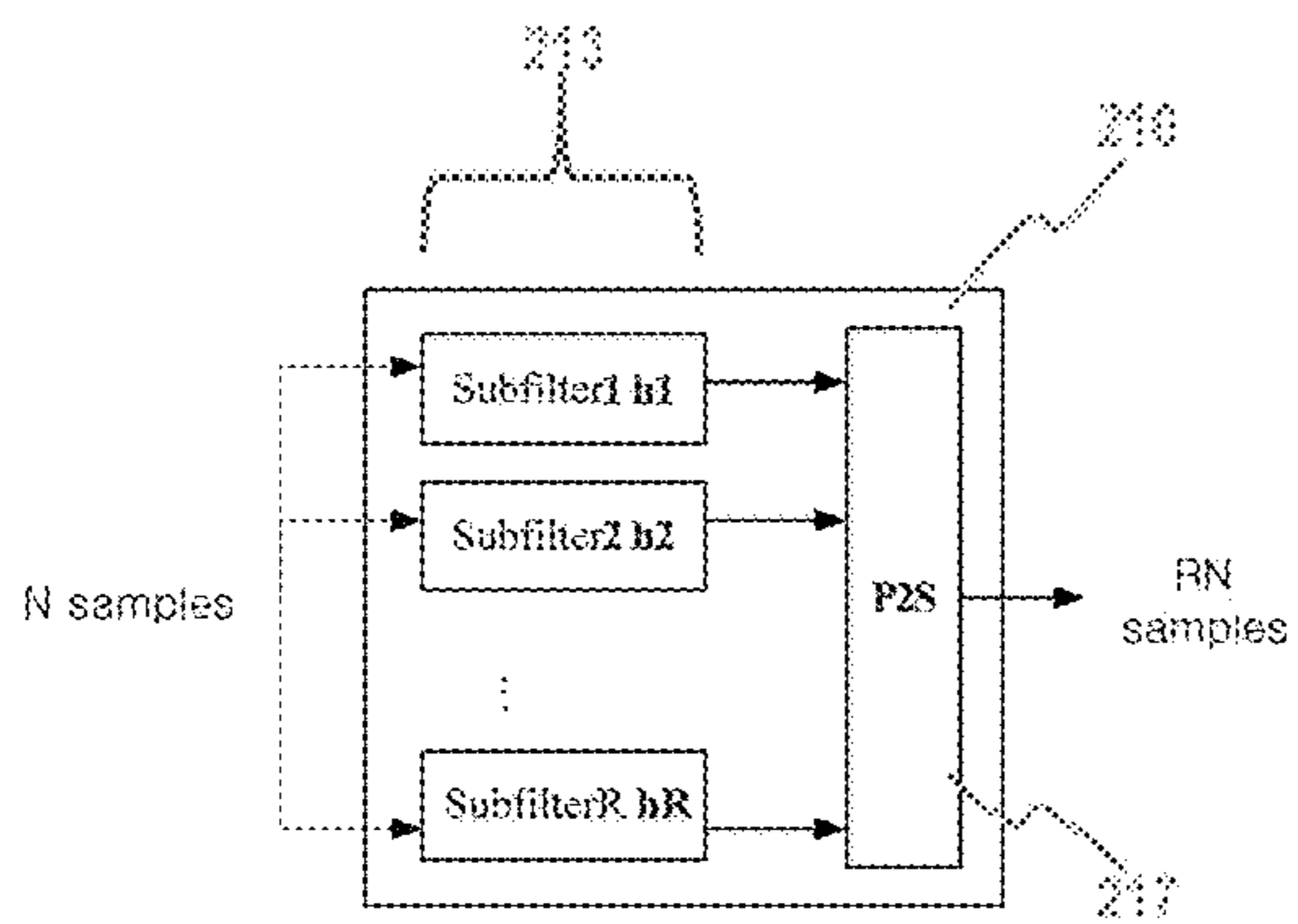
Polyphase Interpolator
