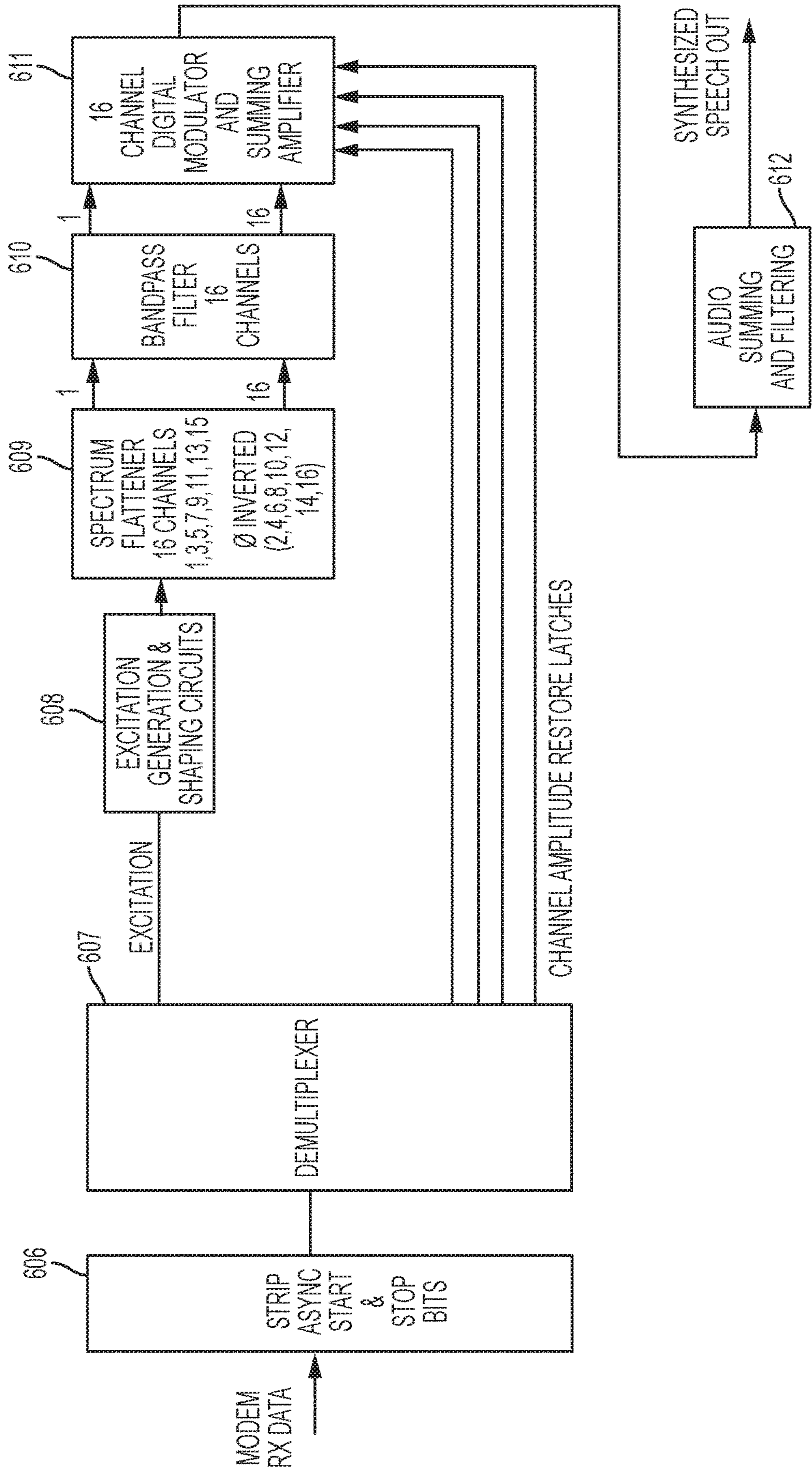
CHANNEL VOCODER RECEIVER
