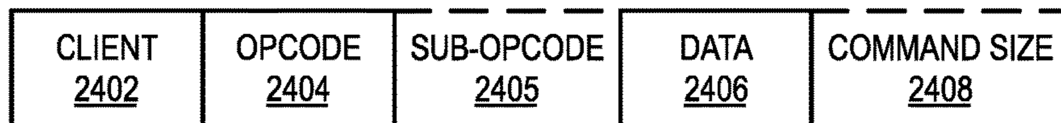
GRAPHICS PROCESSOR COMMAND FORMAT 2400
