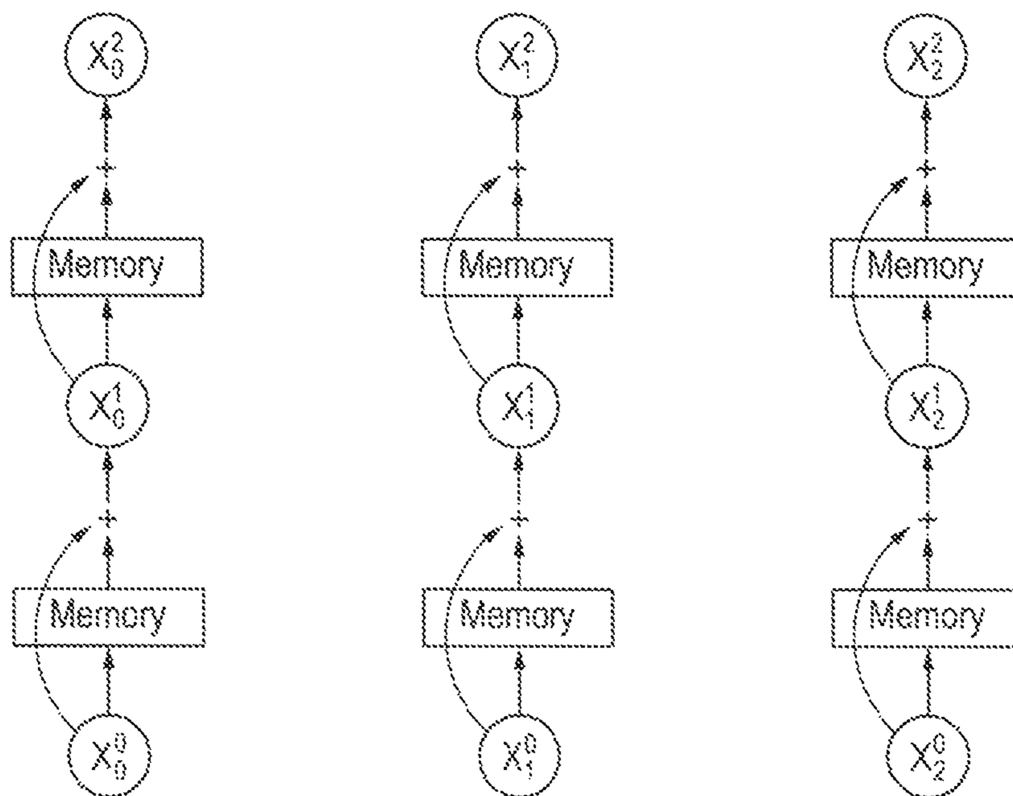
Neural Network
