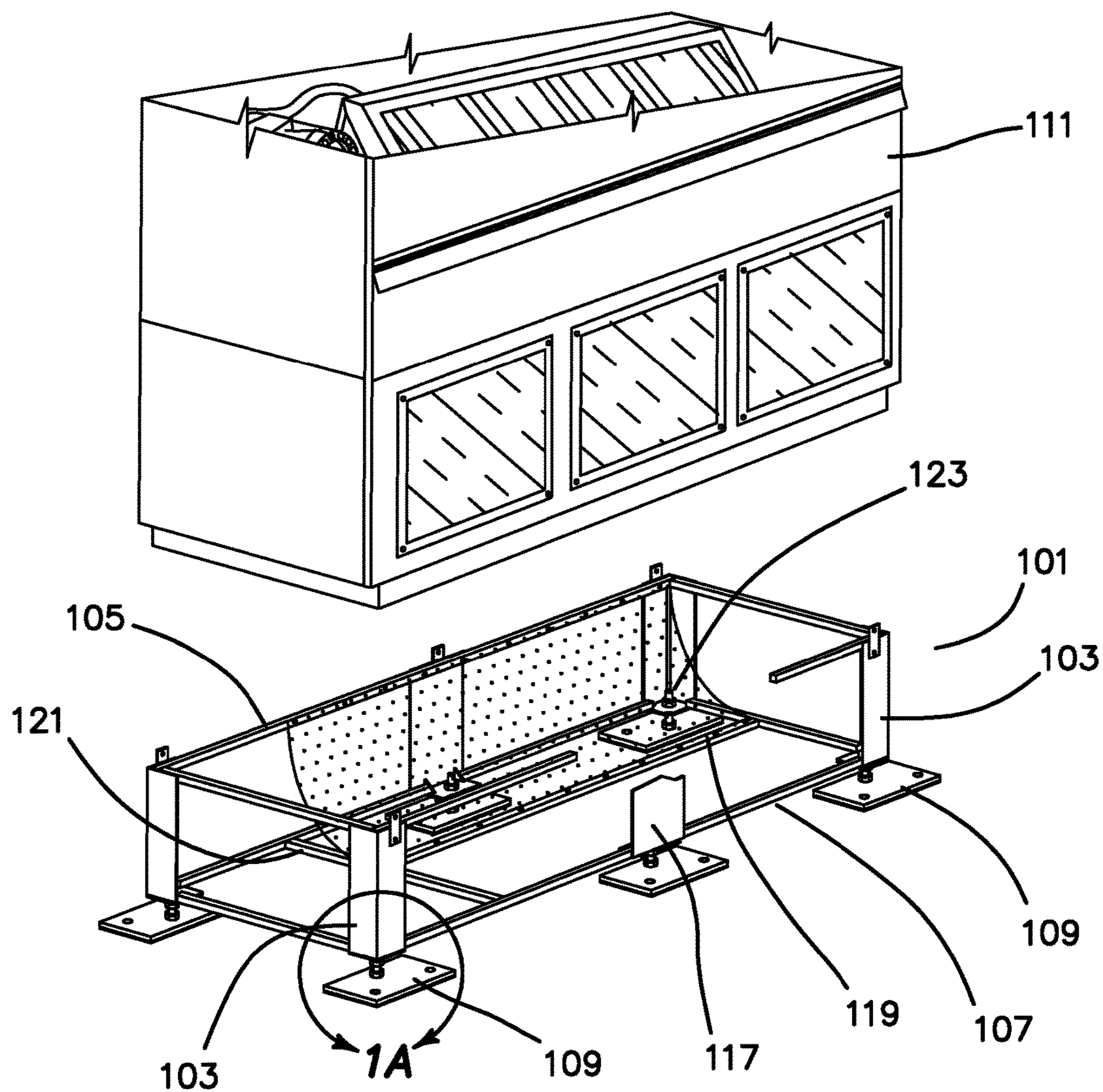
FIG. 1 PRIOR ART
