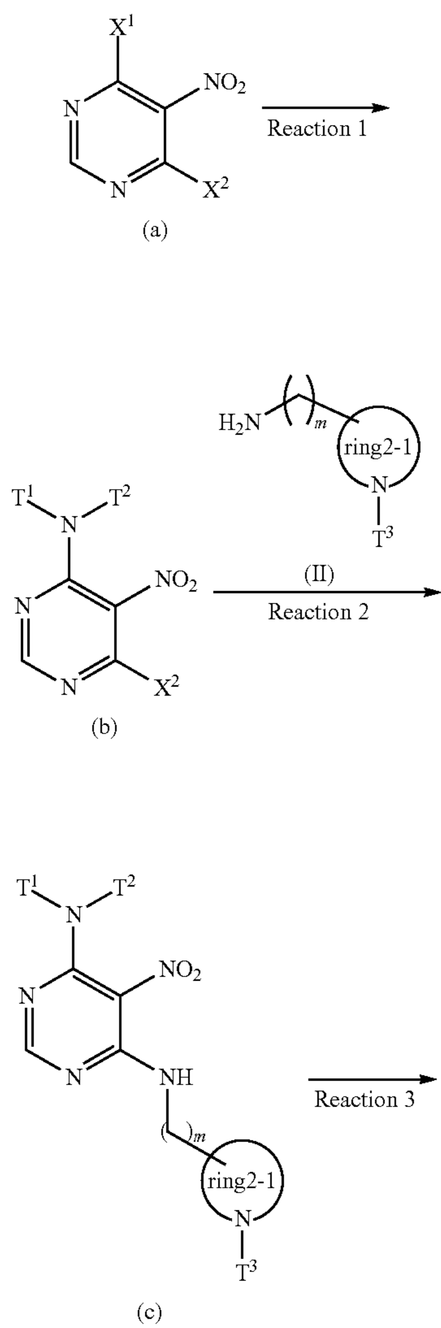
Reaction scheme 1
