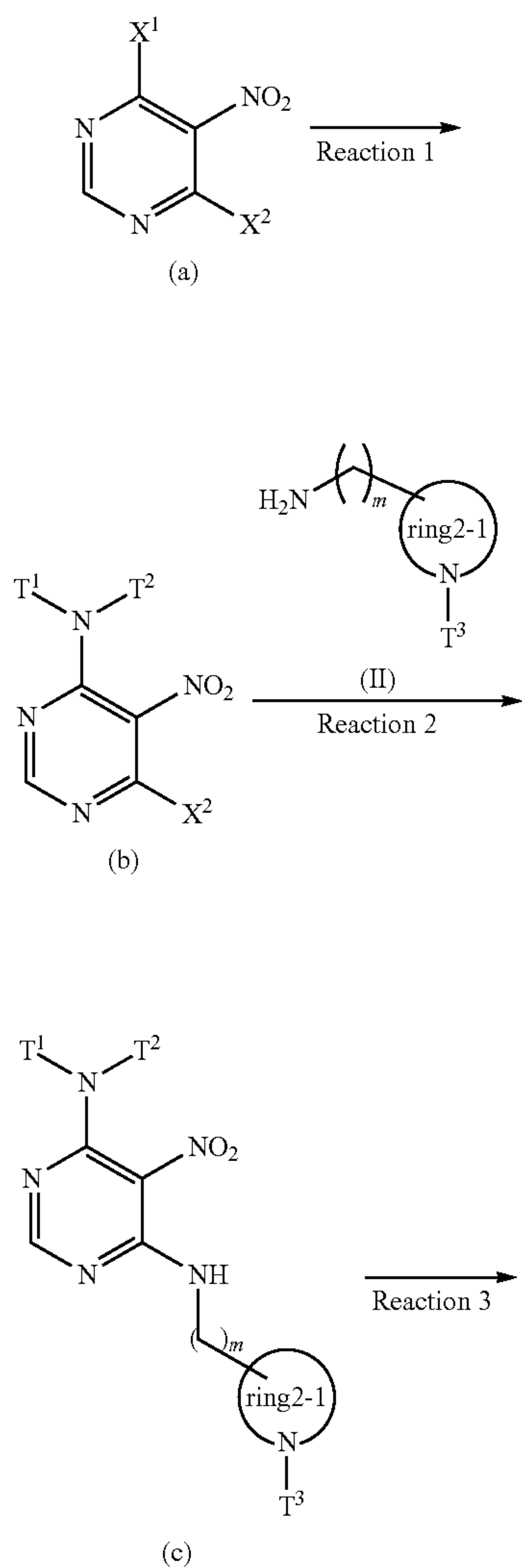
Reaction scheme 1
