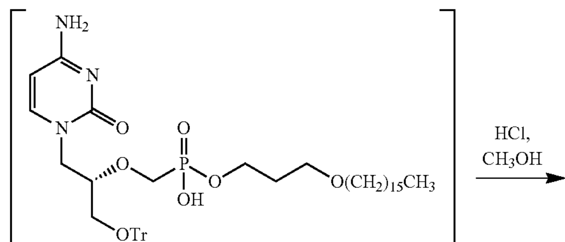
Compound 3
