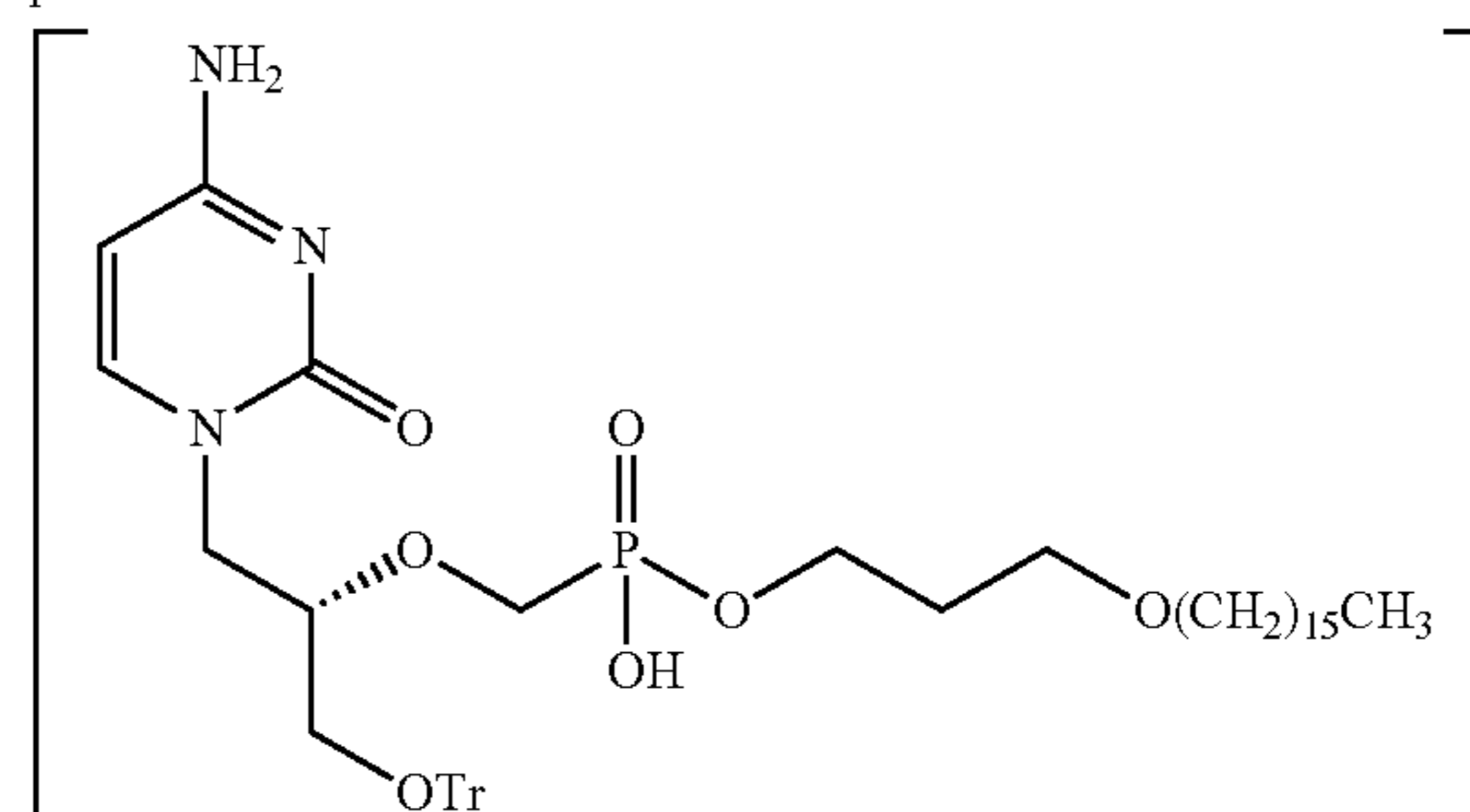
Compound 3
