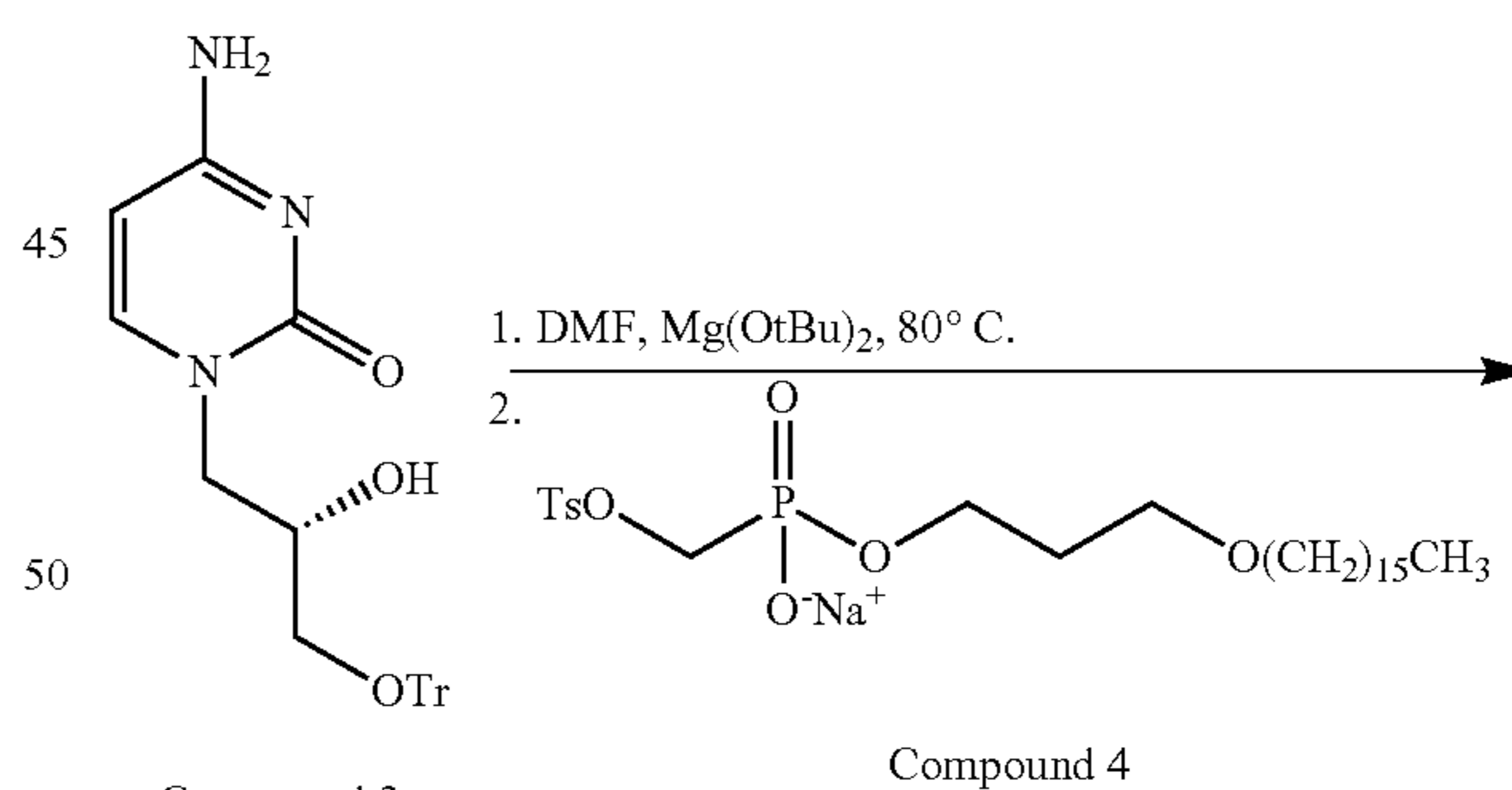
Compound 2
