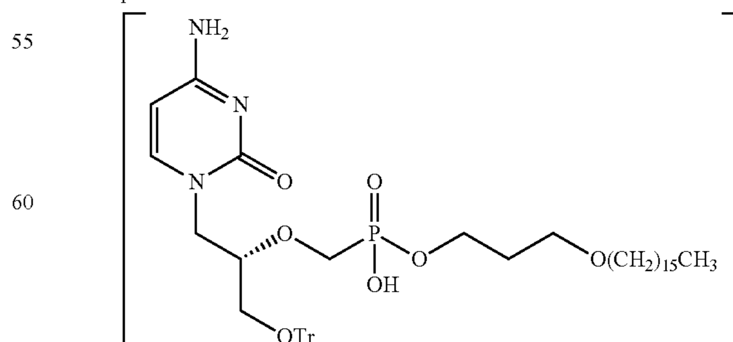
Compound 3
