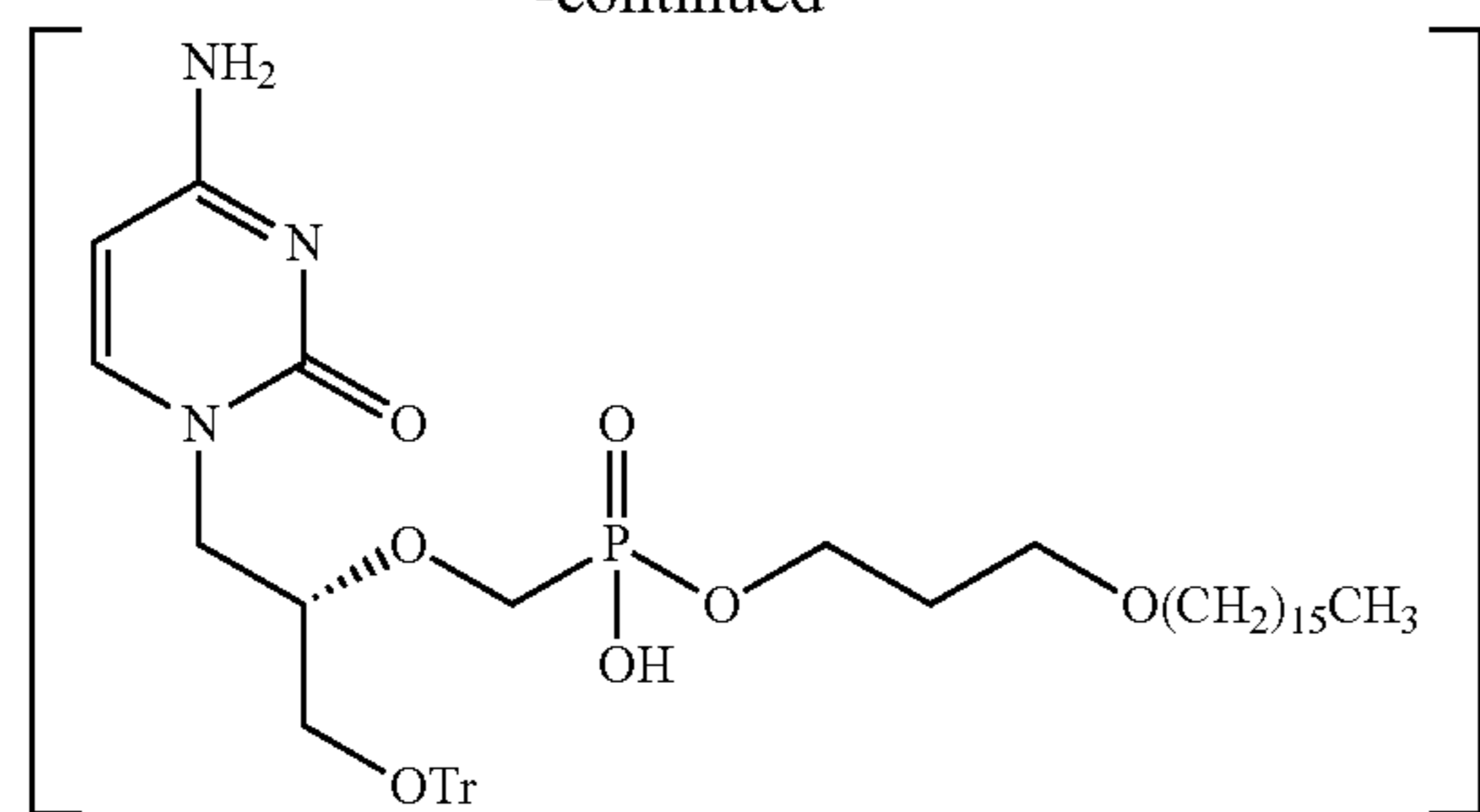
Compound 3
