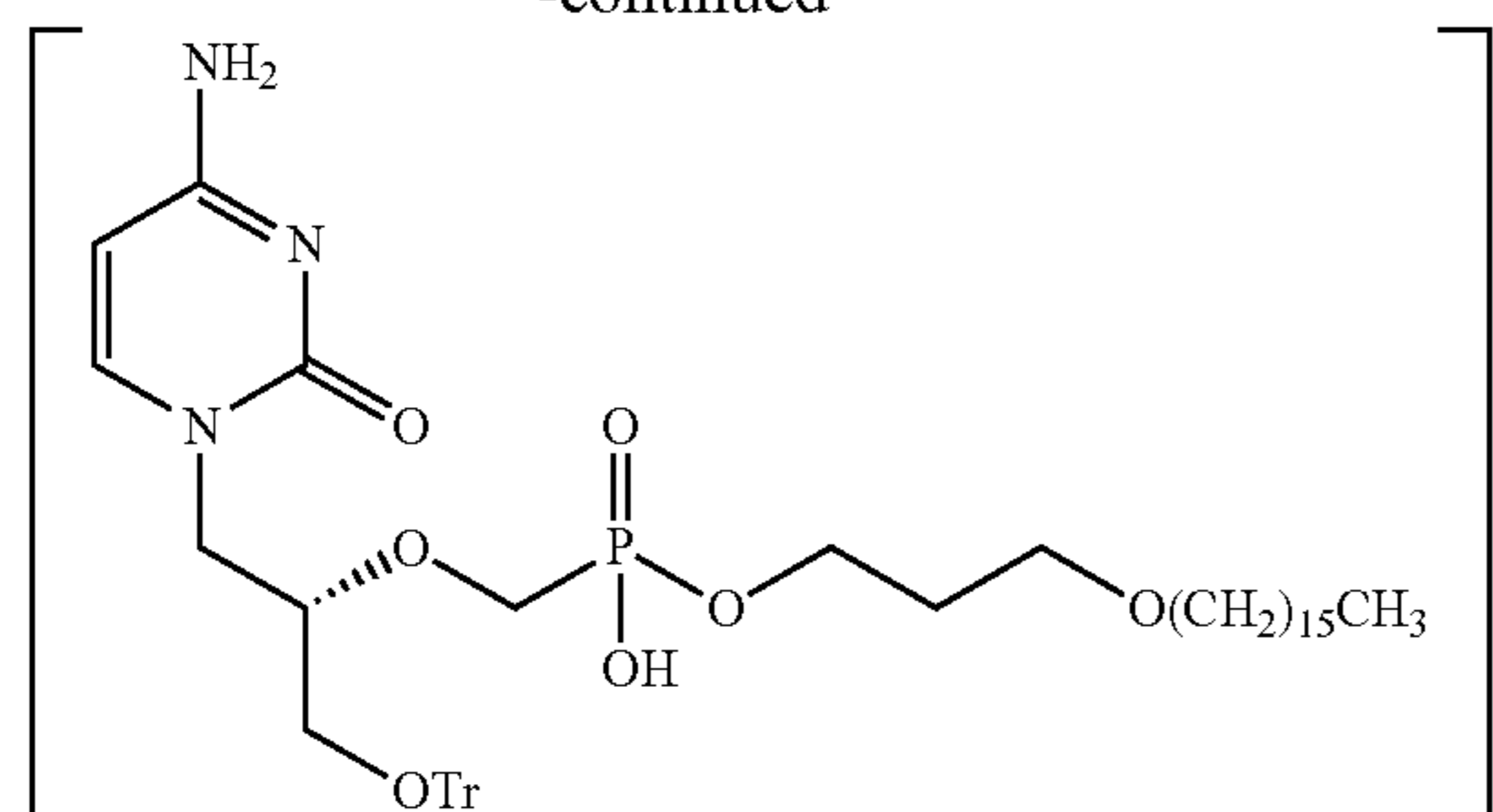
Compound 3
