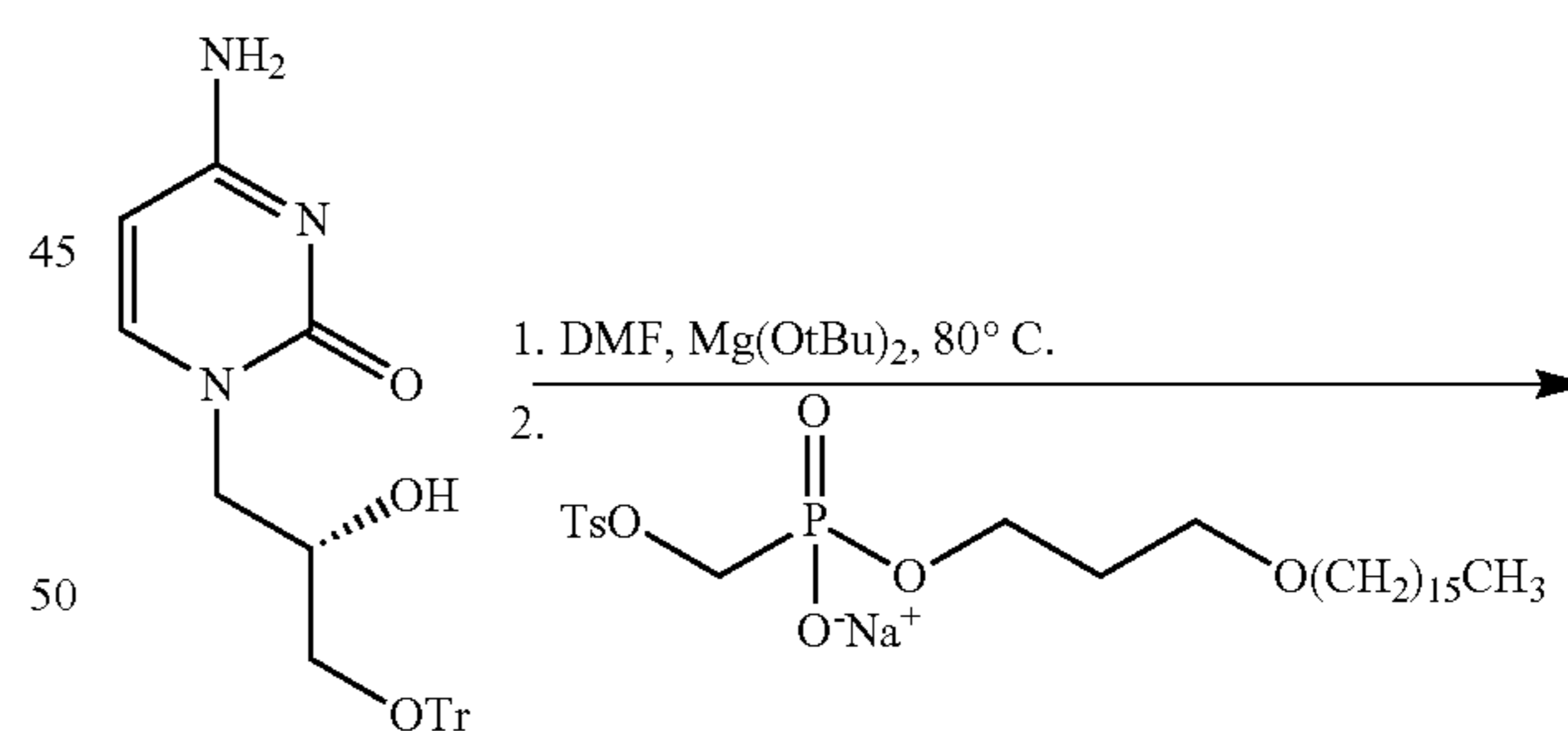
Compound 4
