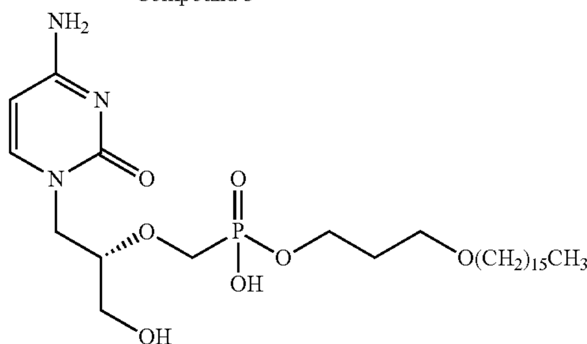
Compound 1
