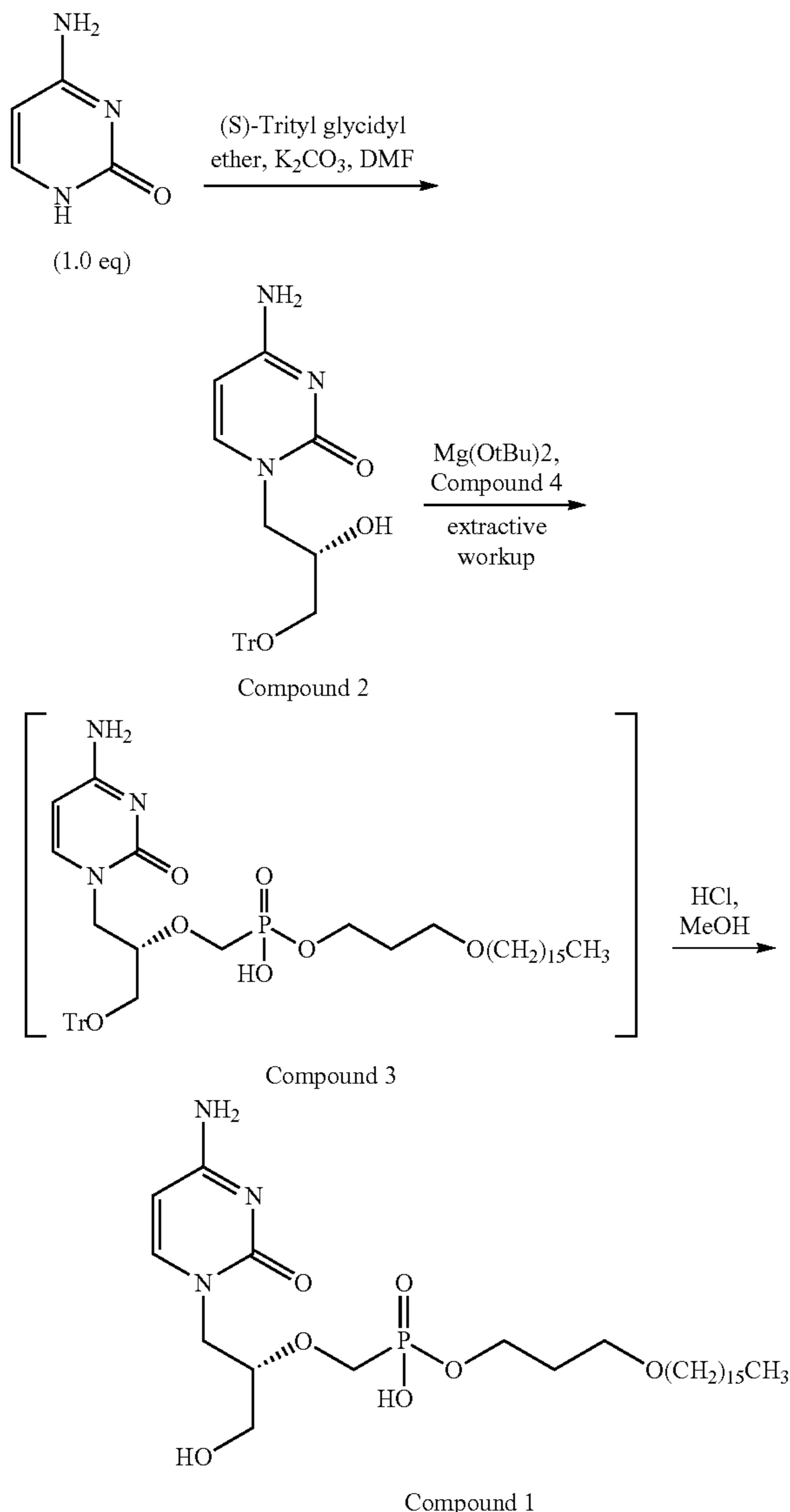
Scheme 1
