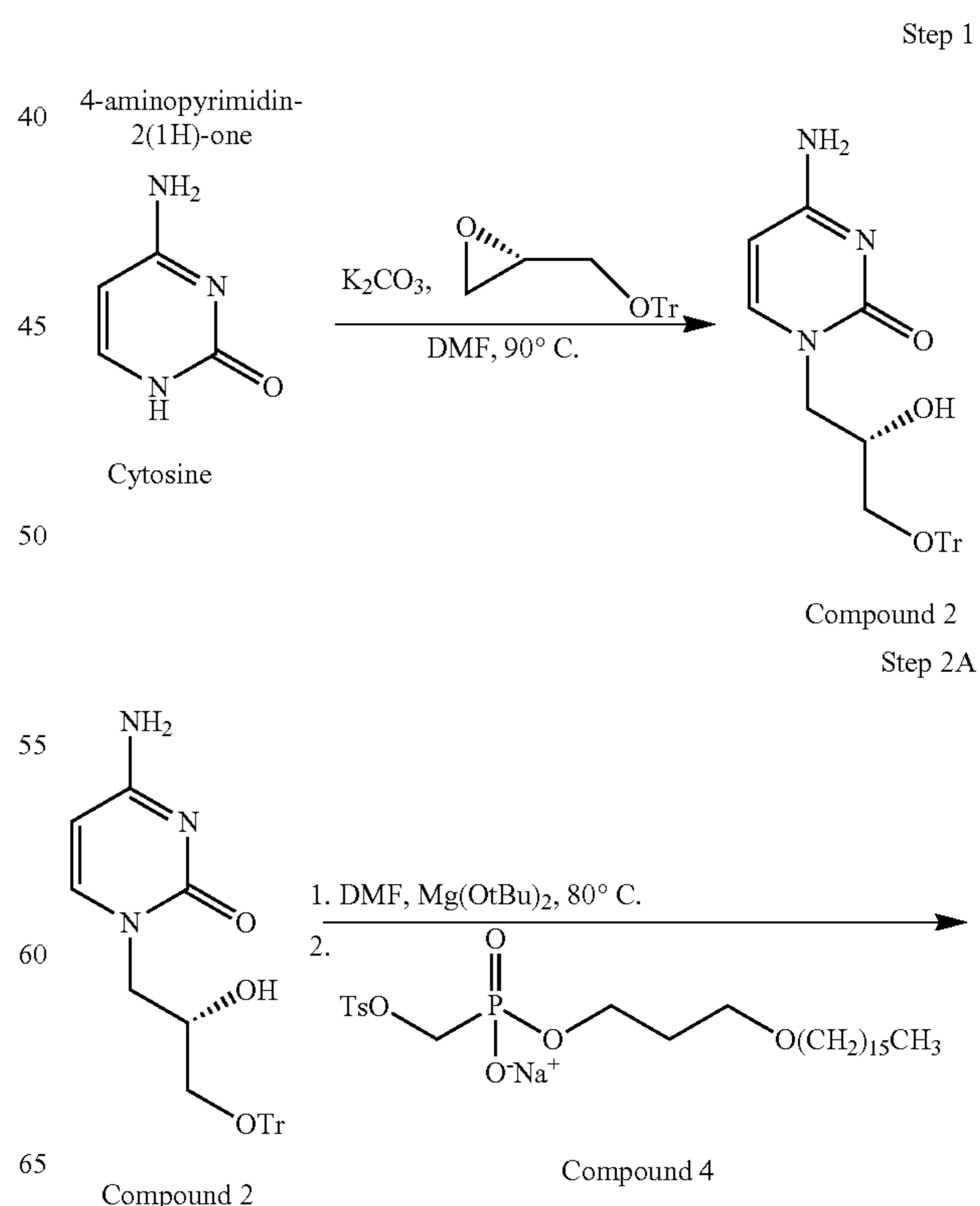
Scheme 1
