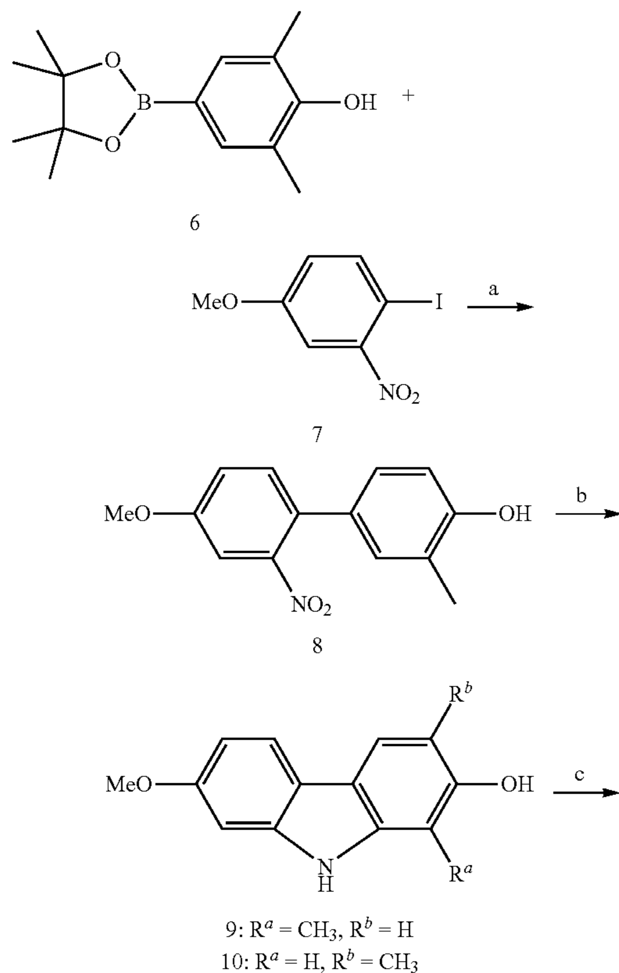
Scheme 2:
