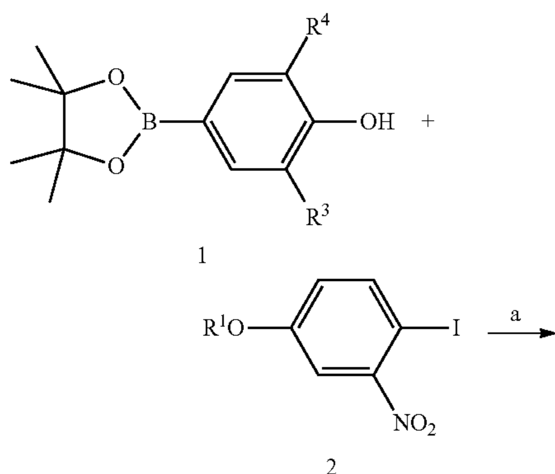
Scheme 1:
