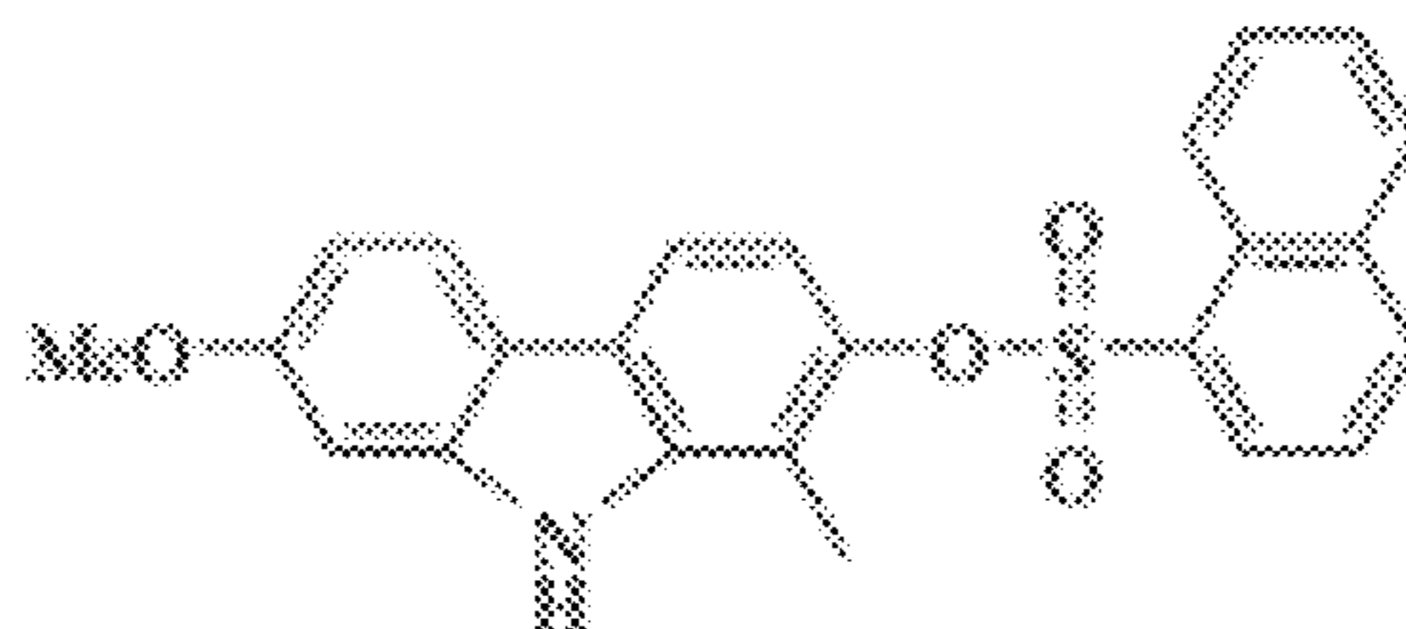
SH-I-125
