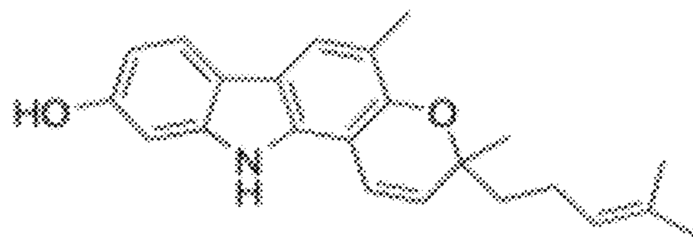
Mahanine
