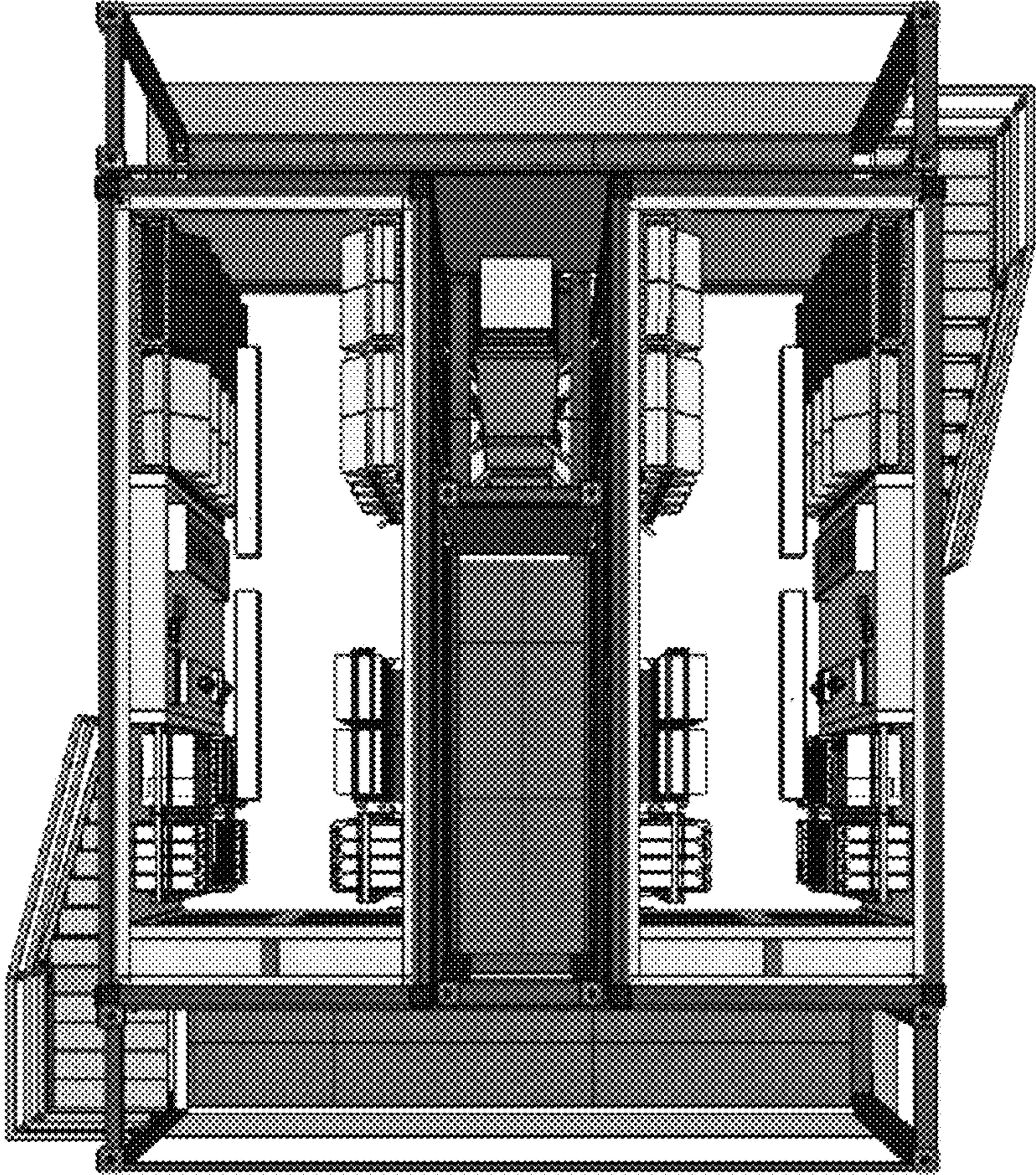
FIG. 46 Co-Located Site Stack-Configuration (Top View)
