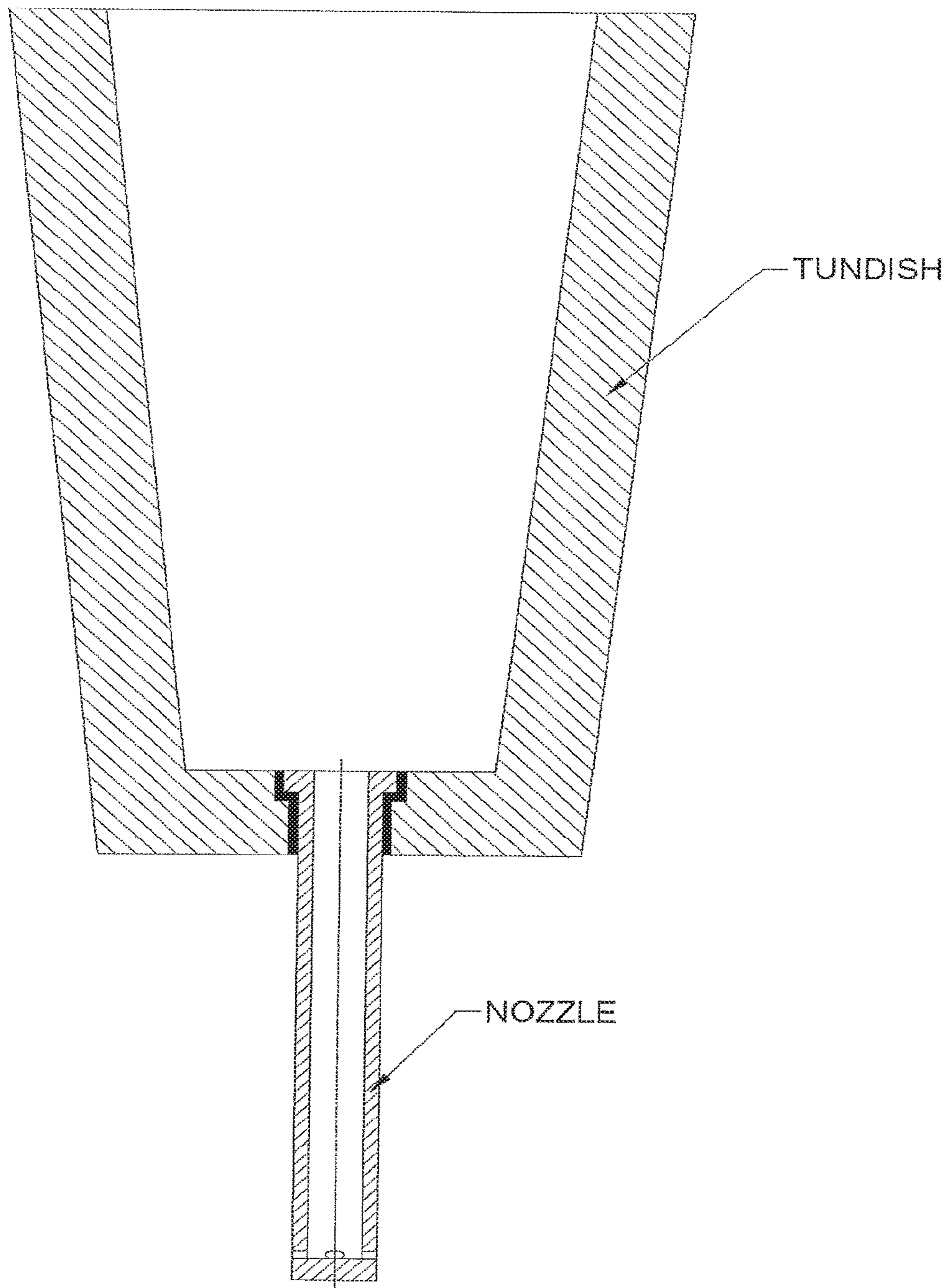
Figure 4. Tundish arrangement
