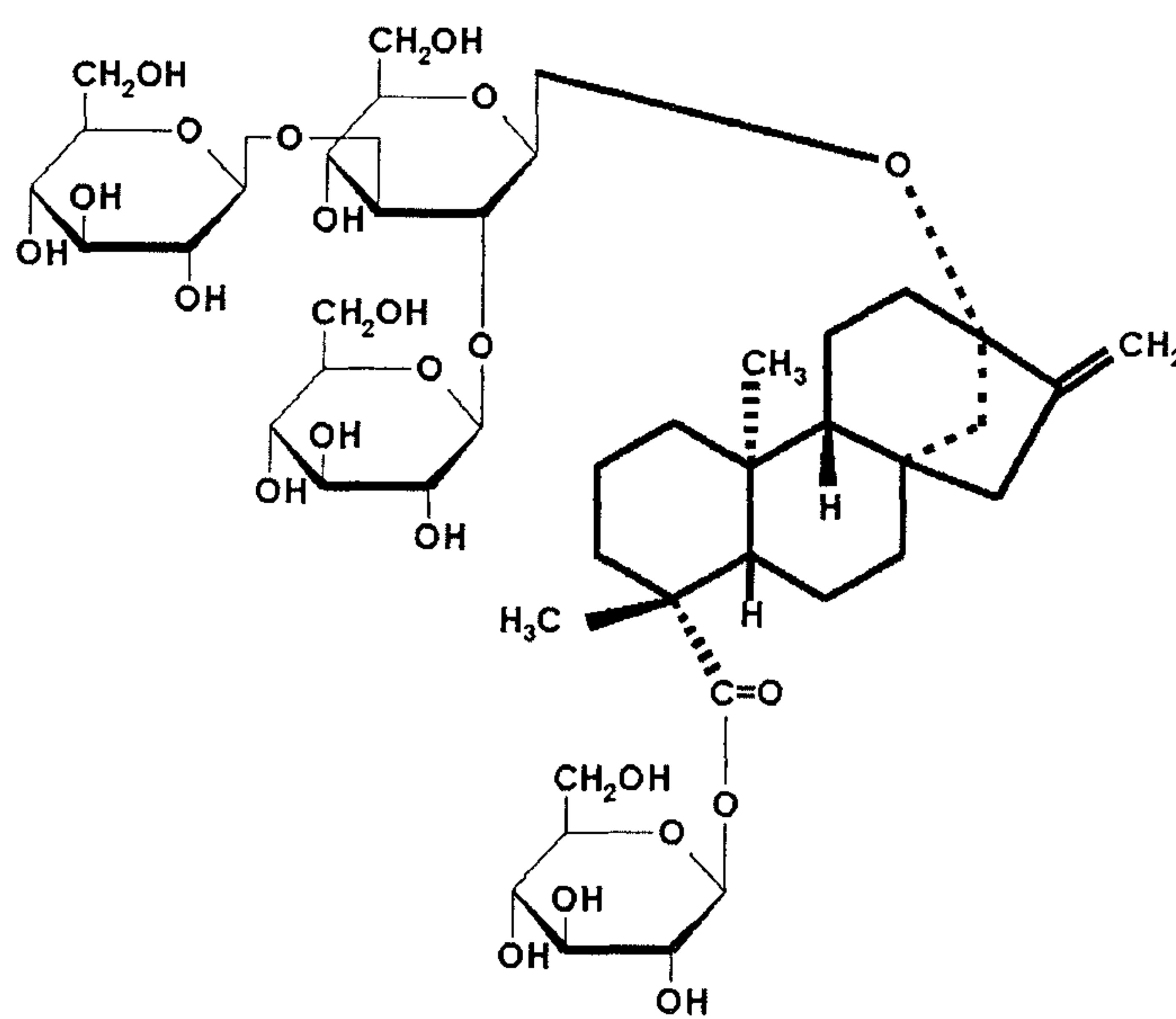
Rebaudioside A
