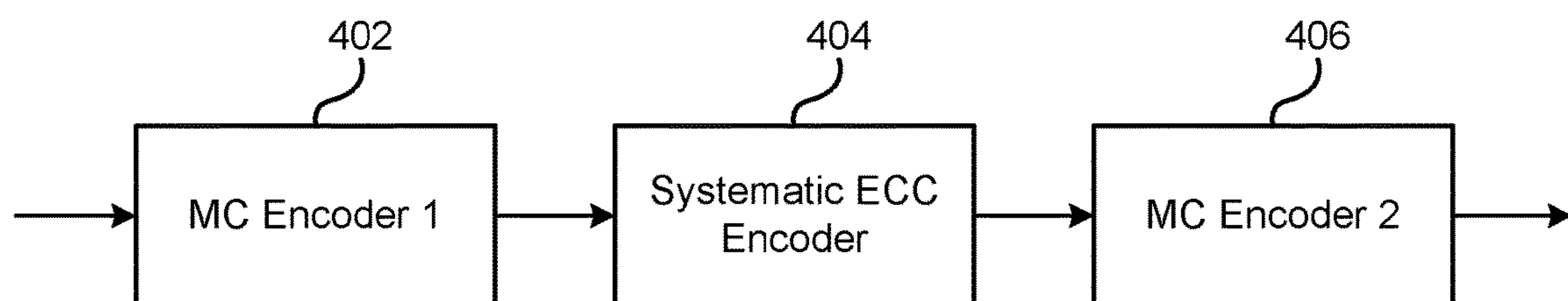
FIG. 4 (prior art)
