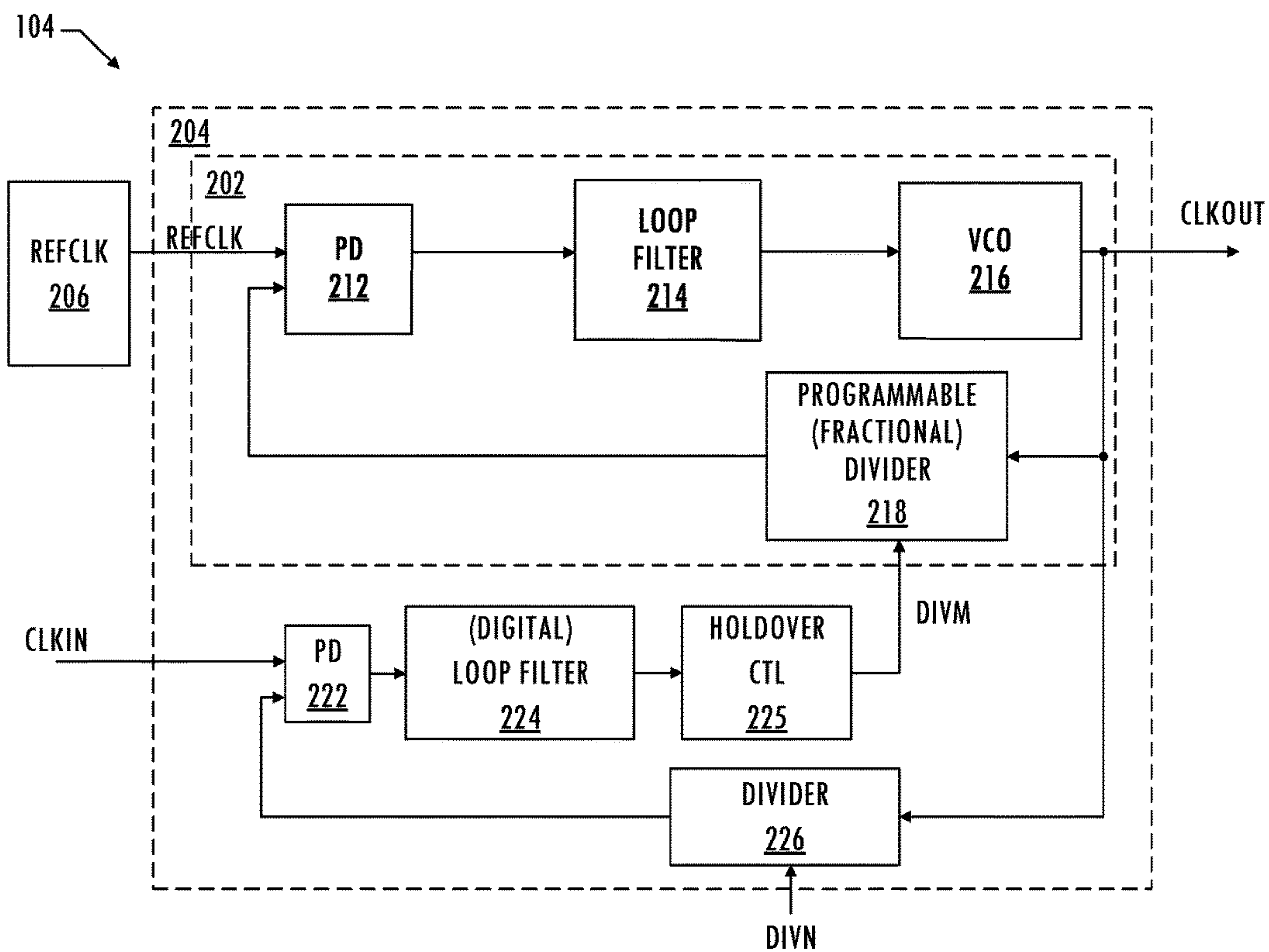
FIG. 2 (PRIOR ART)
