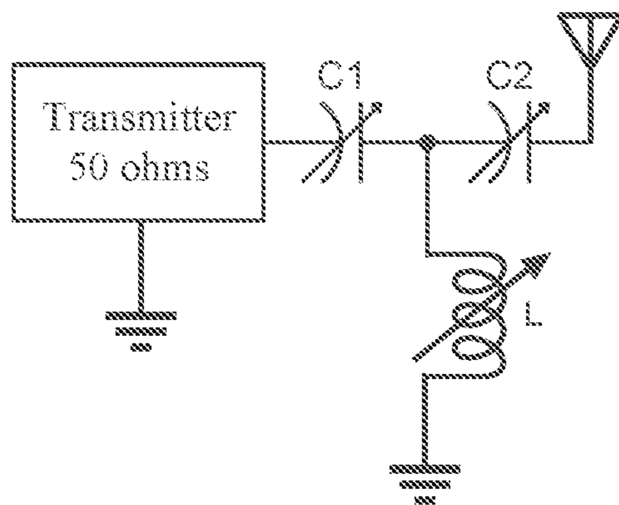
FIGURE 1 (Prior Art)
