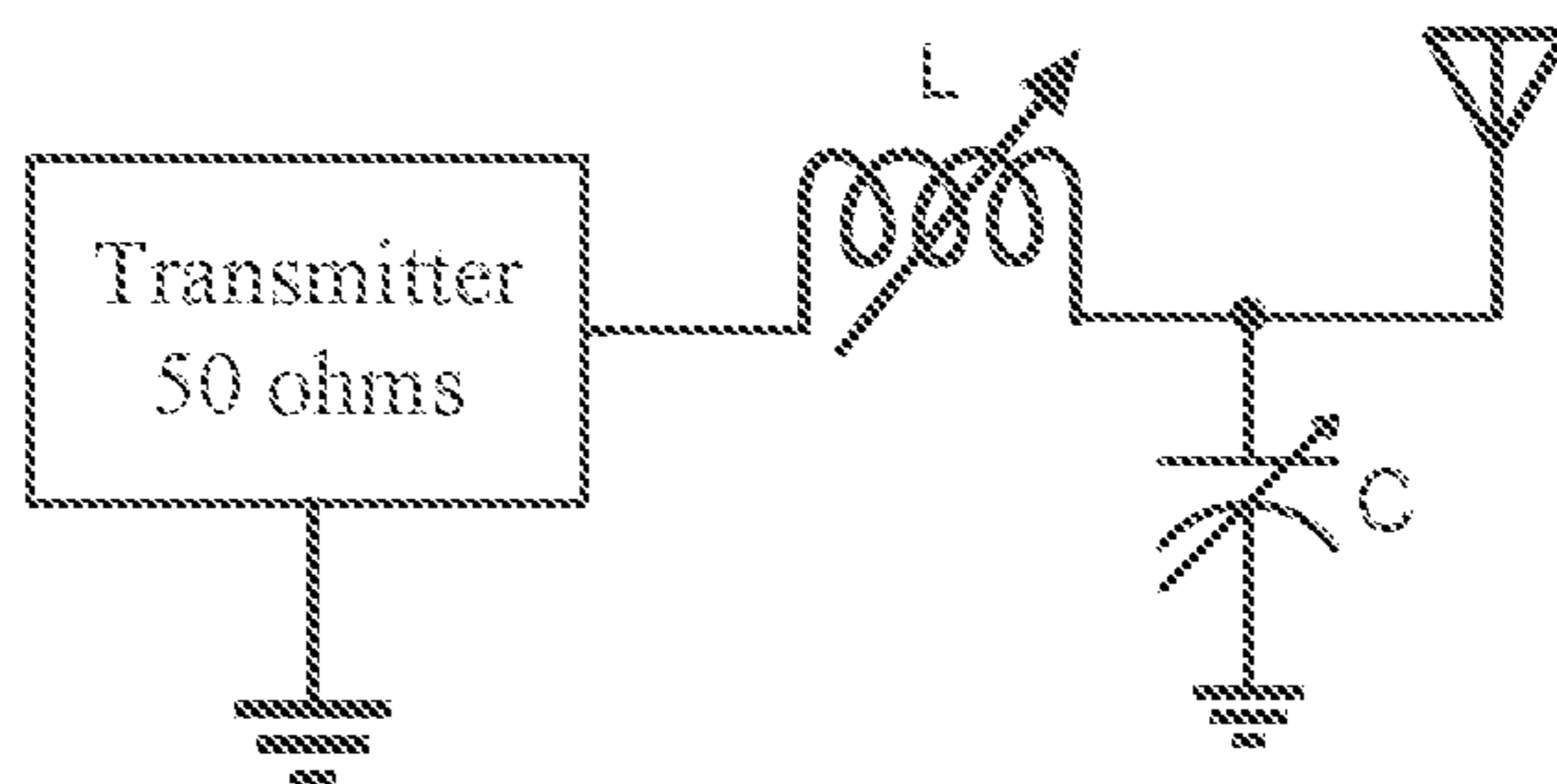
FIGURE 2 (Prior Art)
