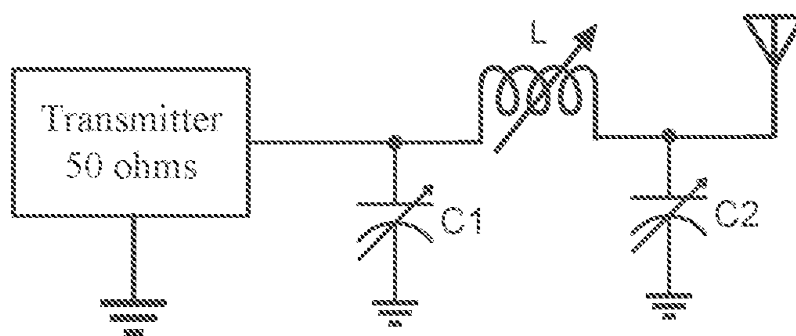
FIGURE 3 (Prior Art)
