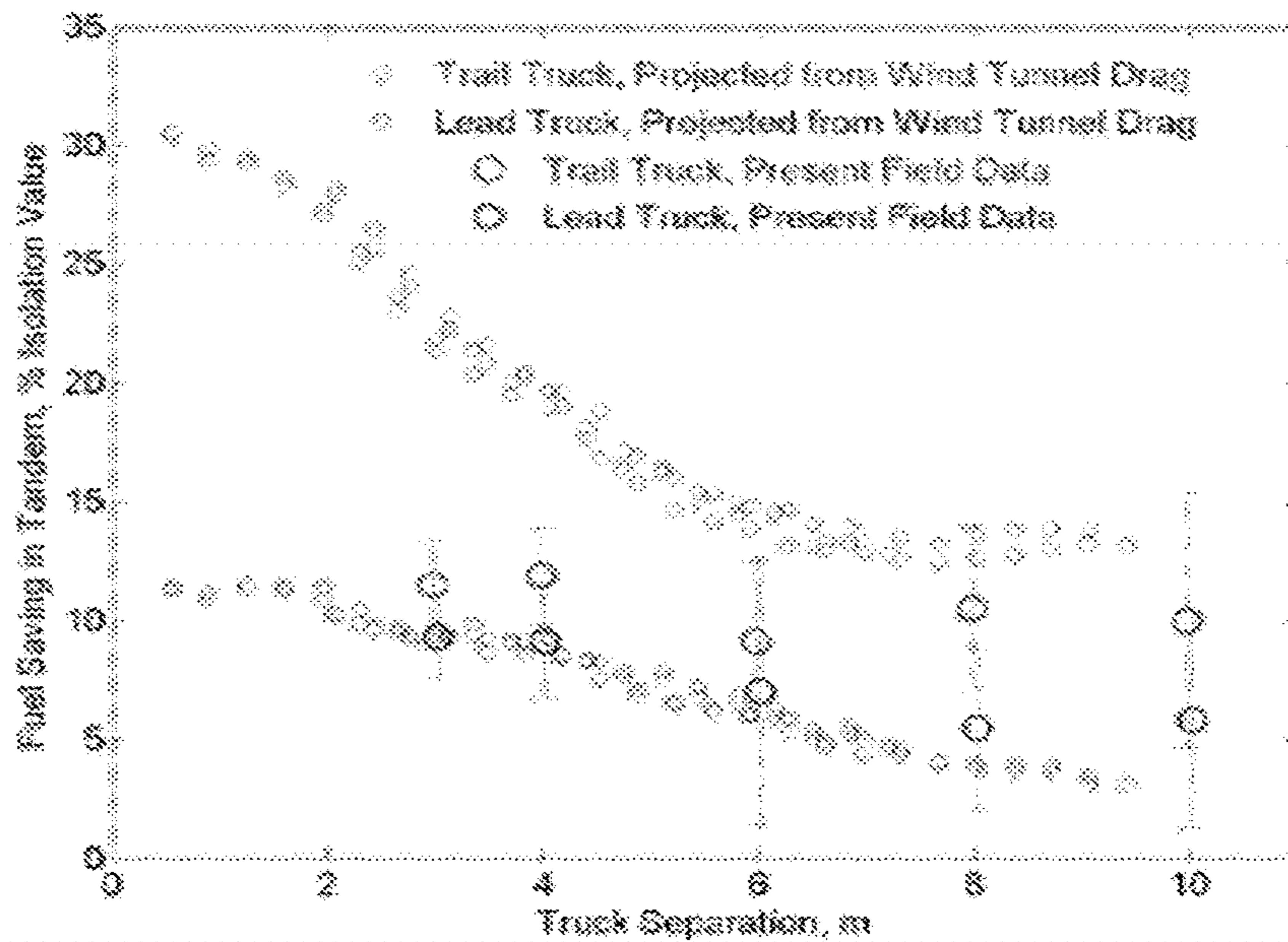
Figure 5: Fuel savings versus vehicle gap (Heavy Trucks)
