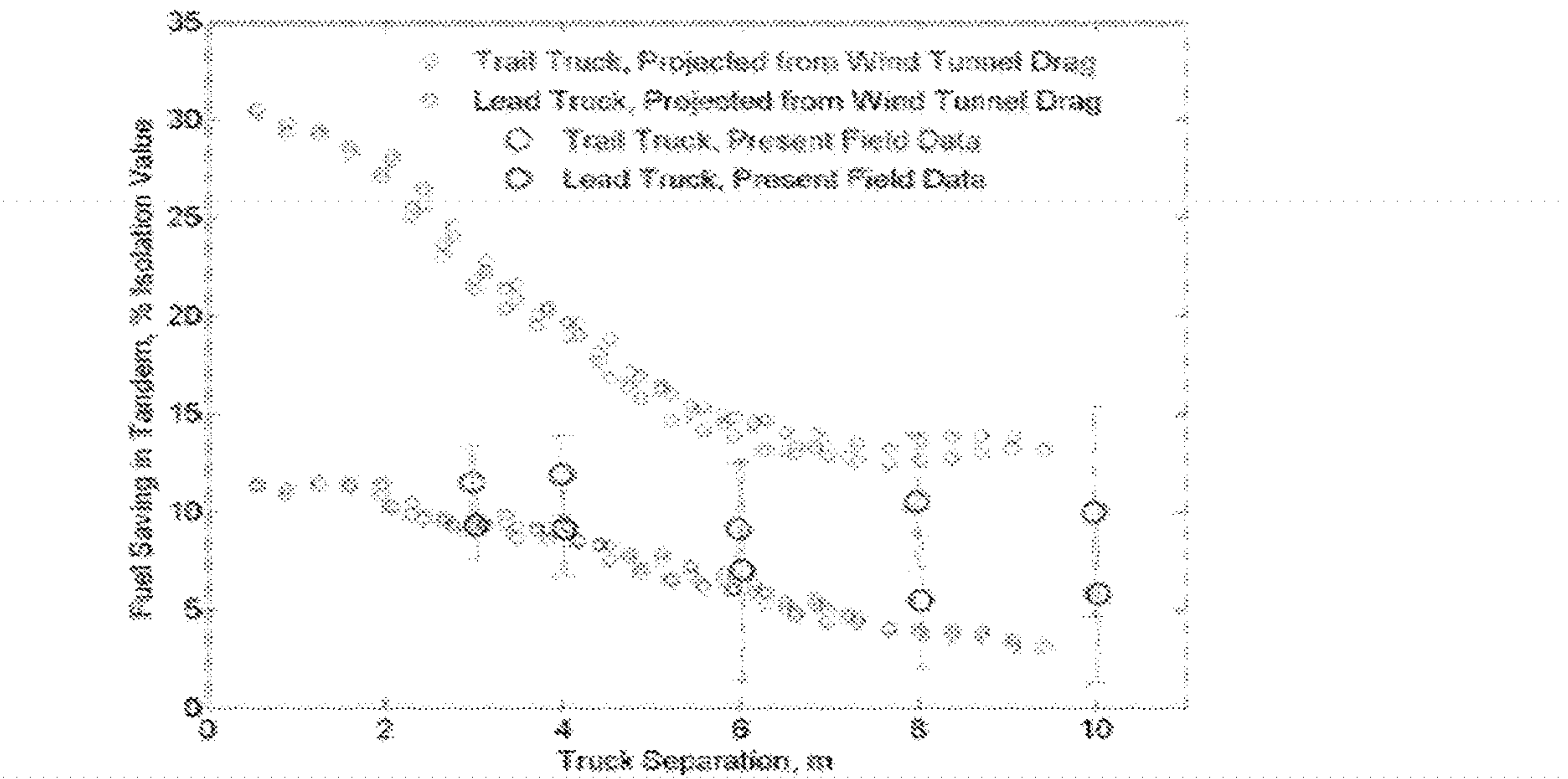
Figure 5: Fuel savings versus vehicle gap (Heavy Trucks)
