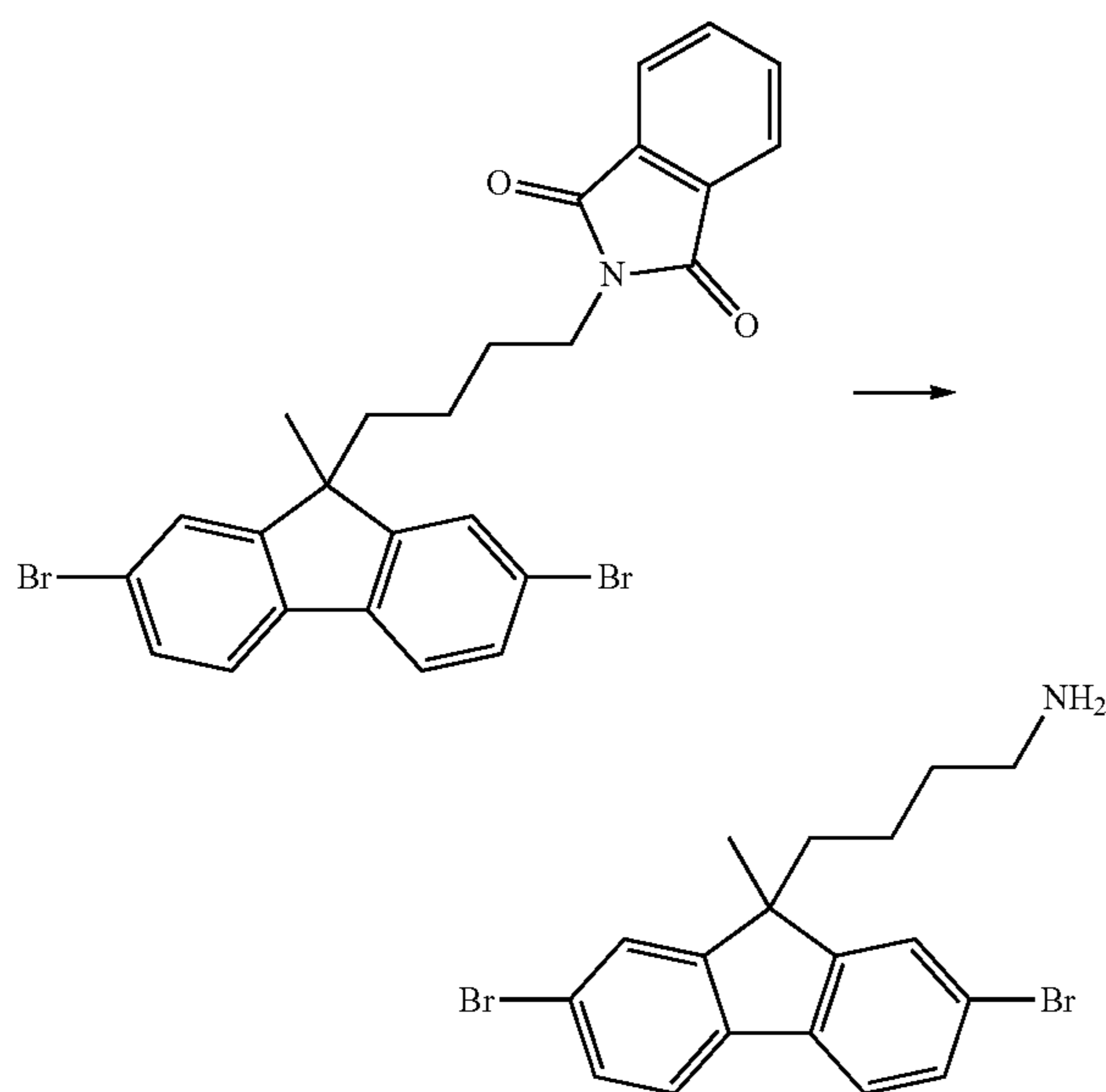
Step 3: 4-(2,7-dibromo-9-methyl-9H-fluoren-9-yl)butan-1-amine
