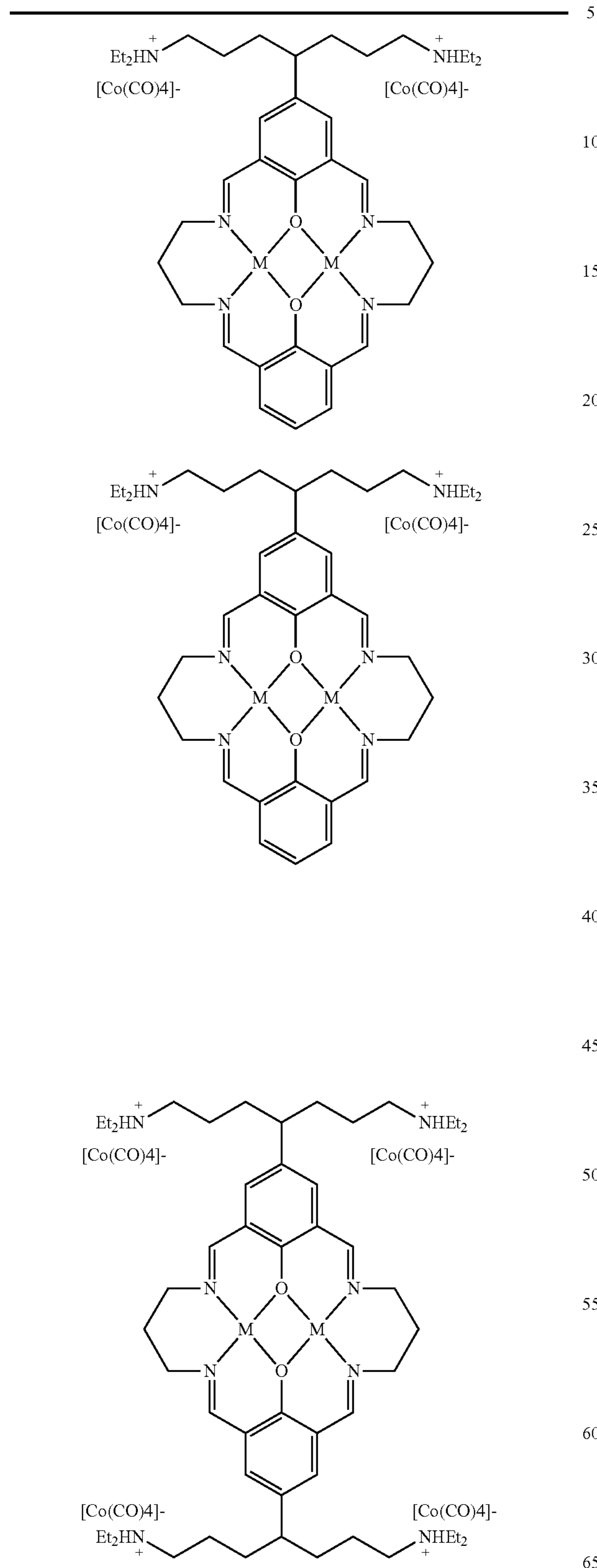
CATALYST TABLE 3
