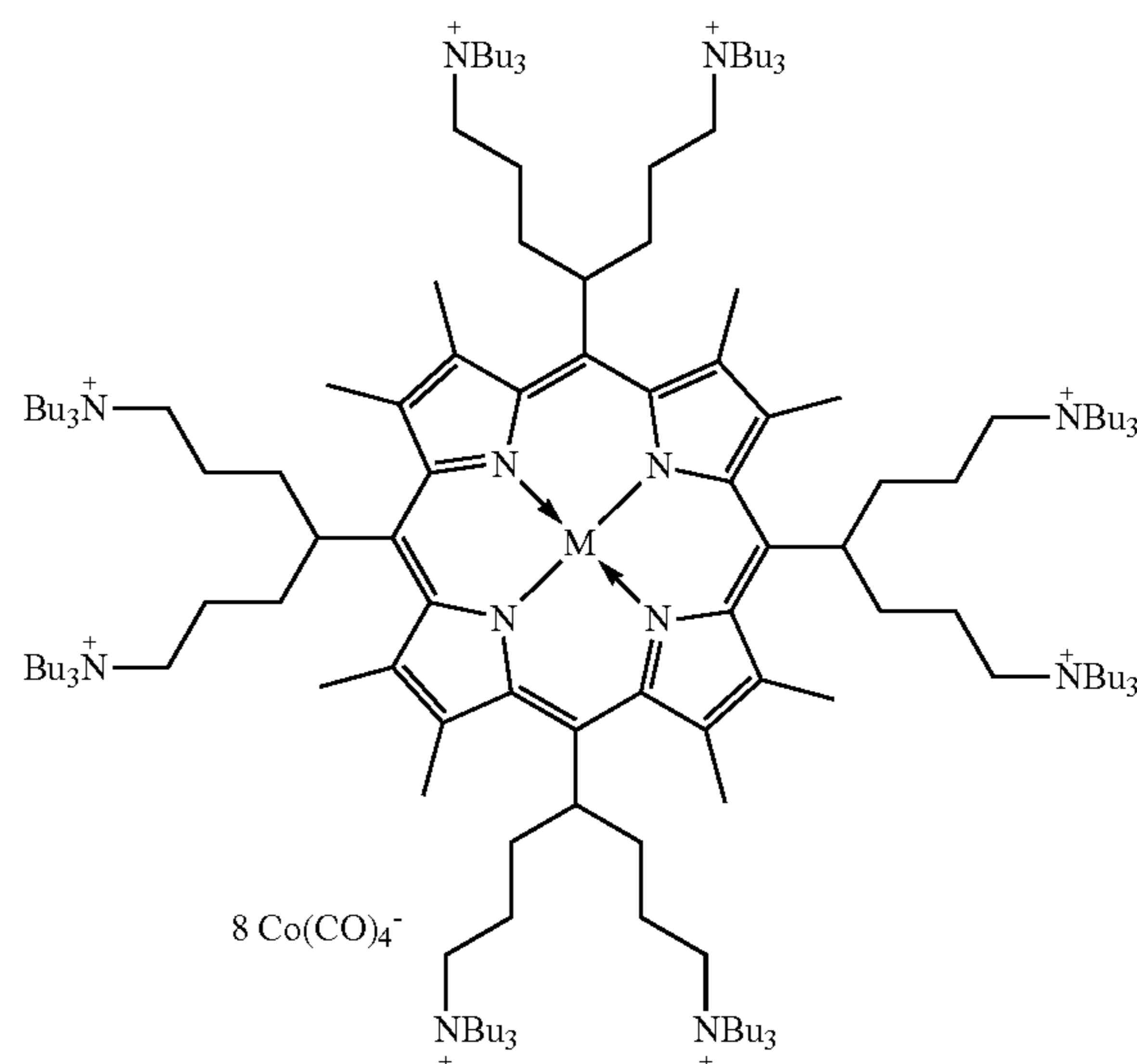
CATALYST TABLE 1
