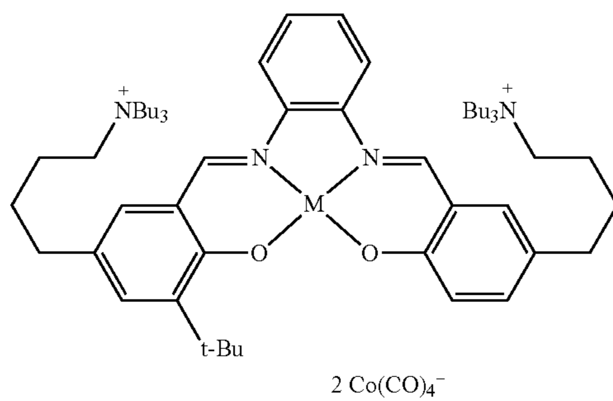
CATALYST TABLE 2
