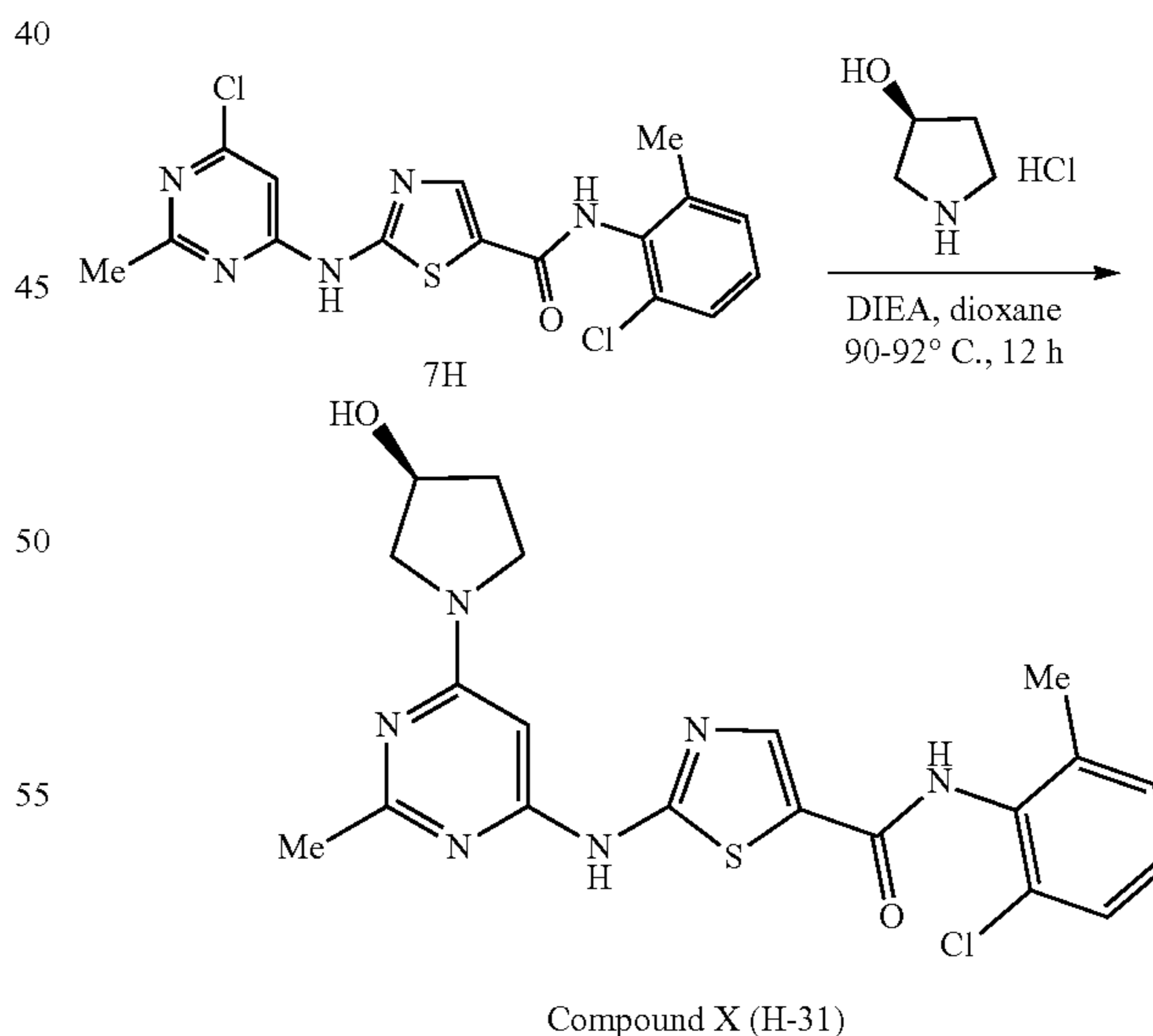
Scheme 10 Synthetic route for Compound X (H-31)
