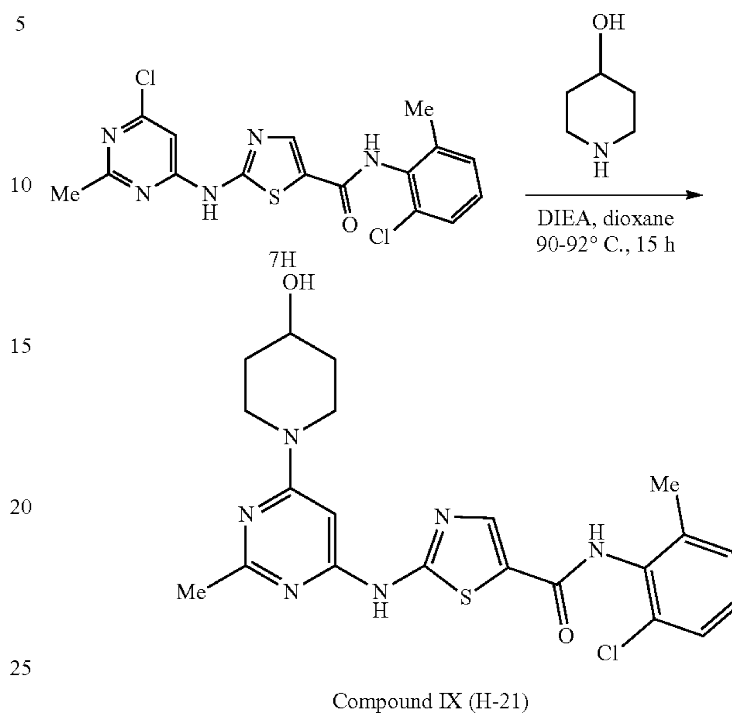
Scheme 9 Synthetic route for Compound IX
