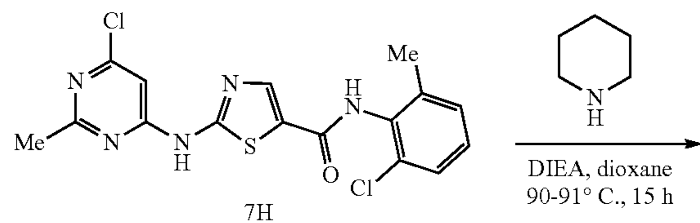
Scheme 8 Synthetic route for Compound VIII
