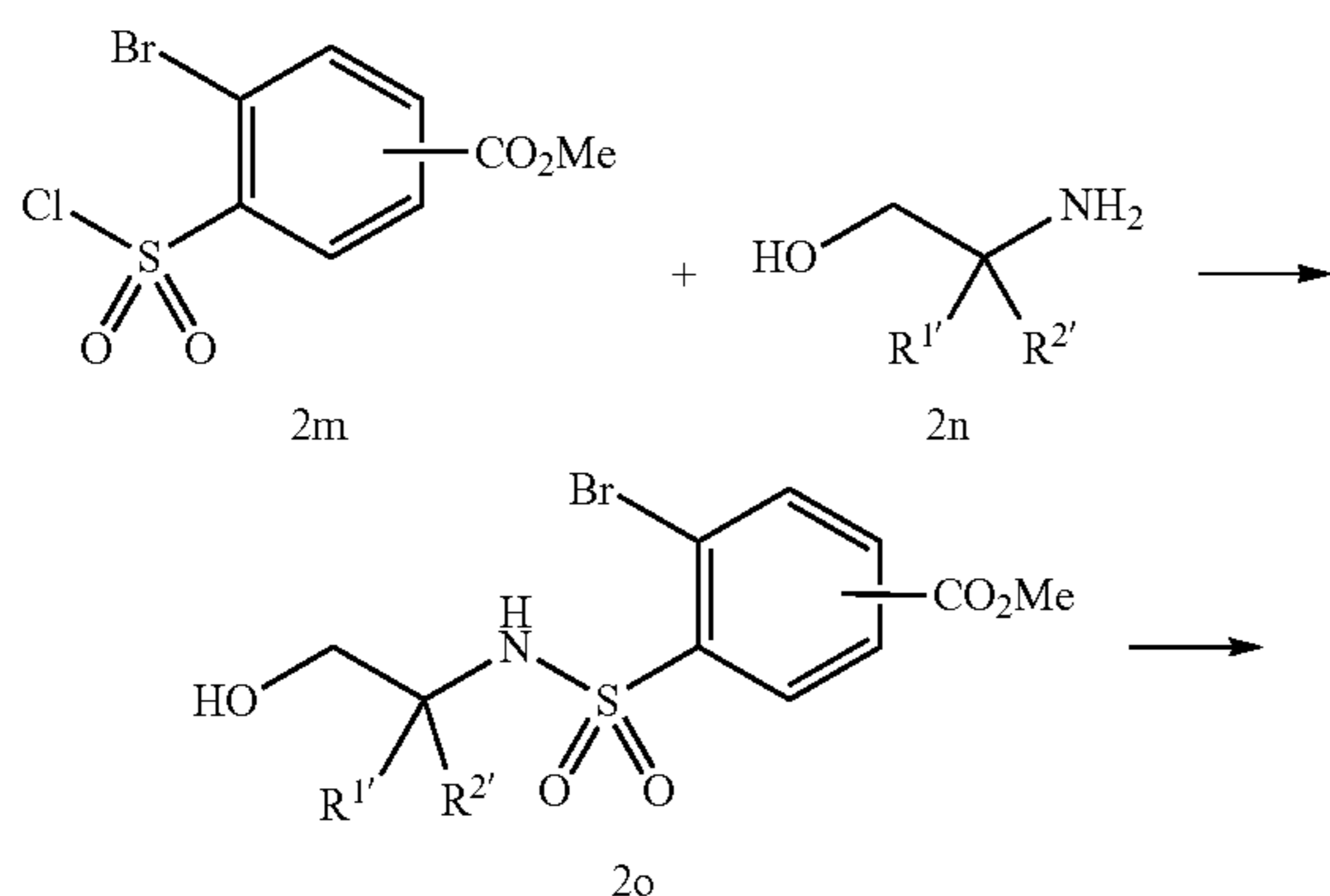
Scheme 3. General synthesis of sulfonamides described in the disclosure.
