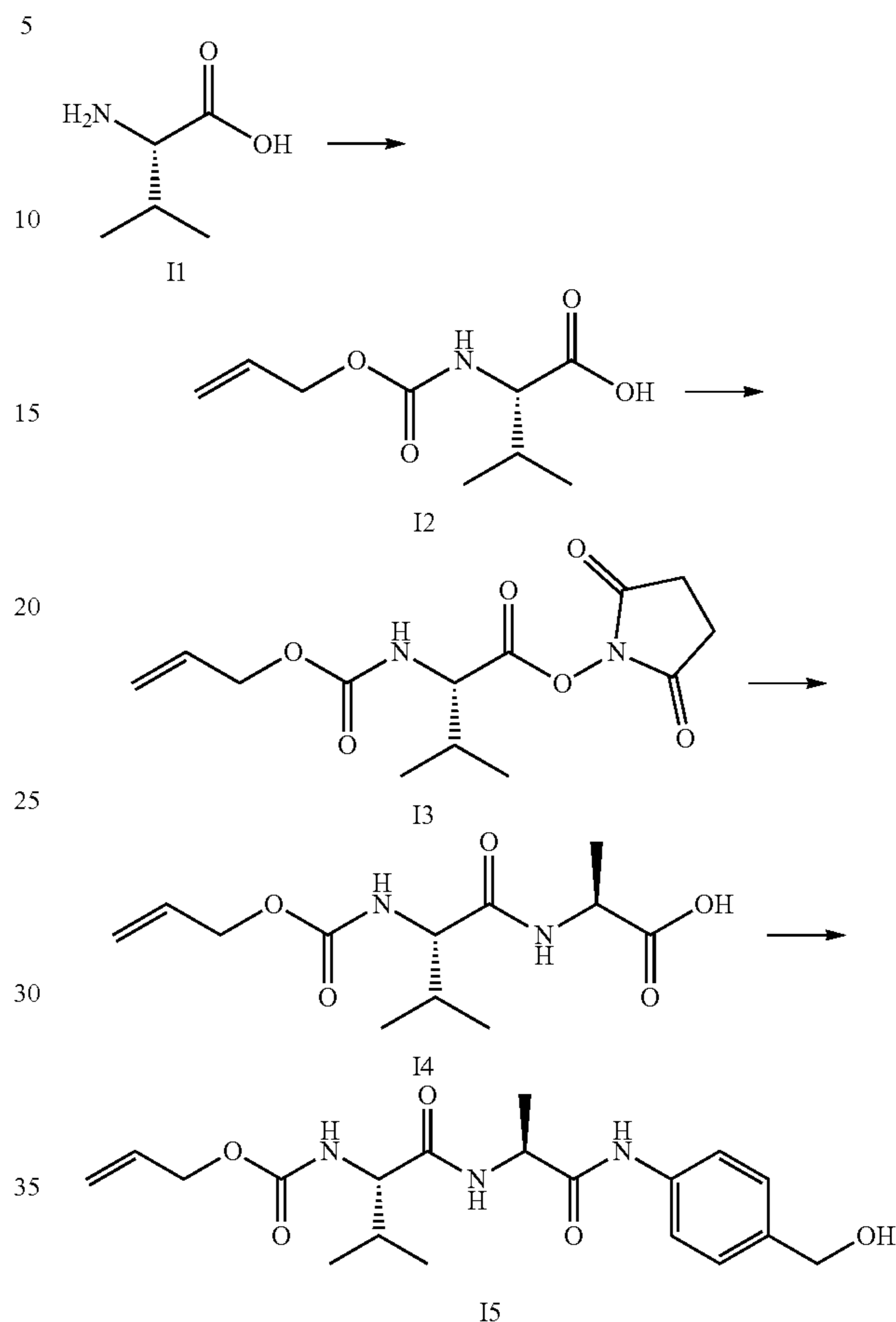
(a-i) (S)-2-(allyloxycarbonylamino)-3-methylbutanoic acid (12)
