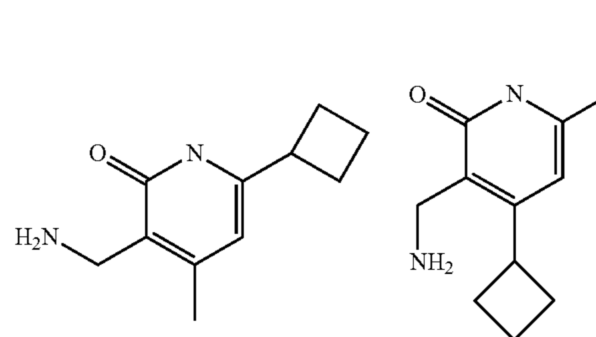
13d) 3-(aminomethyl)-6-cyclobutyl-4-methyl-2(1H)-pyridinone and 3-(aminomethyl)-4-cyclobutyl-6-methyl-2(1H)-pyridinone
