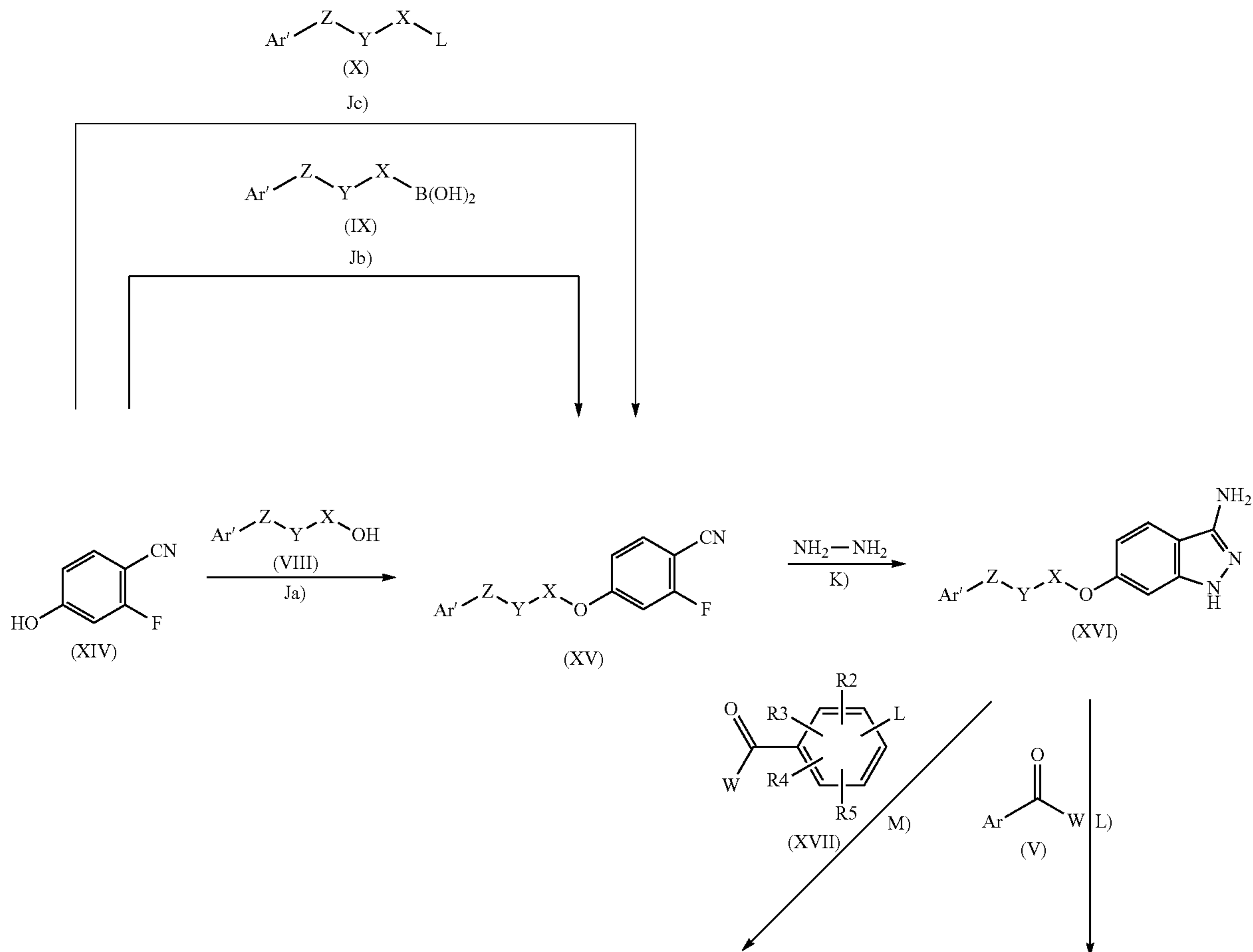
Scheme 2
