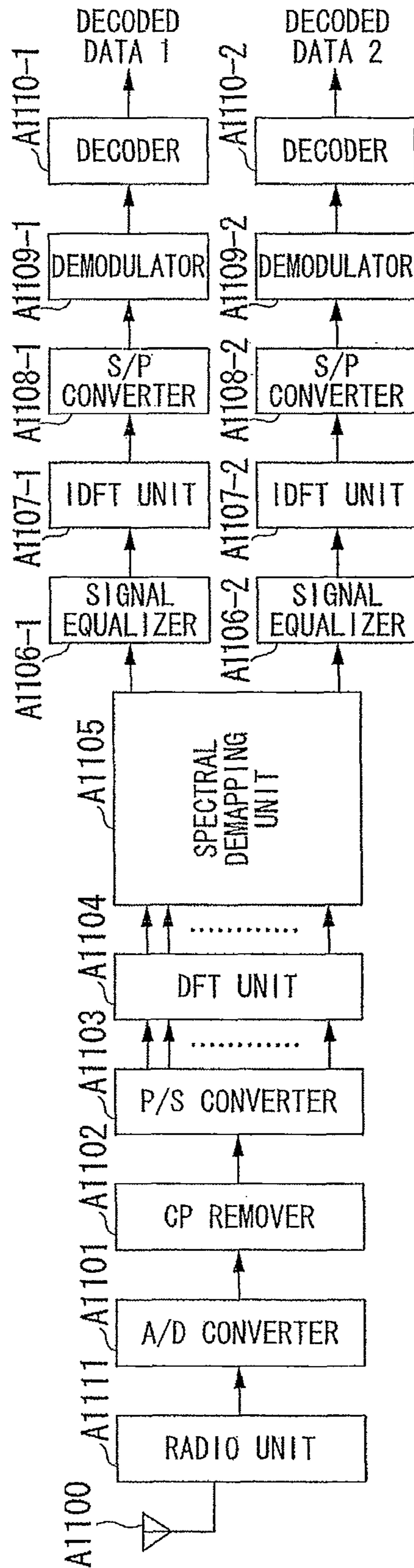
RECEPTION BLOCK DIAGRAM
