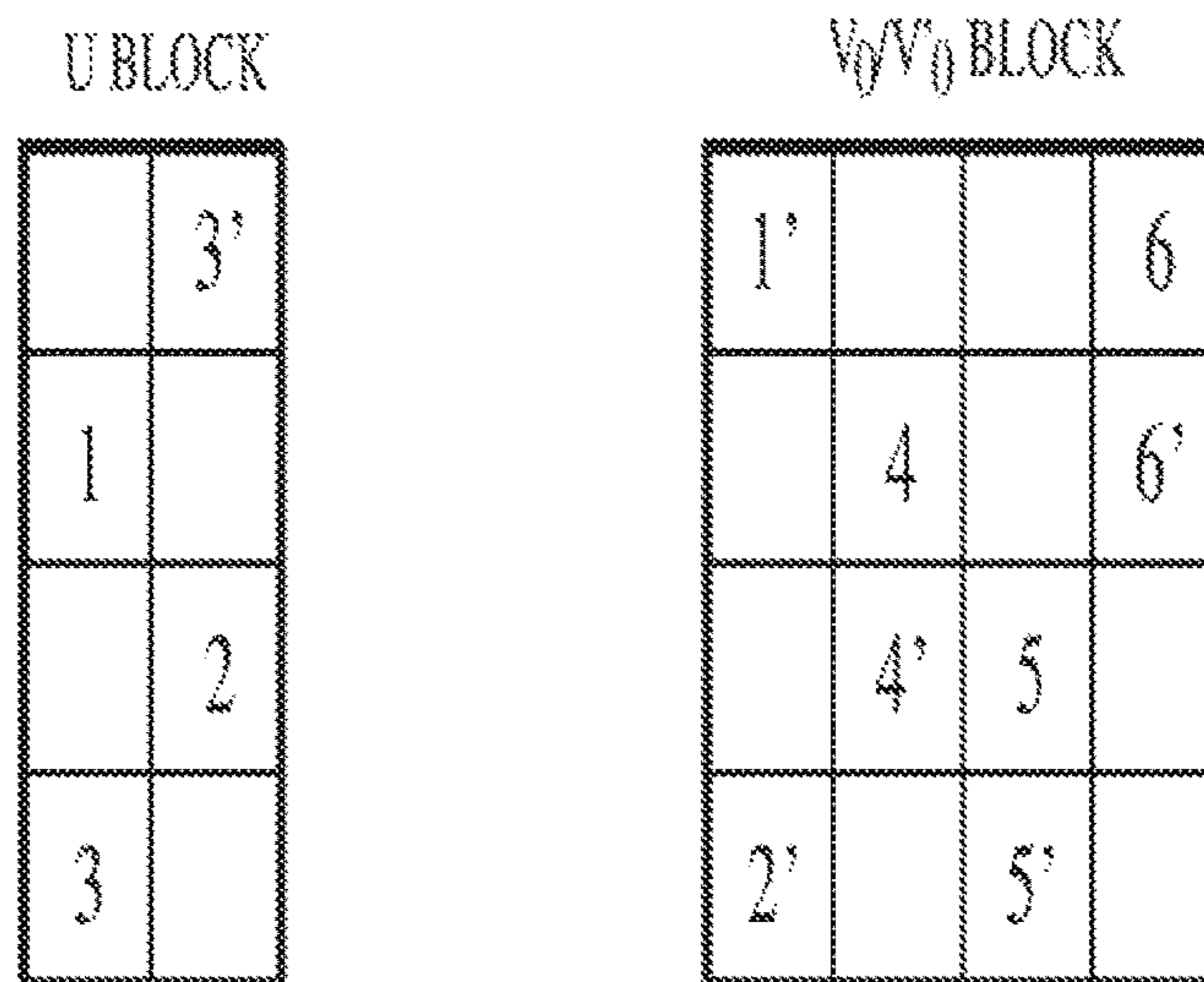
FIG. 7B: BLOCK SWAP PATTERN FOR 16-QAM
