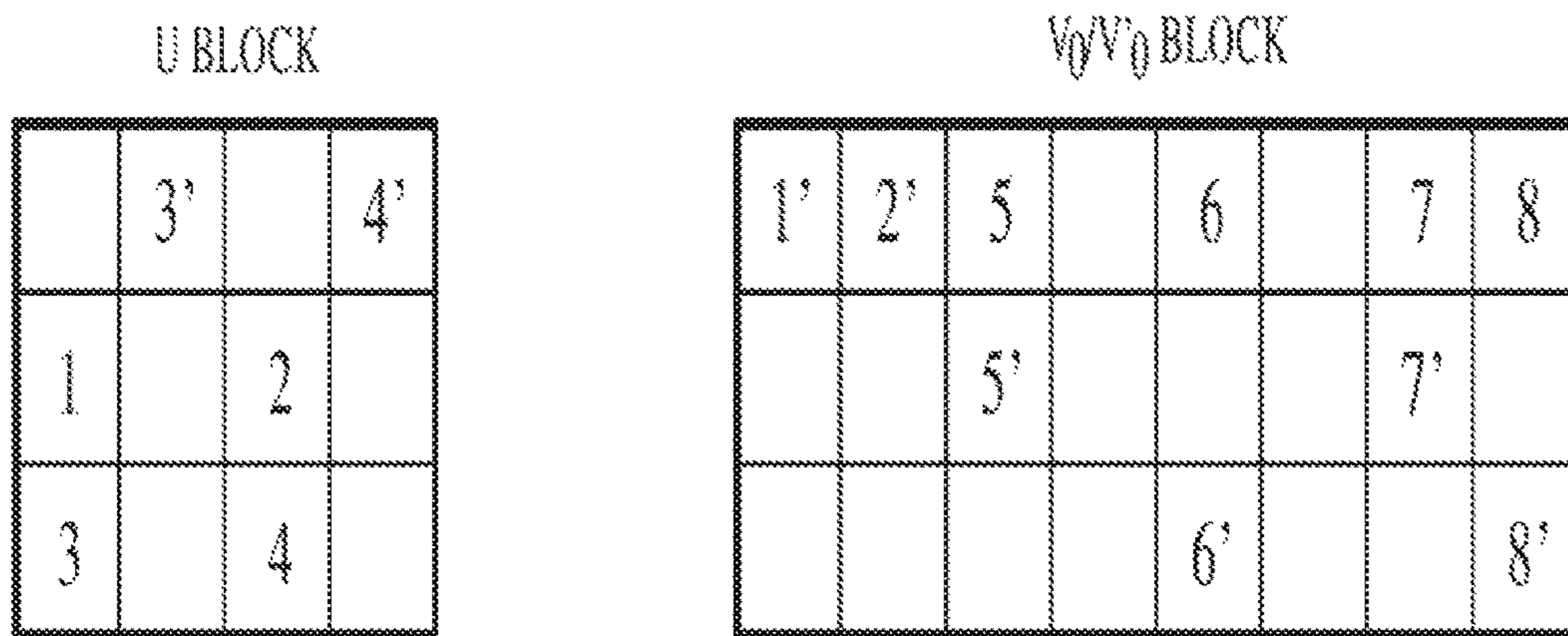
FIG. 7A: BLOCK SWAP PATTERN FOR 8-PSK
