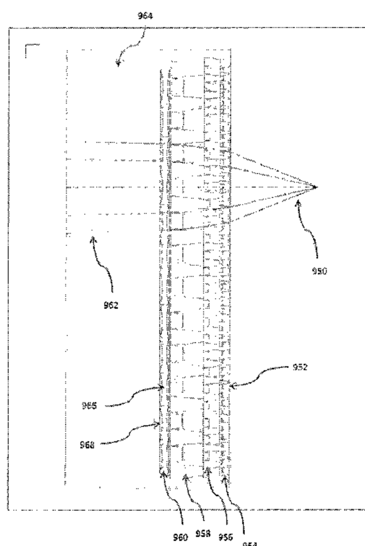
Alternative design of Supercladding layer
