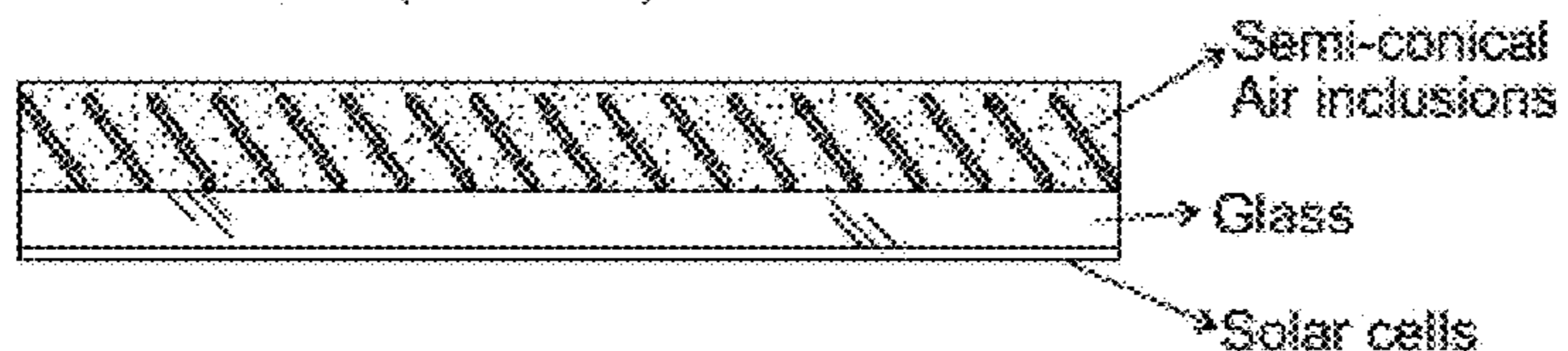
Longitudinal Section (side view)
