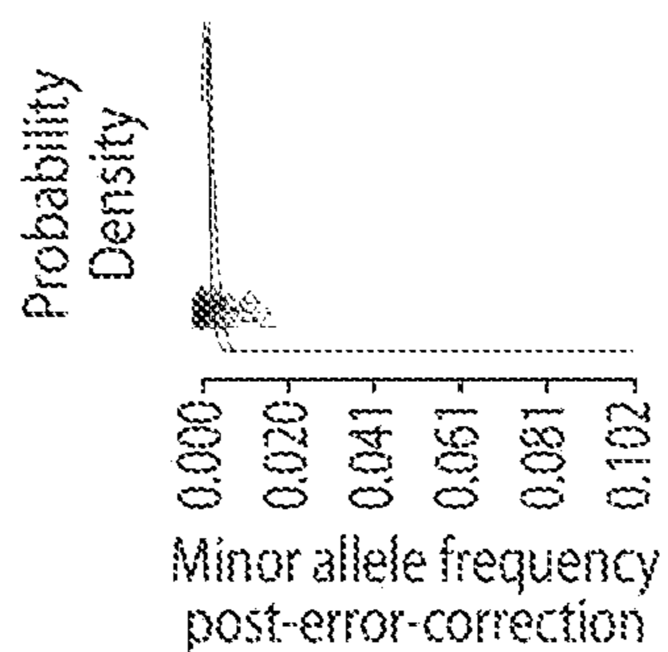
GT-informed fitting Binomials
