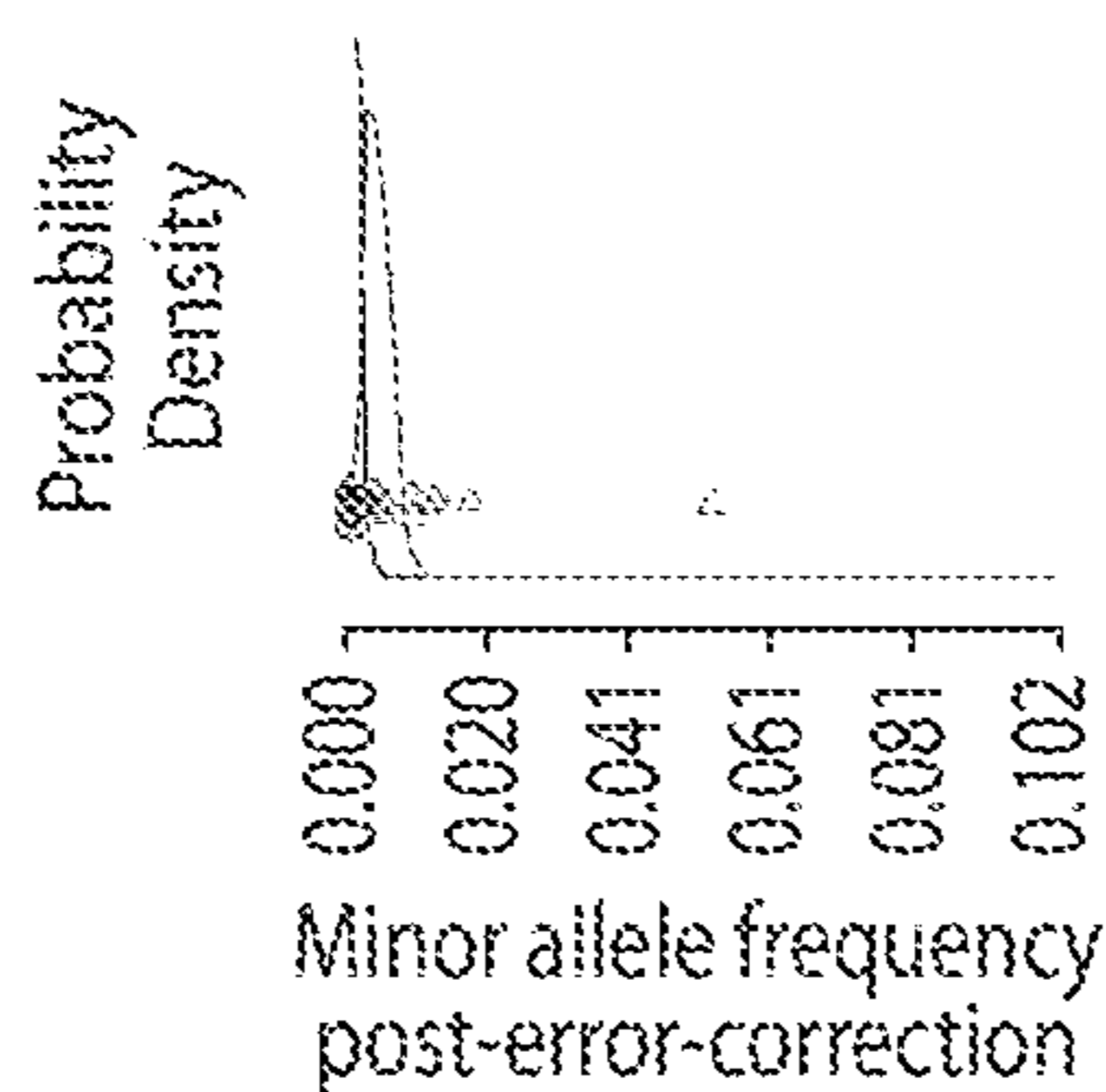
GT-informed fitting Binomials
