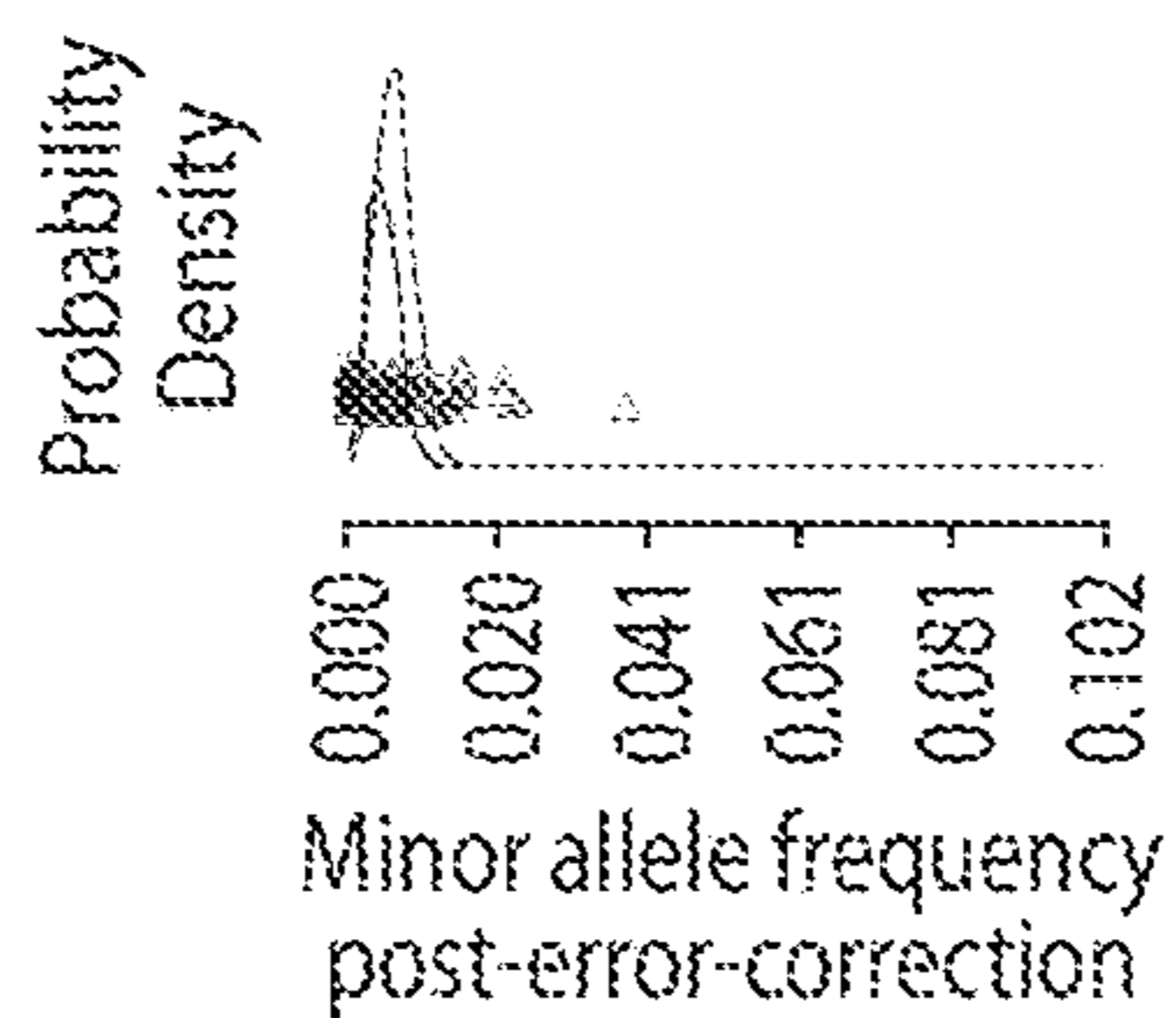
GT-informed fitting Binomials
