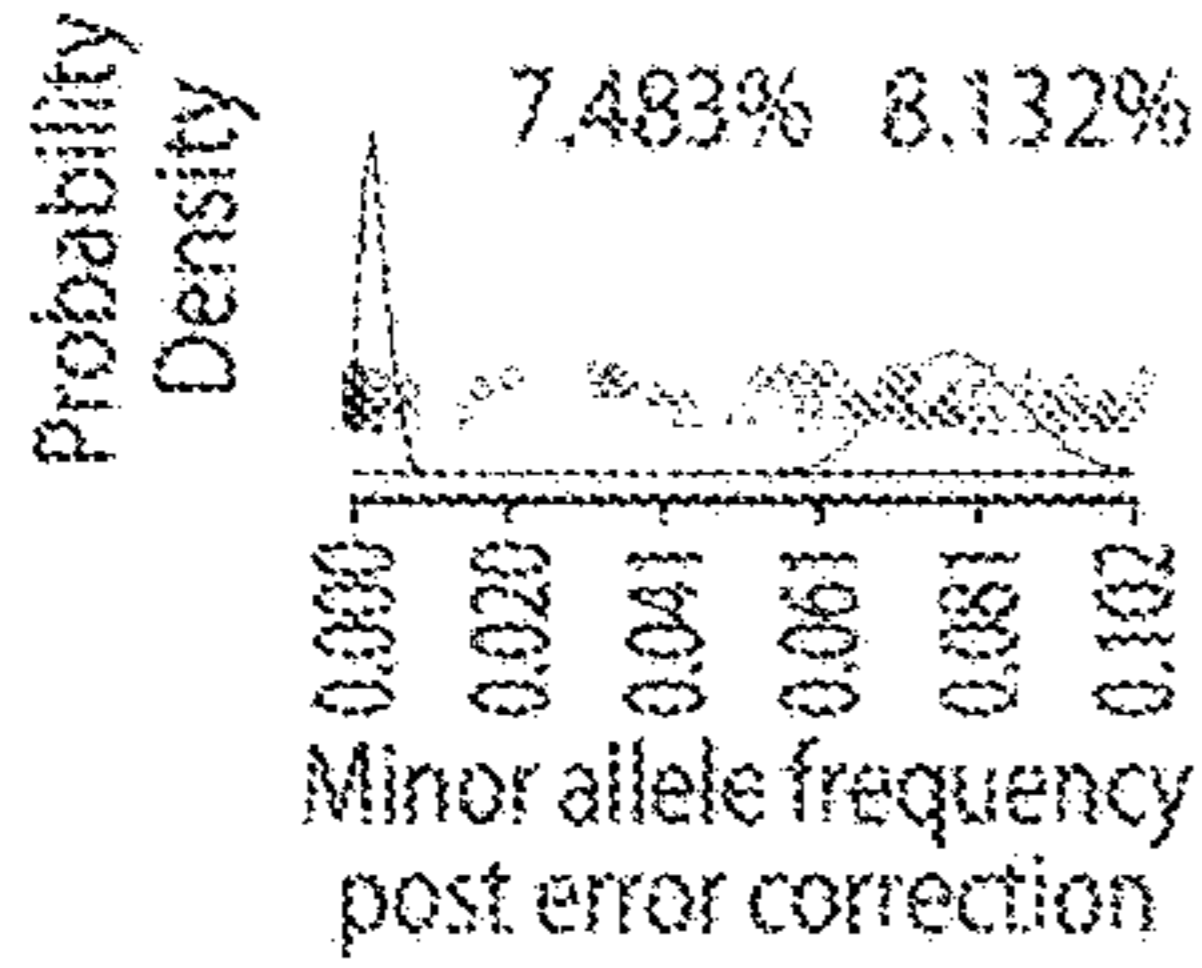
GT-informed fitting Binomials
