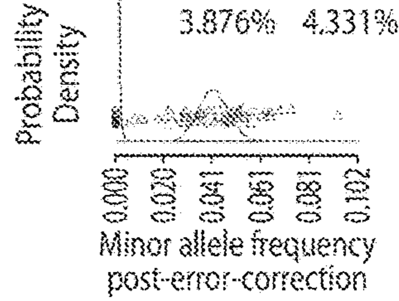
GT-informed fitting Binomials
