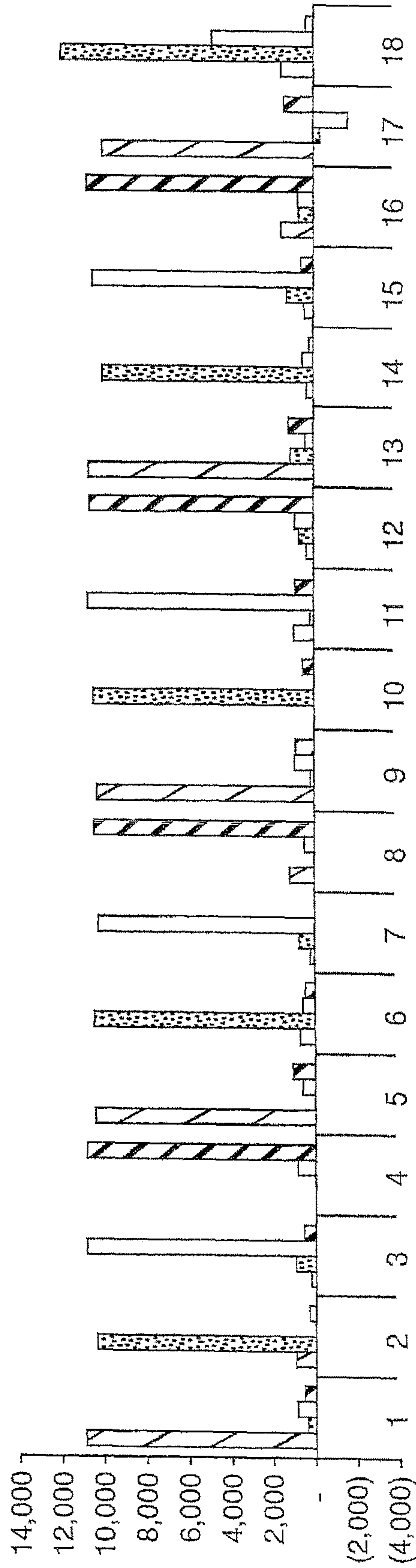
DE-PHASED DATA FOR 18 BASE READ
