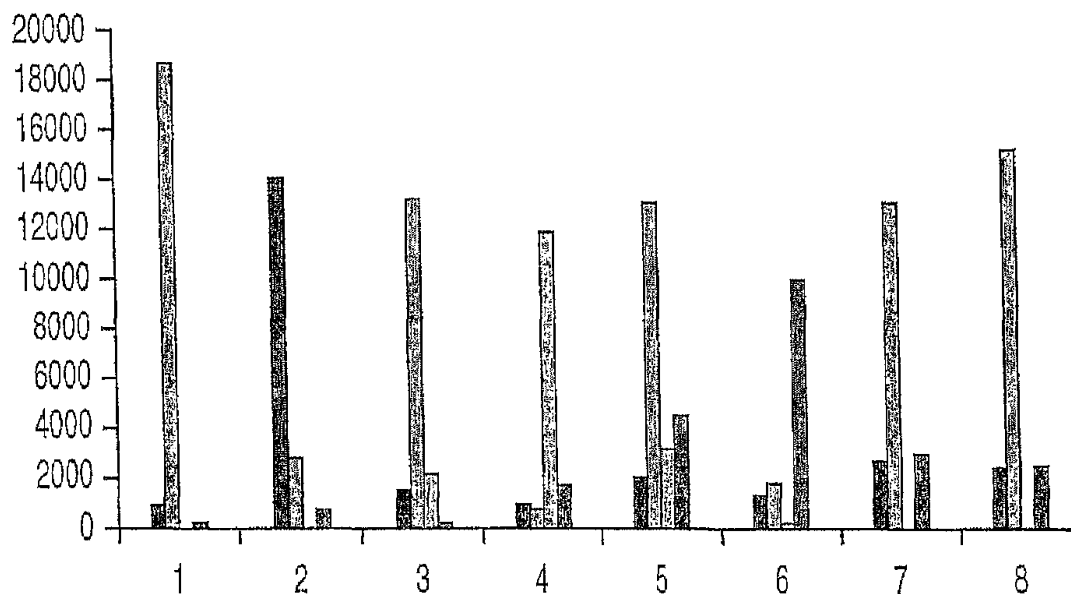
DATA WITH COLOR CROSSTALK REMOVED
