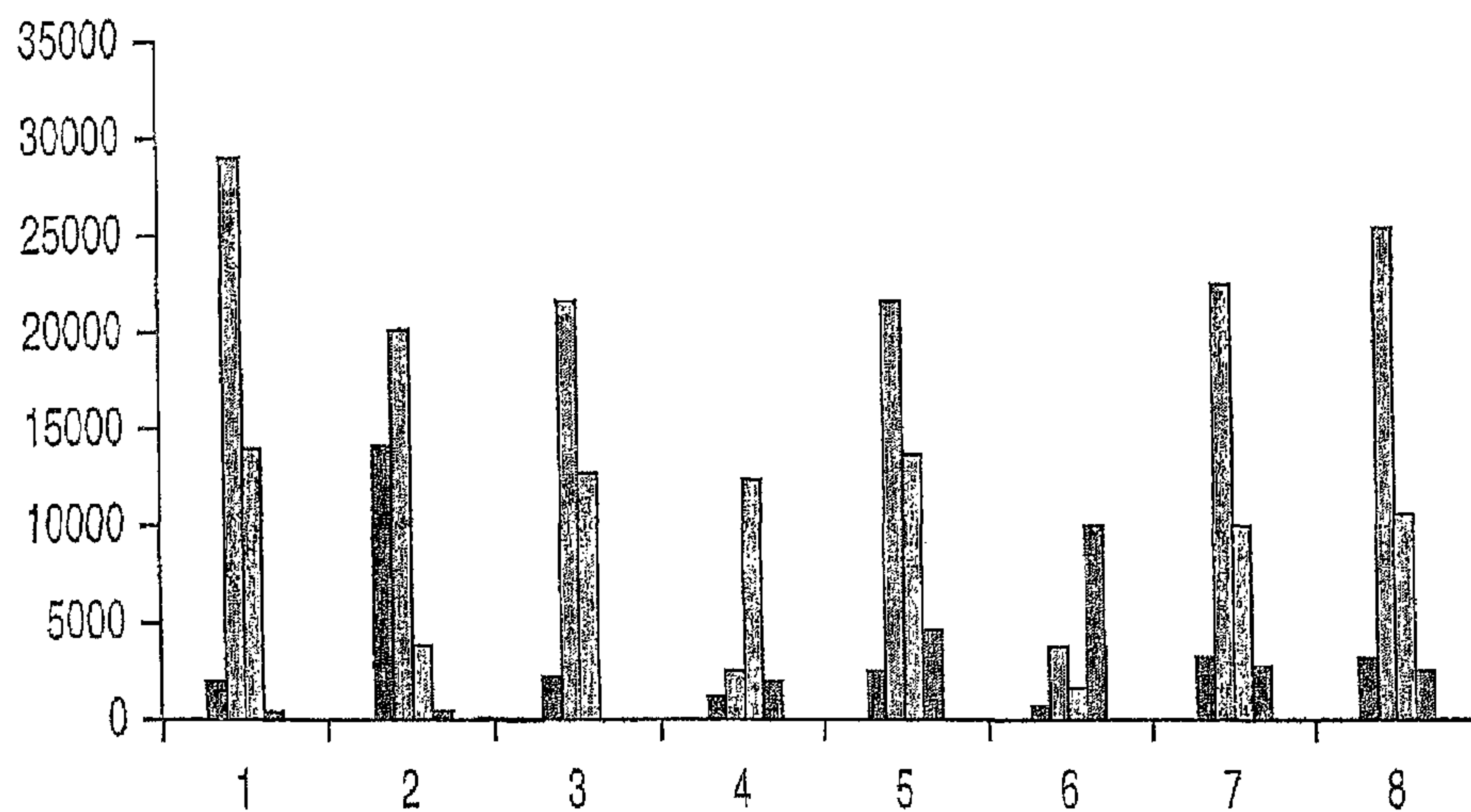
RAW DATA WITH COLOR CROSSTALK
