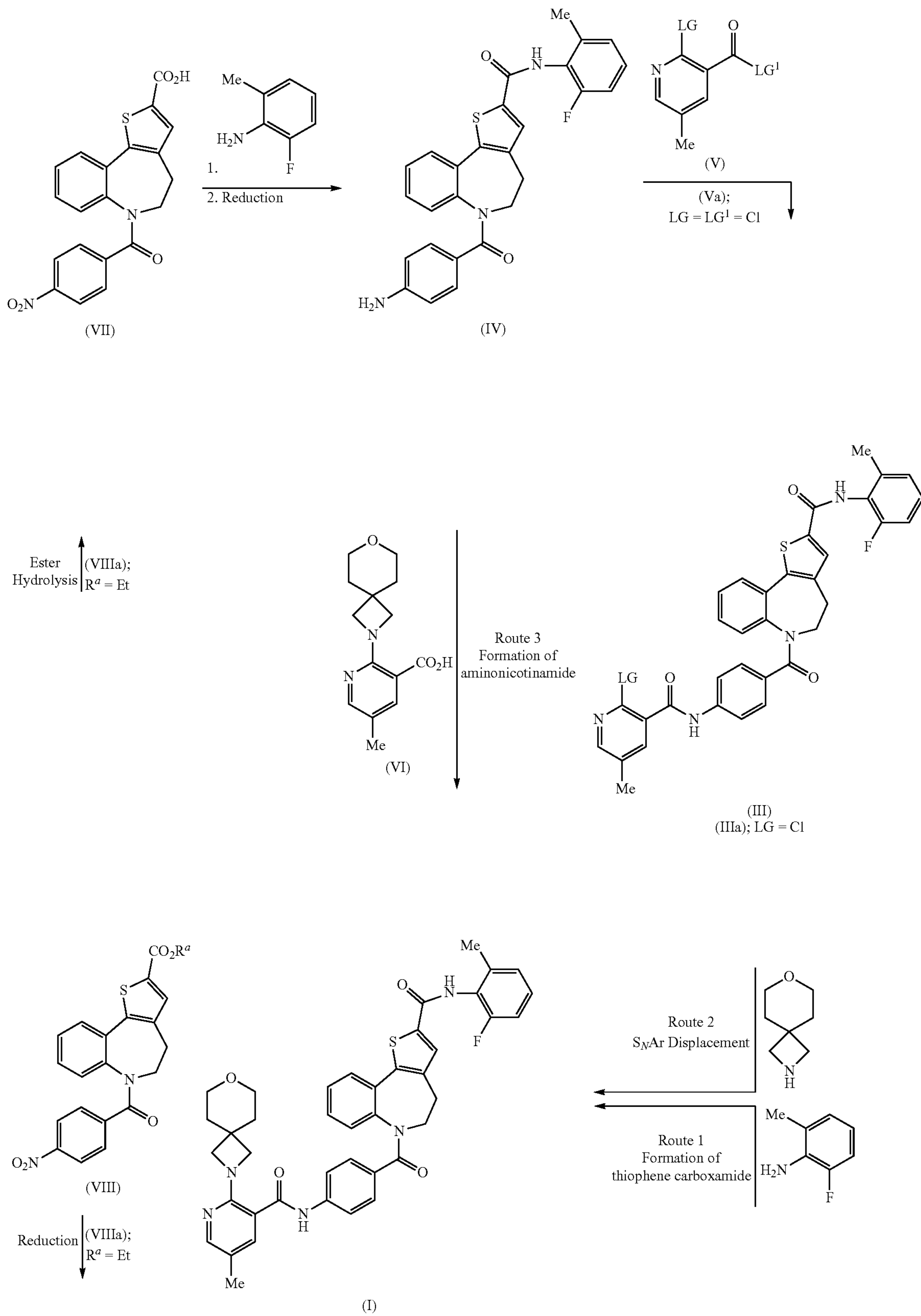
Scheme 1: Synthetic routes used for the preparation of Compound (I).
