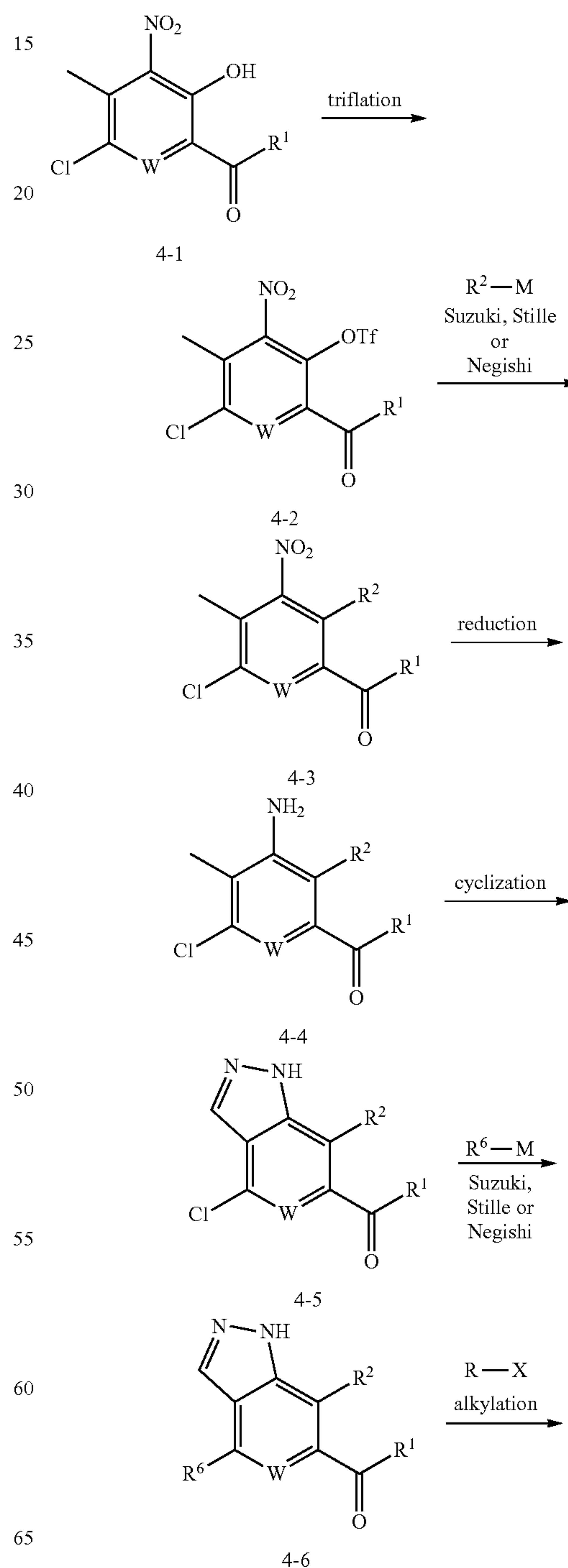
Scheme 4.
