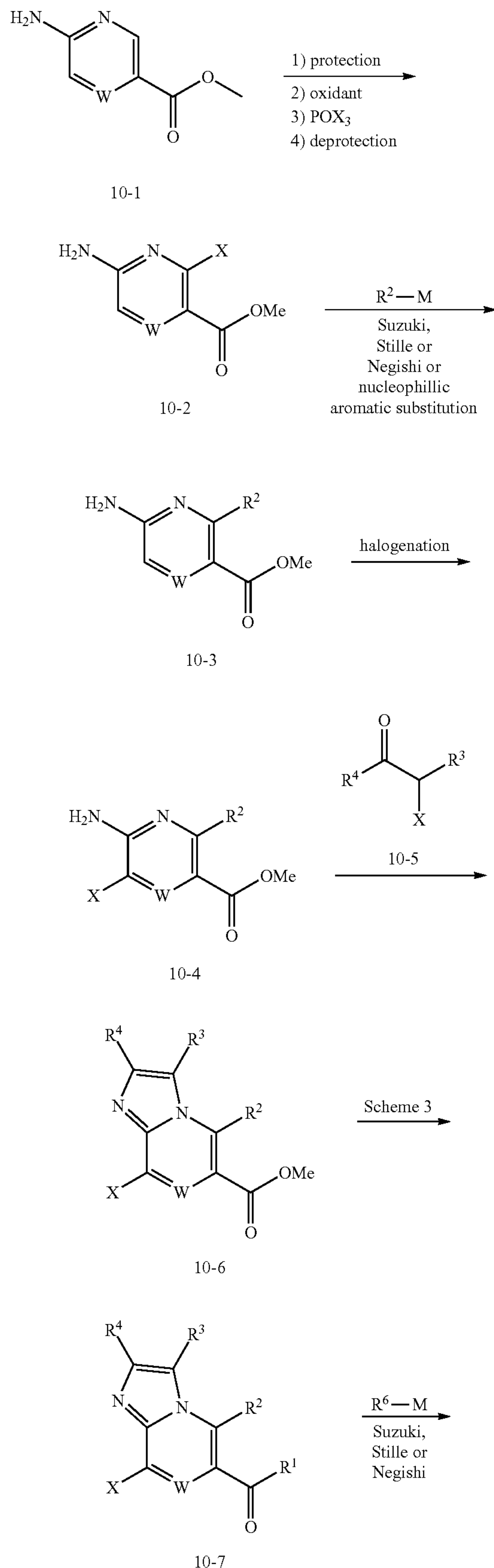
Scheme 10.
