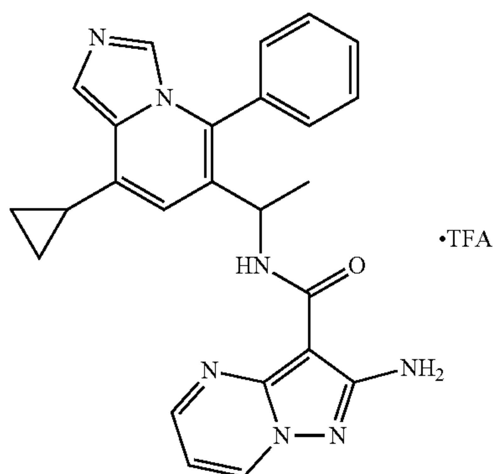
Step 1. 1-(8-Cyclopropyl-5-phenylimidazo[1,5-a]pyridin-6-yl)ethanone
