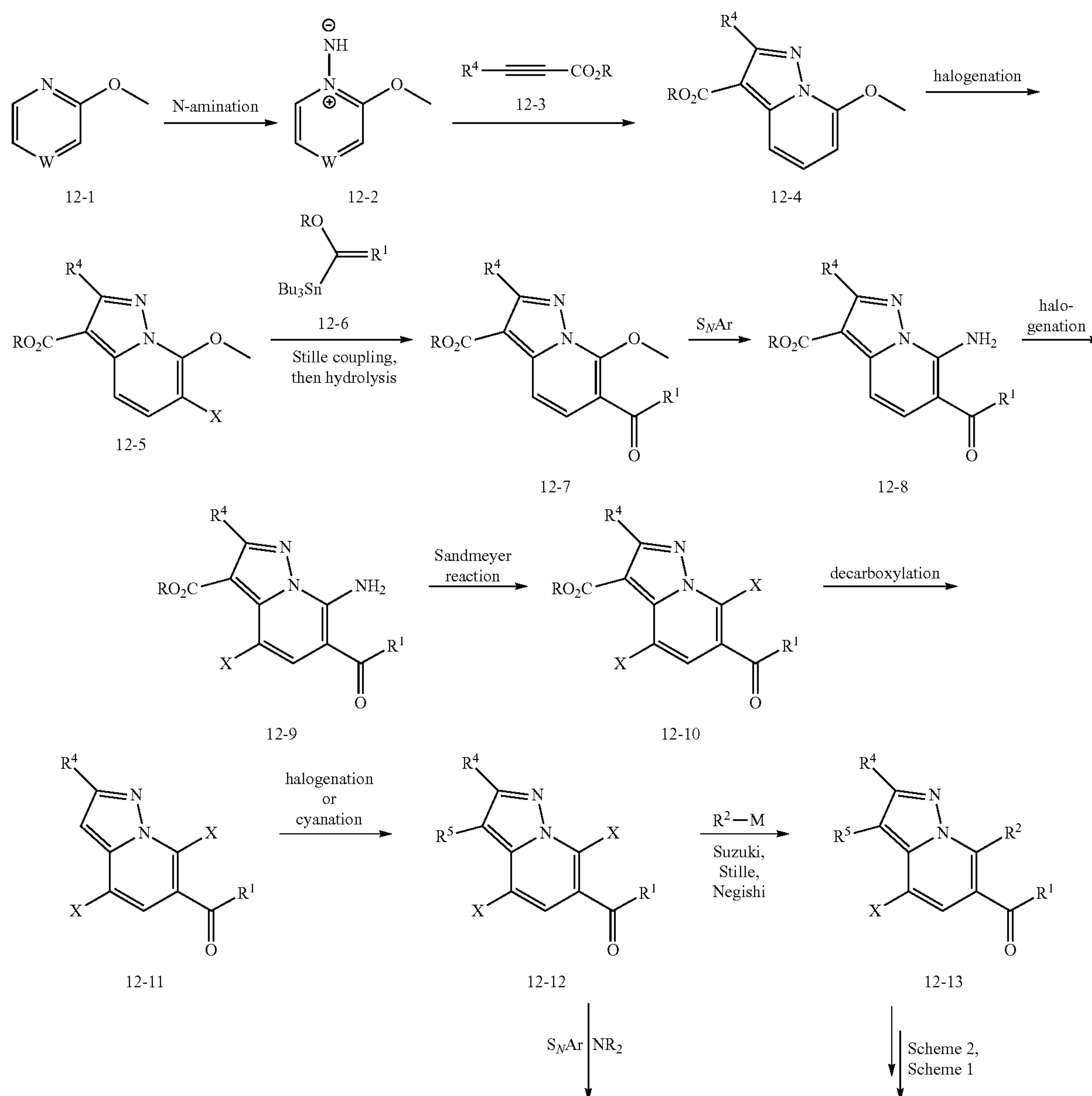
Scheme 12
