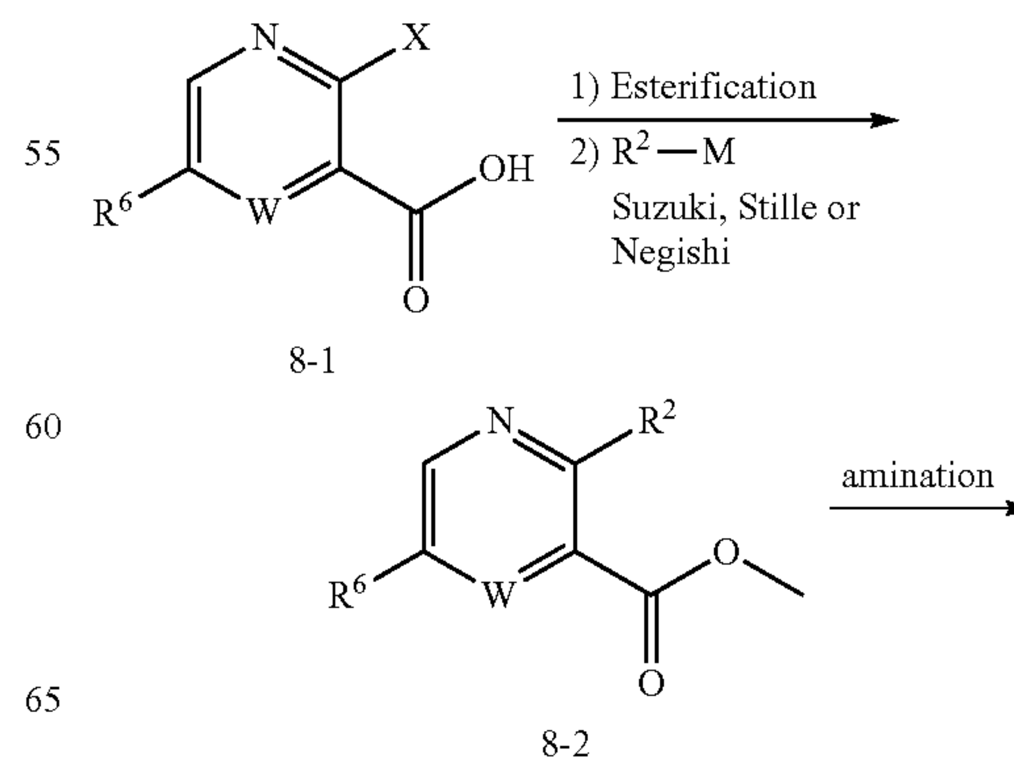
Scheme 8.
