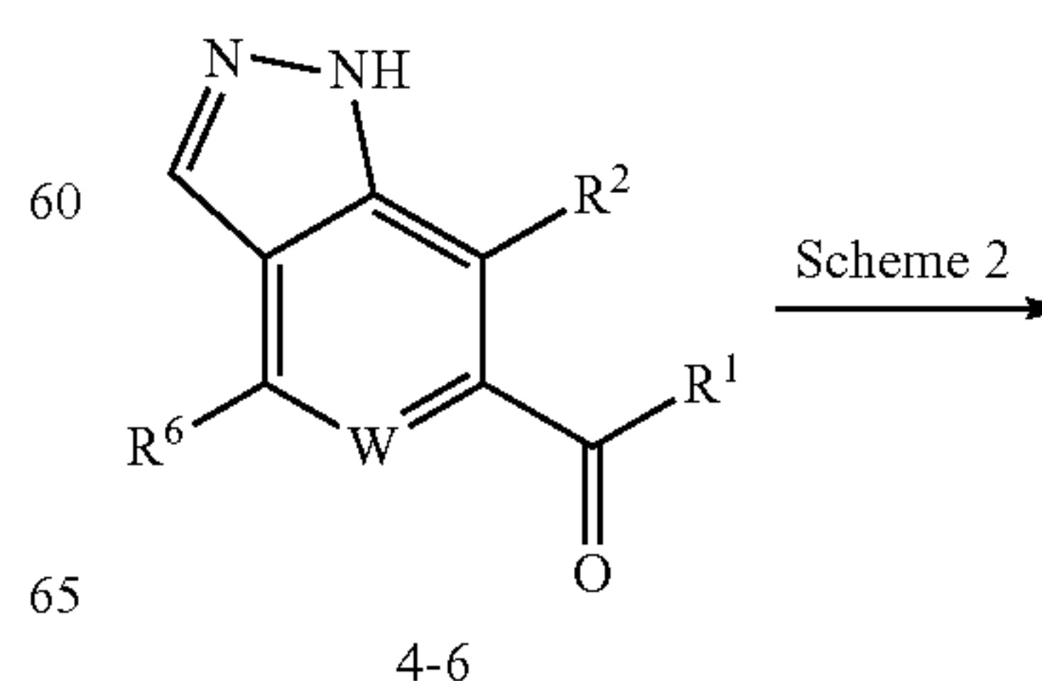
Scheme 6.
