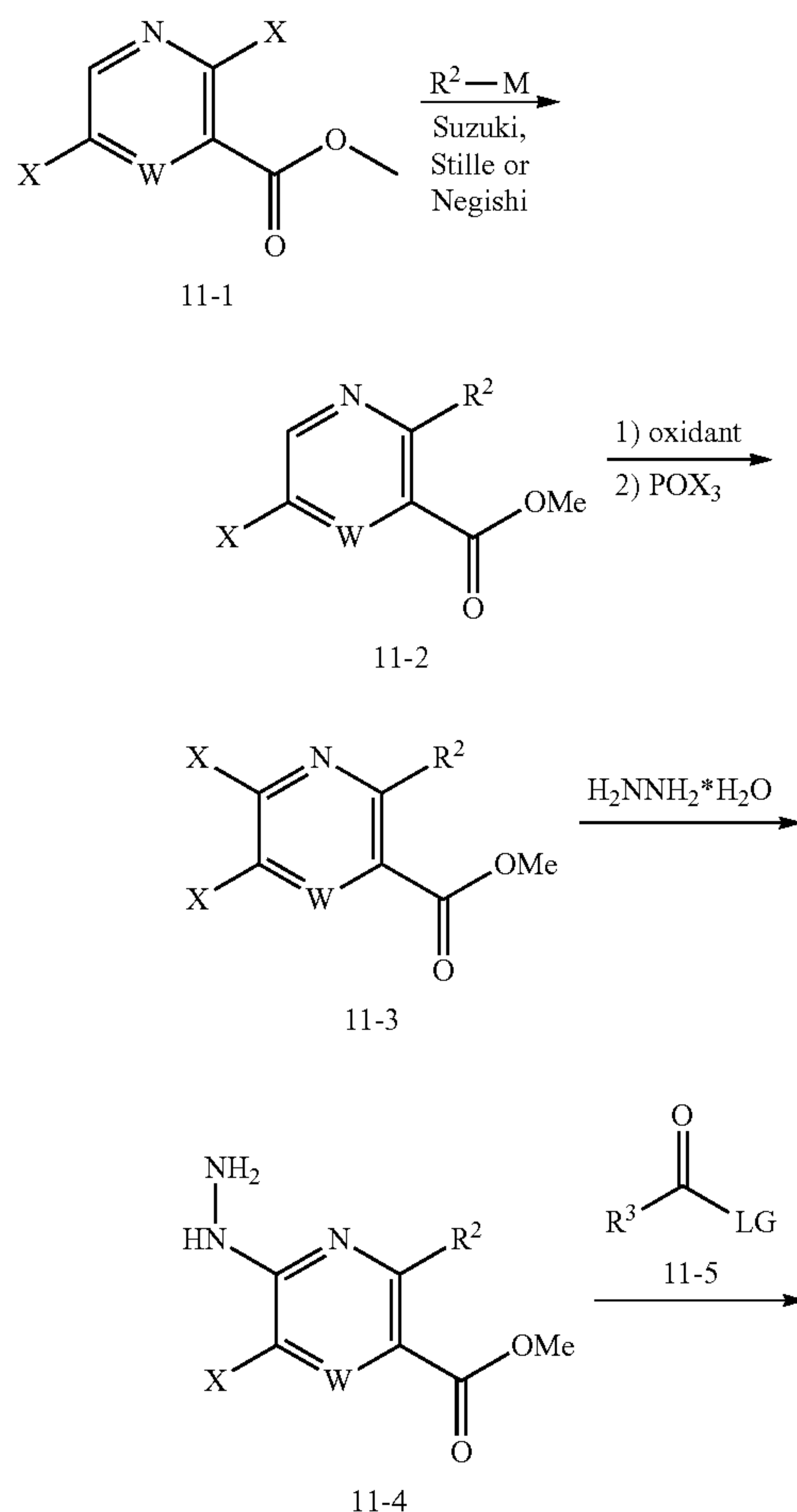
Scheme 11.
