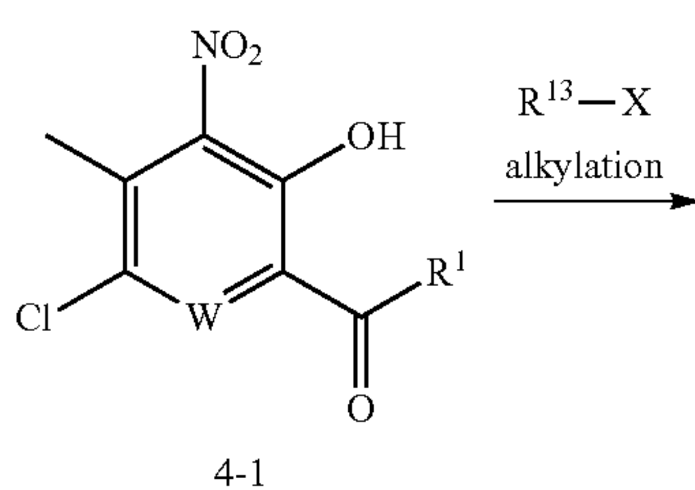
Scheme 5.
