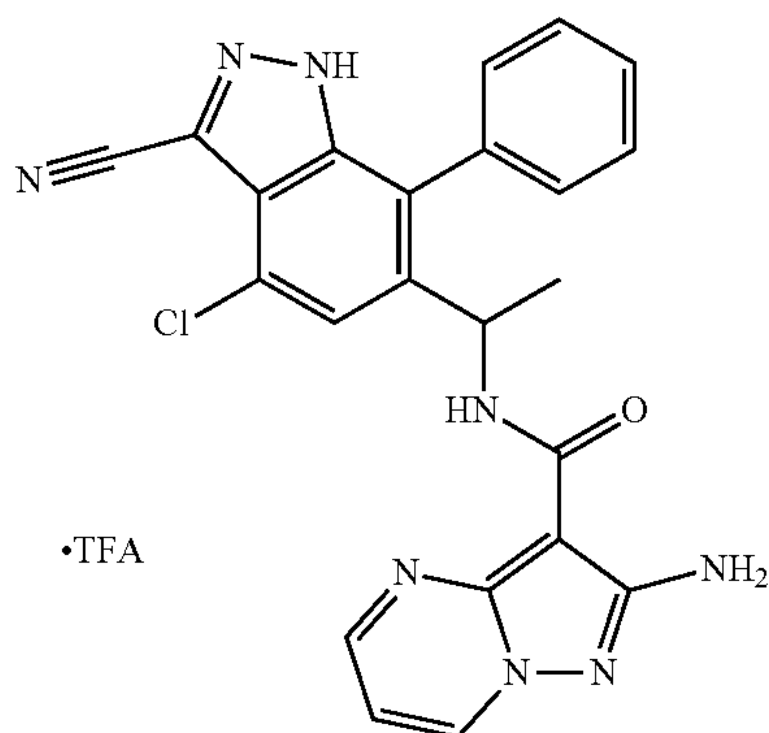
Step 1. 1-(4-chloro-3-iodo-7-phenyl-1H-indazol-6-yl)ethanone
