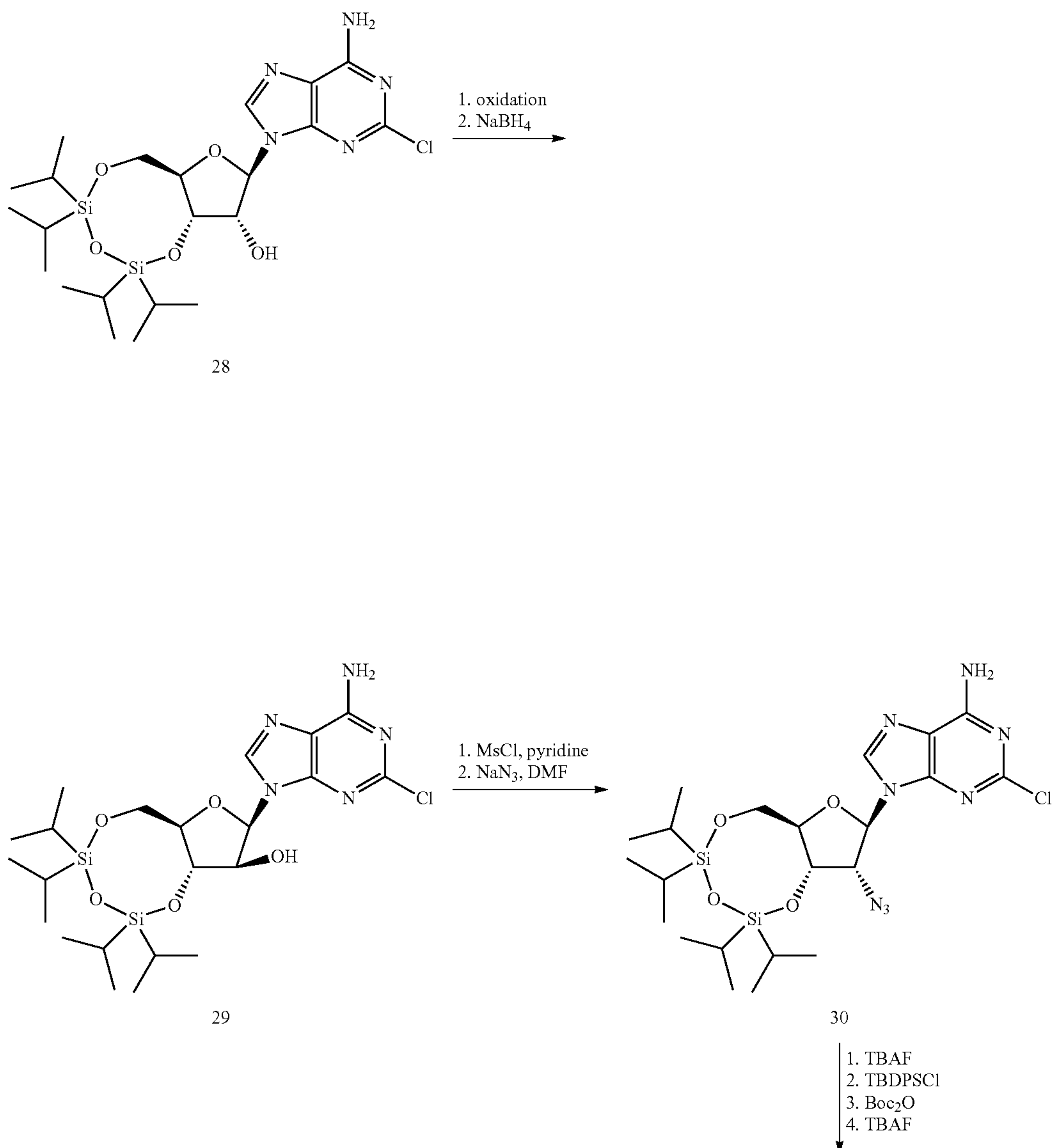
Scheme 6
