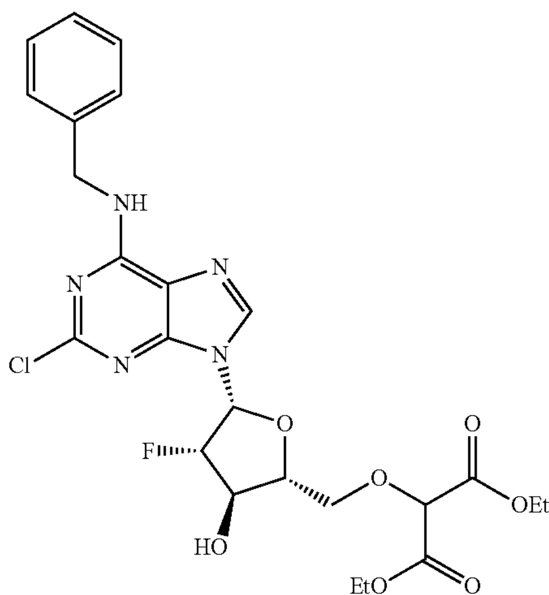
diethyl 2-(((2R,3R,4S,5R)-5-(6-(benzylamino)-2-chloro-9H-purin-9-yl)-4-fluoro-3-hydroxytetrahydrofuran-2-yl)methoxy)malonate;
