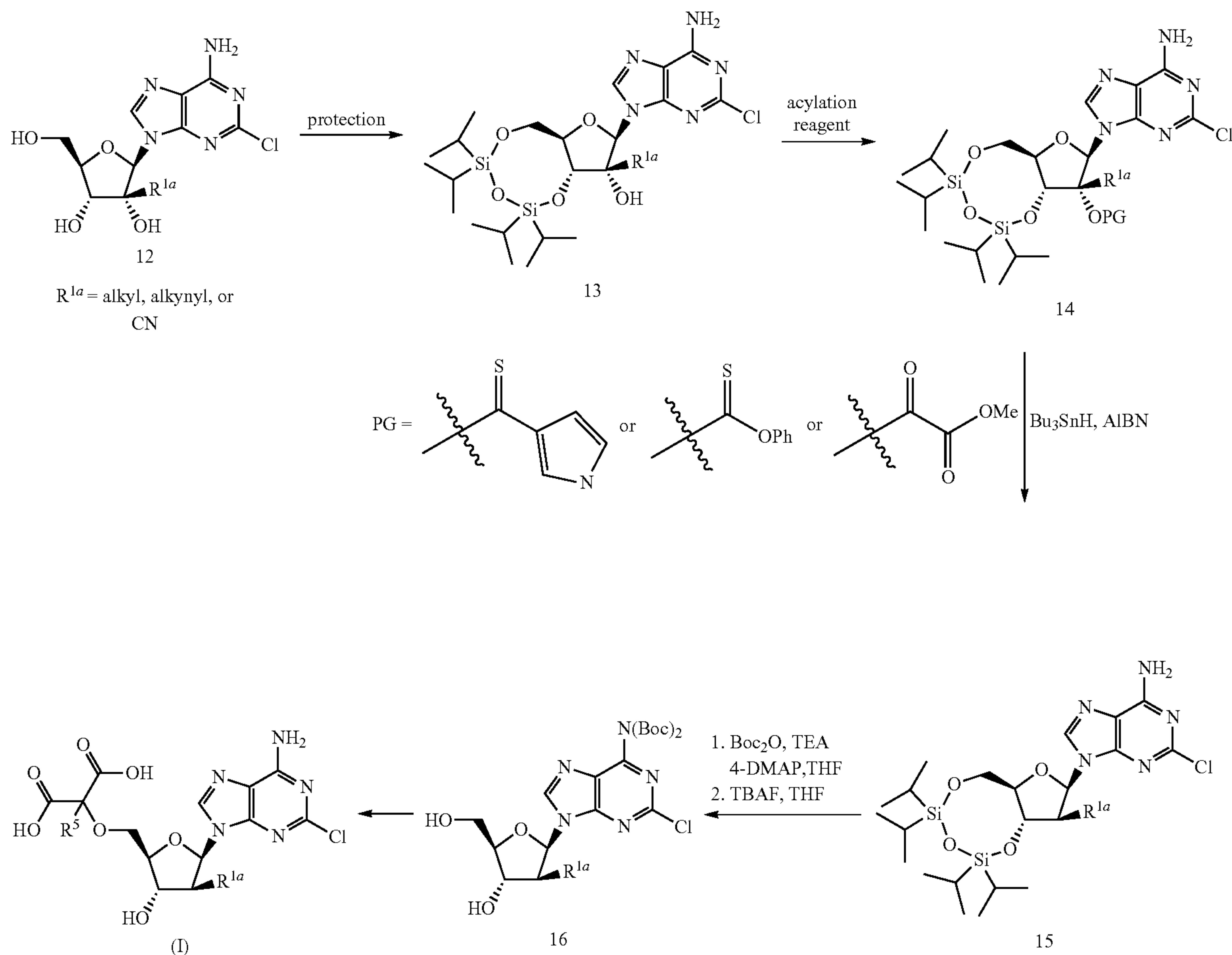
Scheme 3
