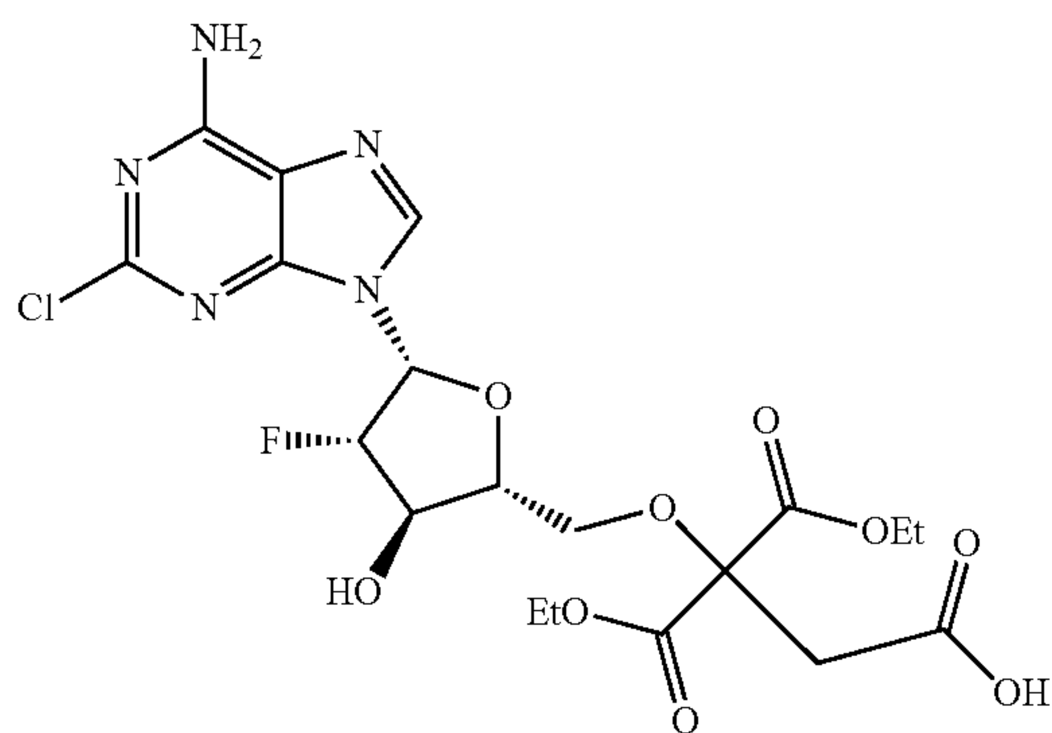
3-(((2R,3R,4S,5R)-5-(6-amino-2-chloro-9H-purin-9-yl)-4-fluoro-3-hydroxytetrahydrofuran-2-yl)methoxy)-4-ethoxy-3-(ethoxycarbonyl)-4-oxobutanoic acid;
