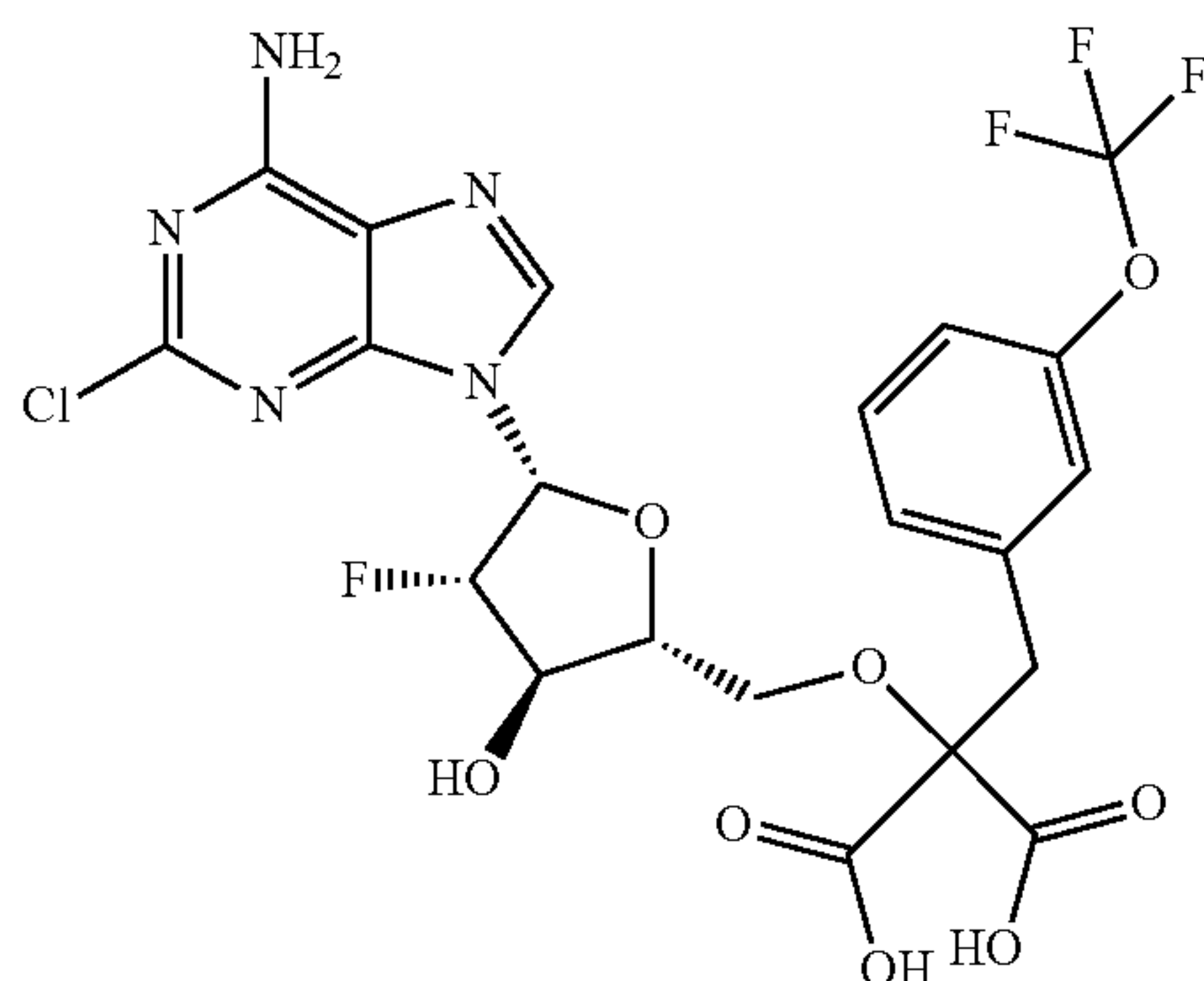
2-(((2R,3R,4S,5R)-5-(6-amino-2-chloro-9H-purin-9-yl)-4-fluoro-3-hydroxytetrahydrofuran-2-yl)methoxy)-2-(3-(trifluoromethoxy)benzyl)malonic acid;
