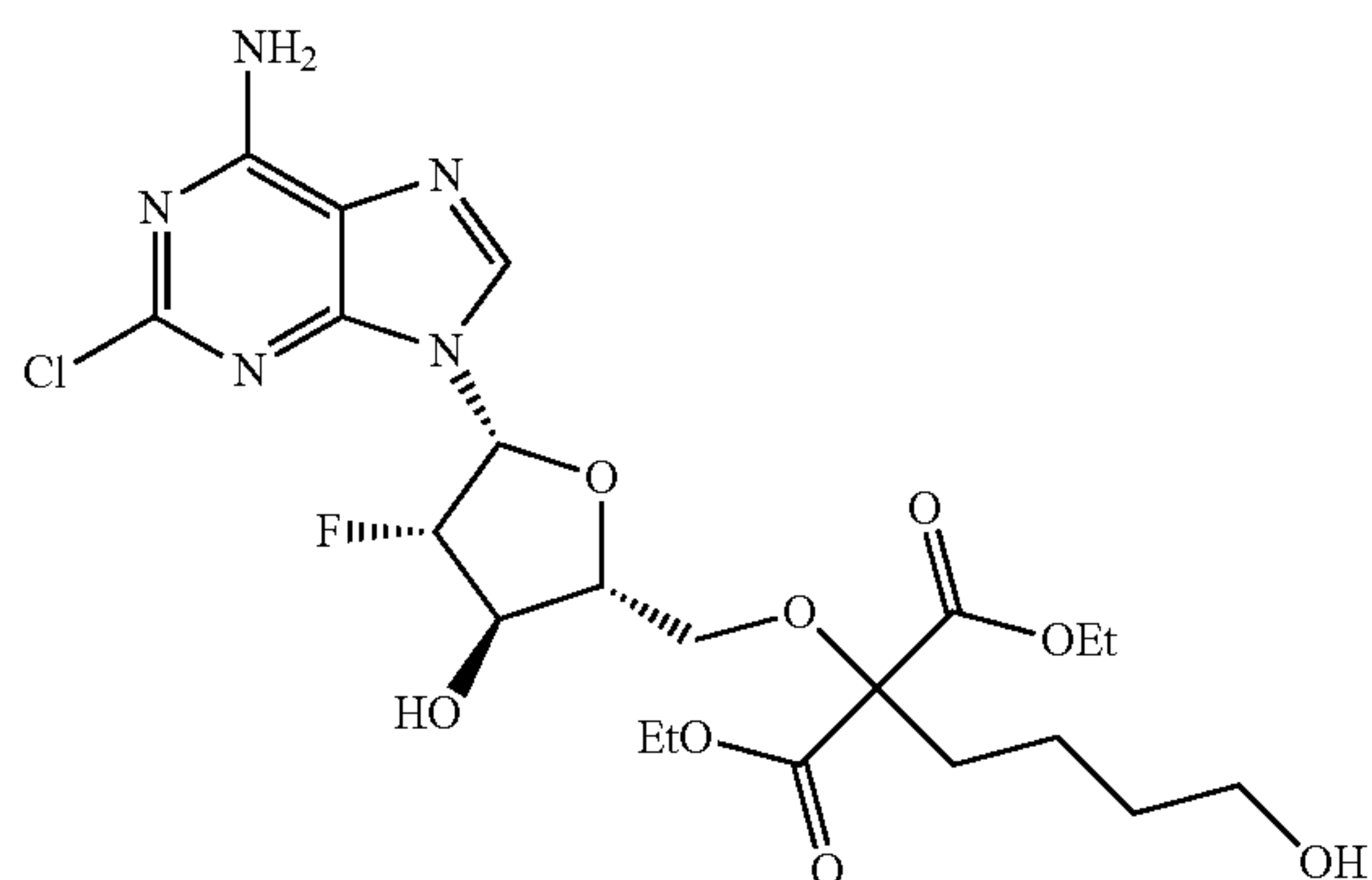
diethyl 2-(((2R,3R,4S,5R)-5-(6-amino-2-chloro-9H-purin-9-yl)-4-fluoro-3-hydroxytetrahydrofuran-2-yl)methoxy)-2-(4-hydroxybutyl)malonate;
