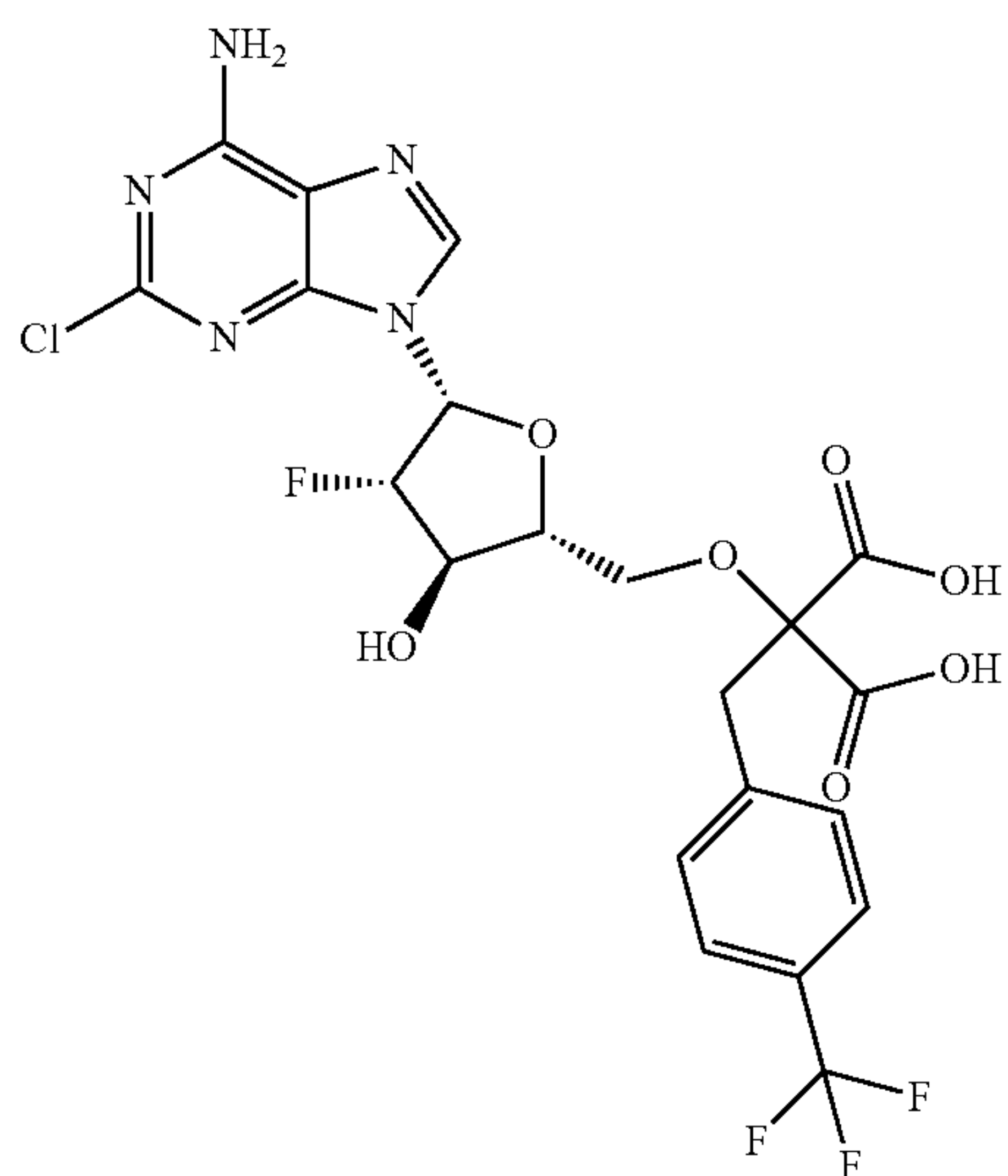
2-(((2R,3R,4S,5R)-5-(6-amino-2-chloro-9H-purin-9-yl)-4-fluoro-3-hydroxytetrahydrofuran-2-yl)methoxy)-2-(4-(trifluoromethyl)benzyl)malonic acid;
