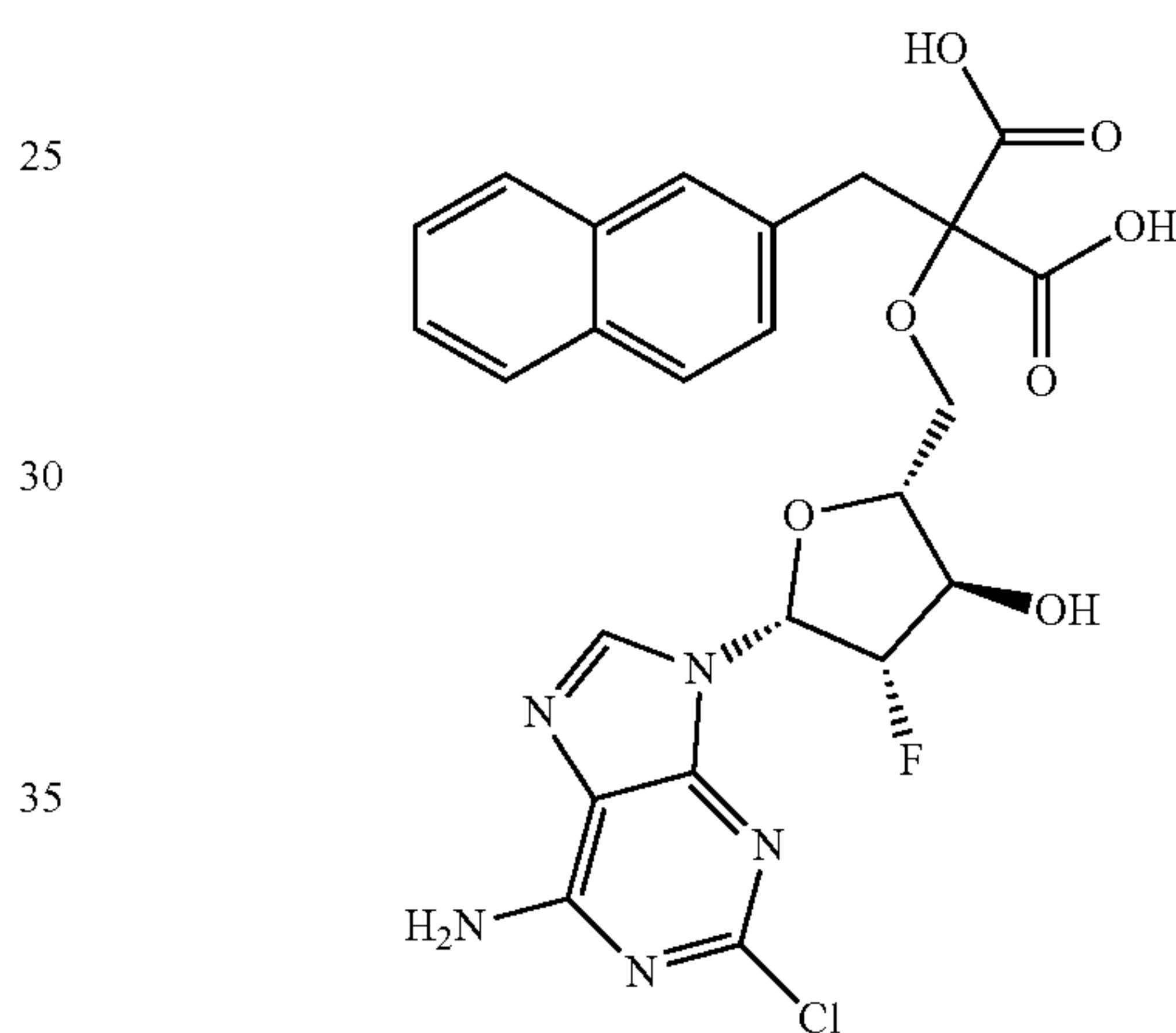
2-(((2R,3R,4S,5R)-5-(6-amino-2-chloro-9H-purin-9-yl)-4-fluoro-3-hydroxytetrahydrofuran-2-yl)methoxy)-2-(naphthalen-2-ylmethyl)malonic acid;
