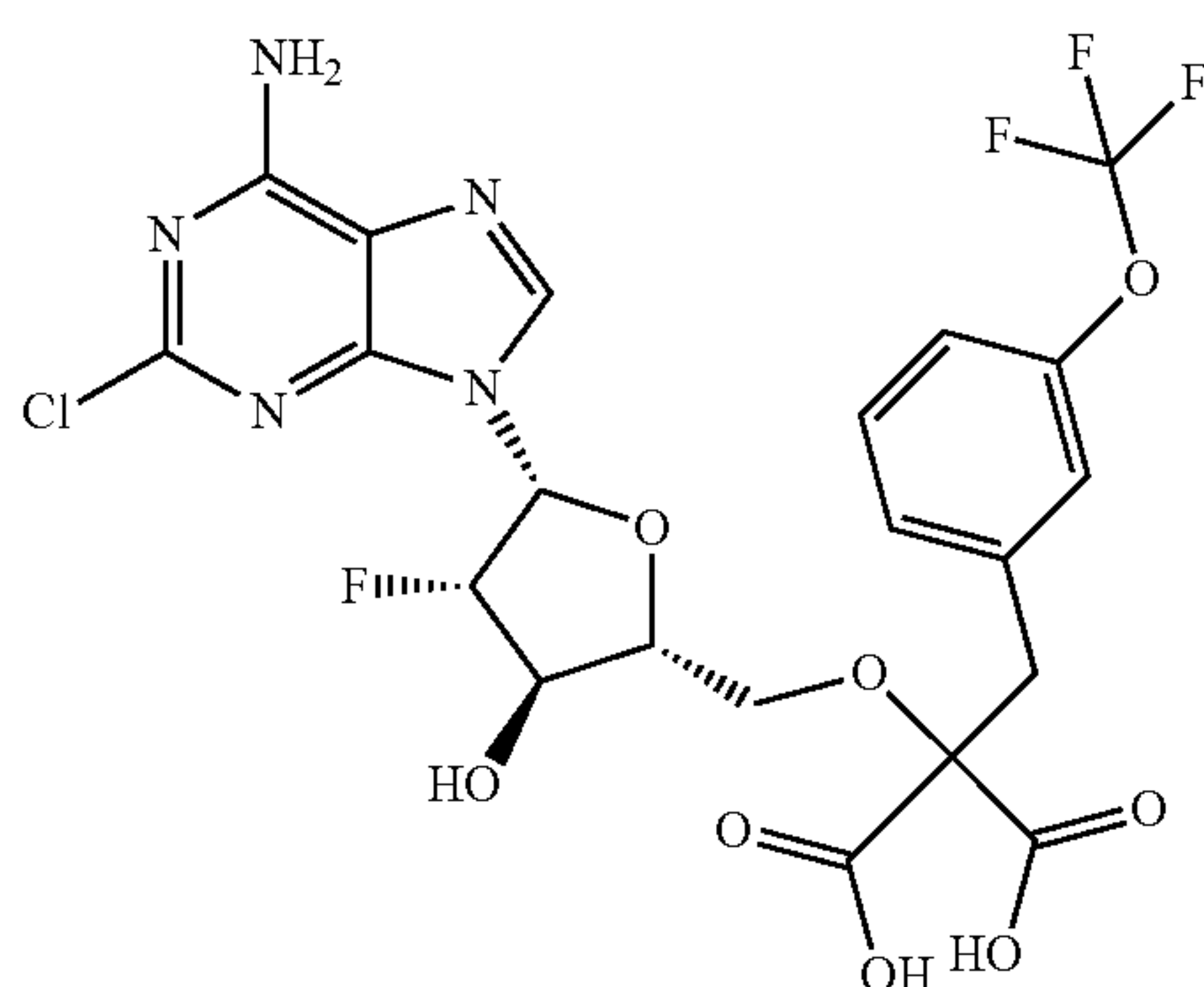
2-(((2R,3R,4S,5R)-5-(6-amino-2-chloro-9H-purin-9-yl)-4-fluoro-3-hydroxytetrahydrofuran-2-yl)methoxy)-2-(3-(trifluoromethoxy)benzyl)malonic acid;
