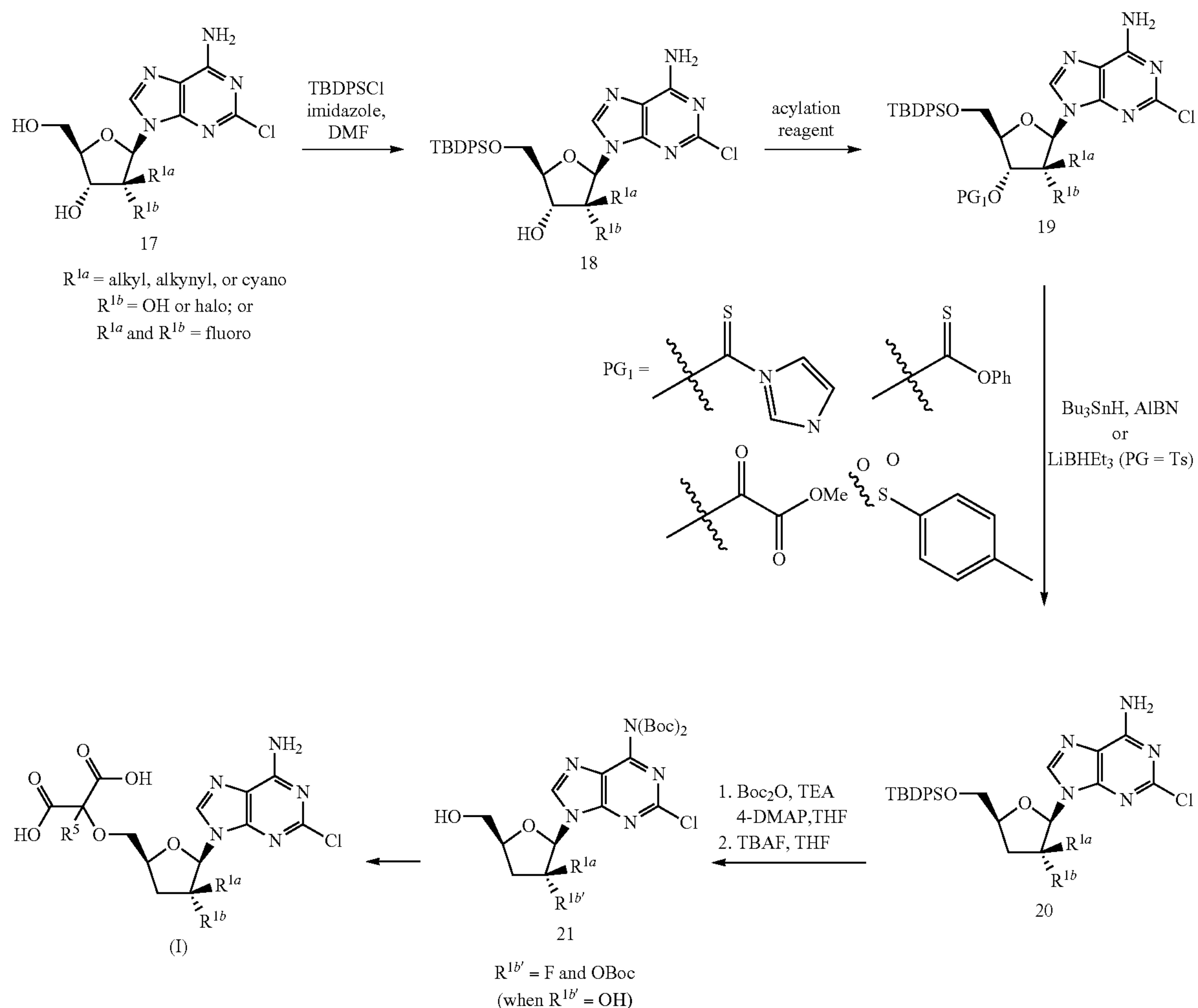
Scheme 4
