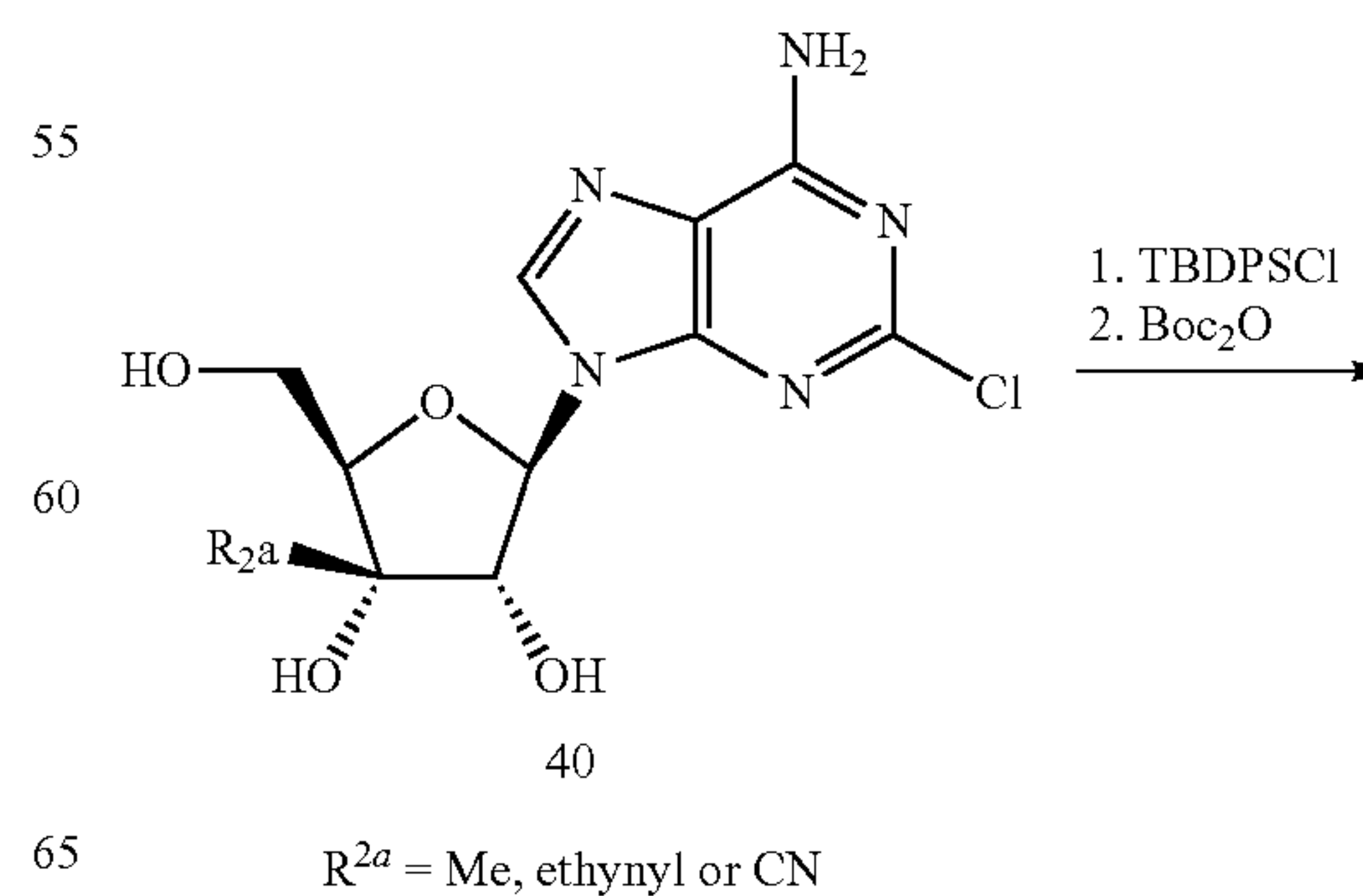
Scheme 9
