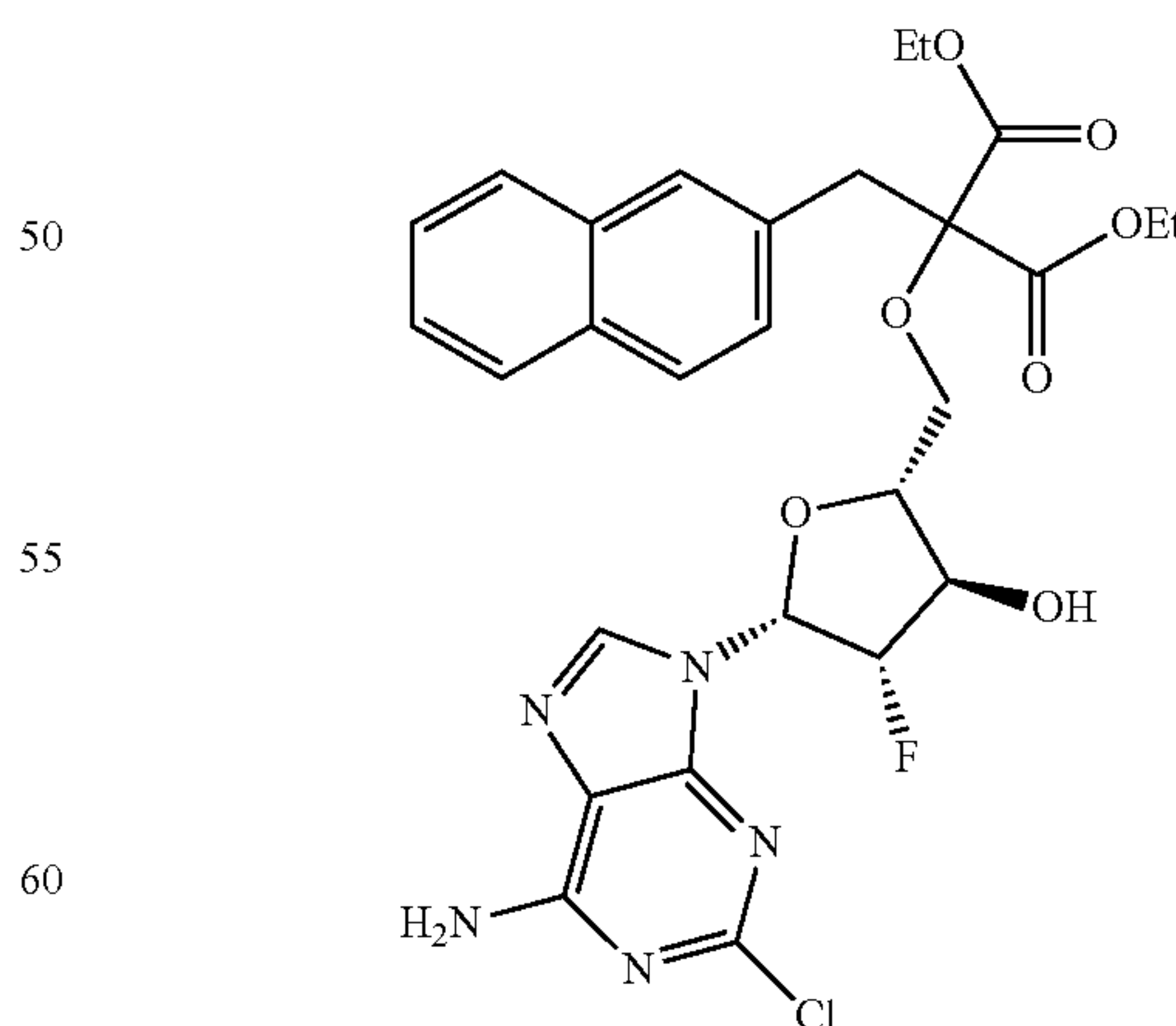
diethyl 2-(((2R,3R,4S,5R)-5-(6-amino-2-chloro-9H-purin-9-yl)-4-fluoro-3-hydroxytetrahydrofuran-2-yl)methoxy)-2-(naphthalen-2-ylmethyl)malonate;
