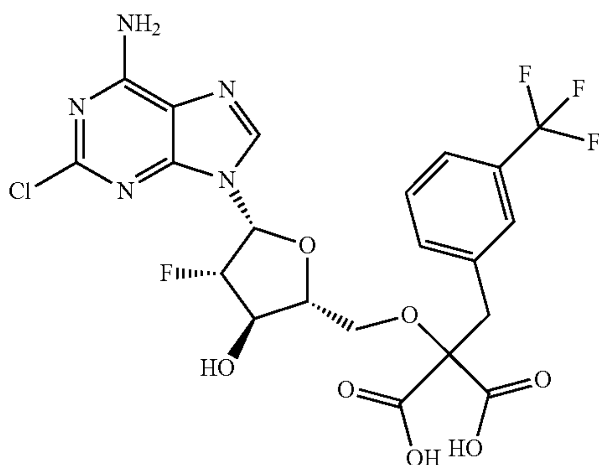
2-(((2R,3R,4S,5R)-5-(6-amino-2-chloro-9H-purin-9-yl)-4-fluoro-3-hydroxytetrahydrofuran-2-yl)methoxy)-2-(3-(trifluoromethyl)benzyl)malonic acid;
