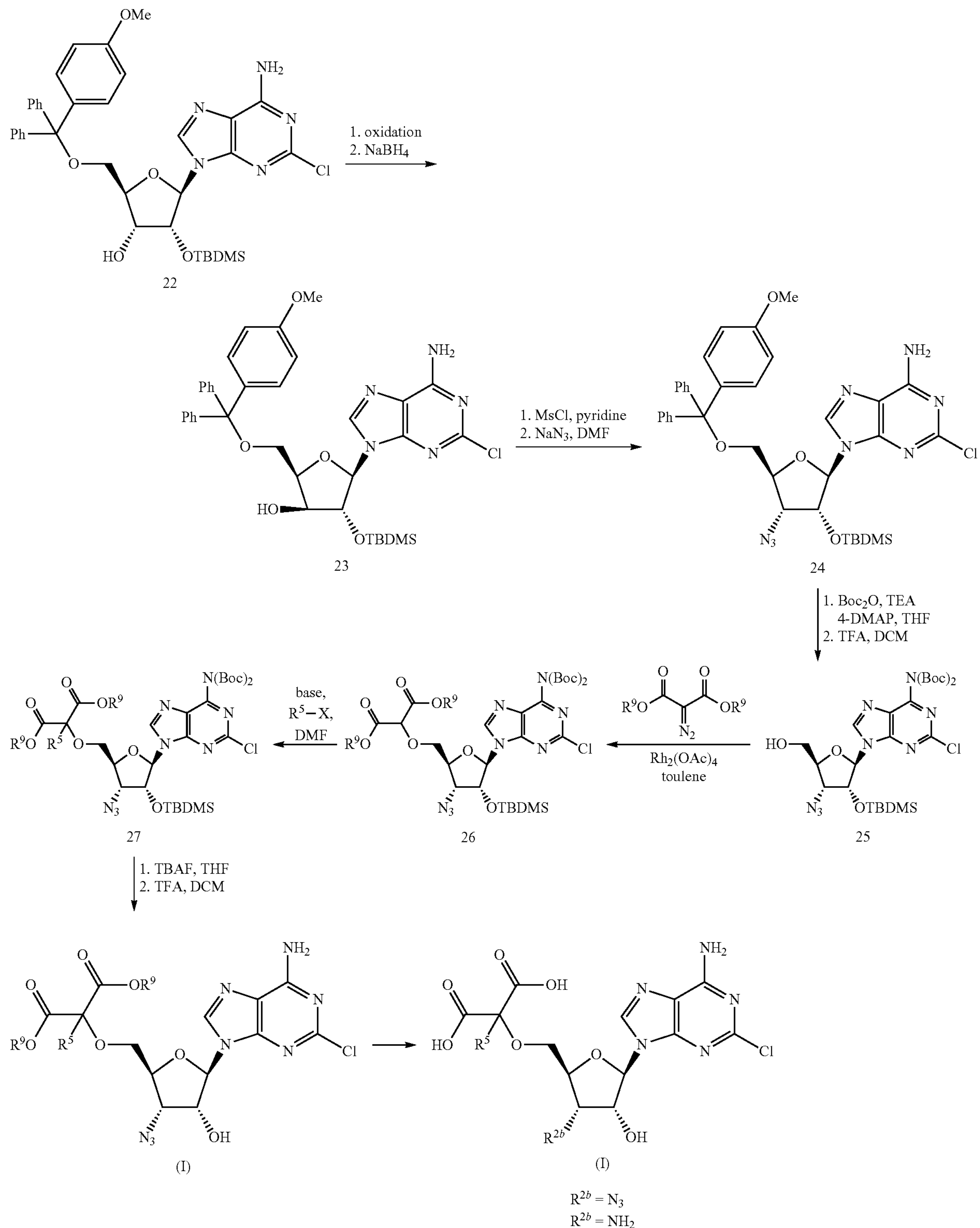
Scheme 5
