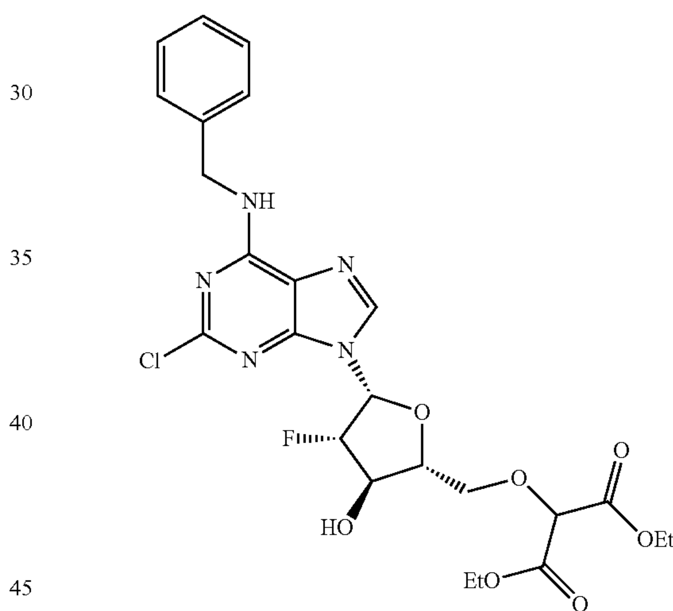
diethyl 2-(((2R,3R,4S,5R)-5-(6-(benzylamino)-2-chloro-9H-purin-9-yl)-4-fluoro-3-hydroxytetrahydrofuran-2-yl)methoxy)malonate;
