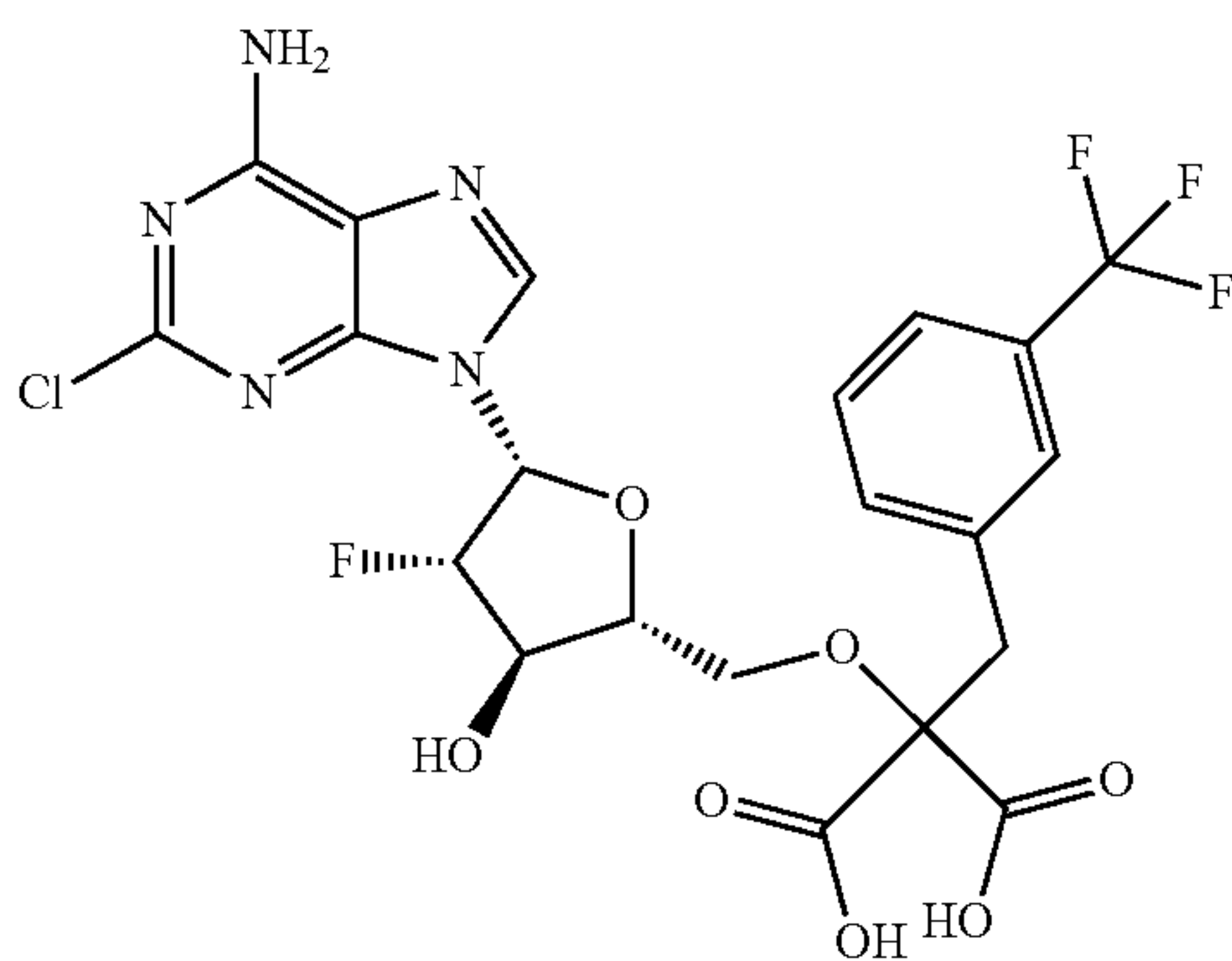
2-(((2R,3R,4S,5R)-5-(6-amino-2-chloro-9H-purin-9-yl)-4-fluoro-3-hydroxytetrahydrofuran-2-yl)methoxy)-2-(3-(trifluoromethyl)benzyl)malonic acid;
