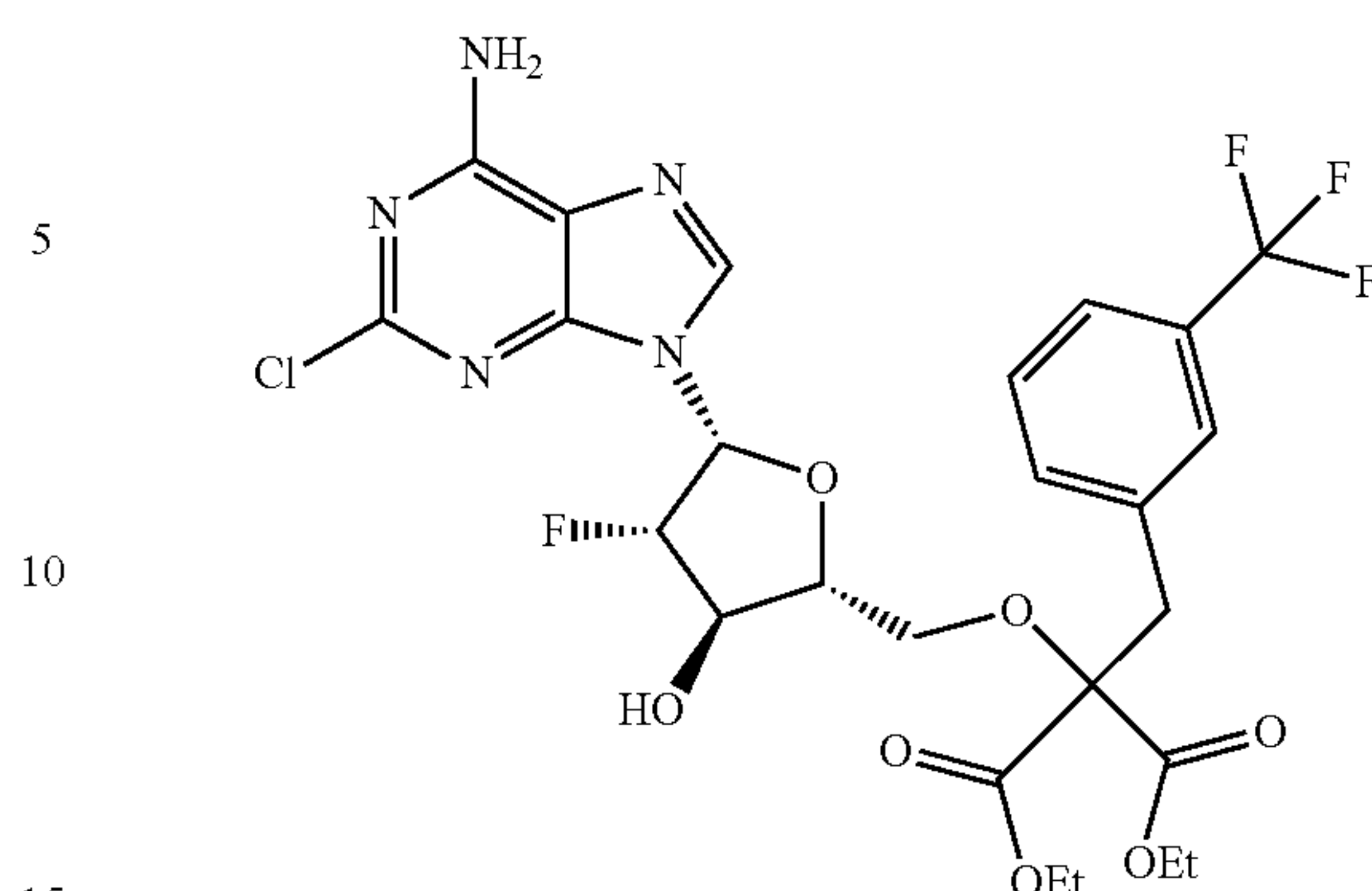
diethyl 2-(((2R,3R,4S,5R)-5-(6-amino-2-chloro-9H-purin-9-yl)-4-fluoro-3-hydroxytetrahydrofuran-2-yl)methoxy)-2-(3-(trifluoromethyl)benzyl)malonate;
