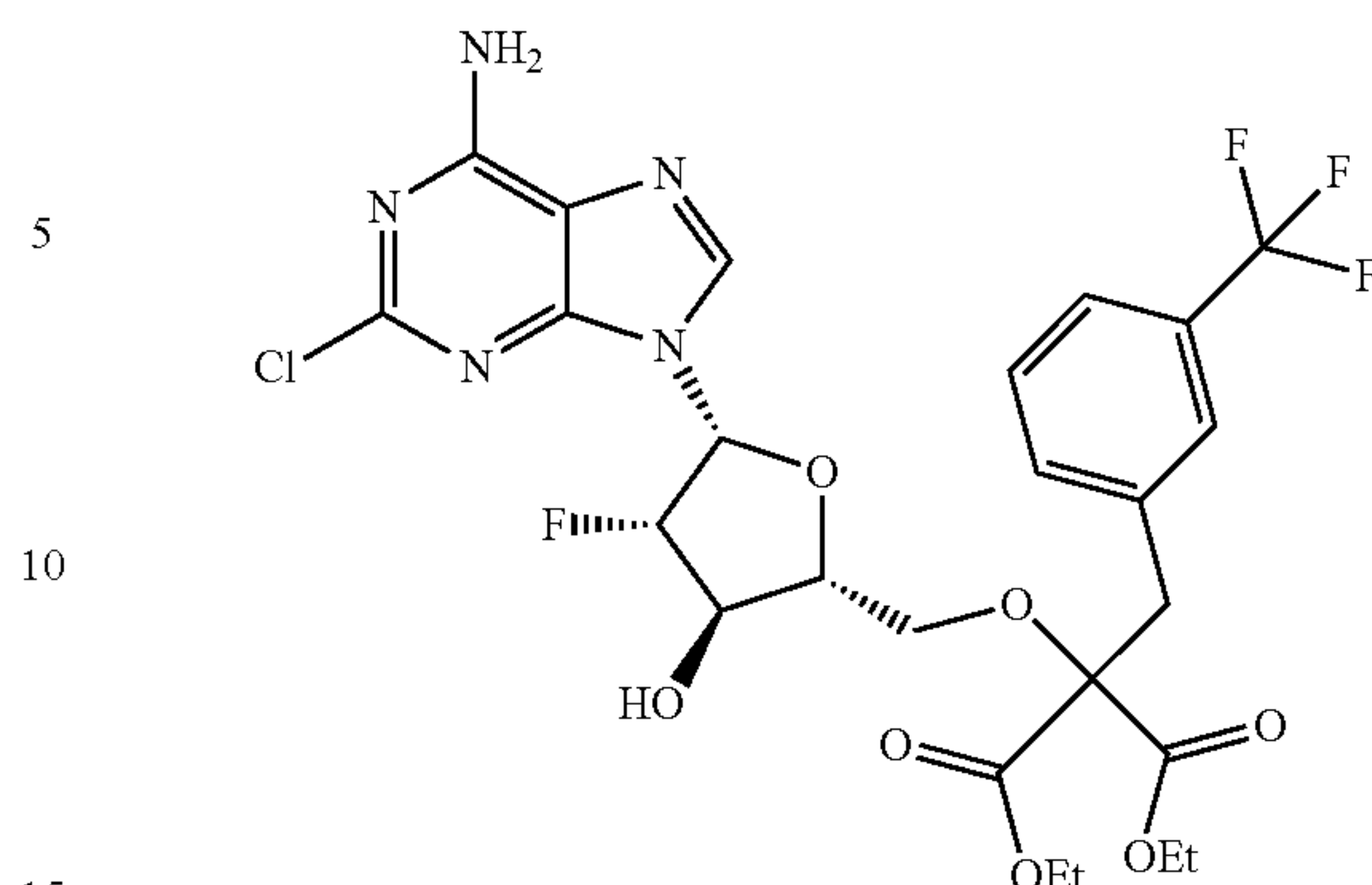
diethyl 2-(((2R,3R,4S,5R)-5-(6-amino-2-chloro-9H-purin-9-yl)-4-fluoro-3-hydroxytetrahydrofuran-2-yl)methoxy)-2-(3-(trifluoromethyl)benzyl)malonate;
