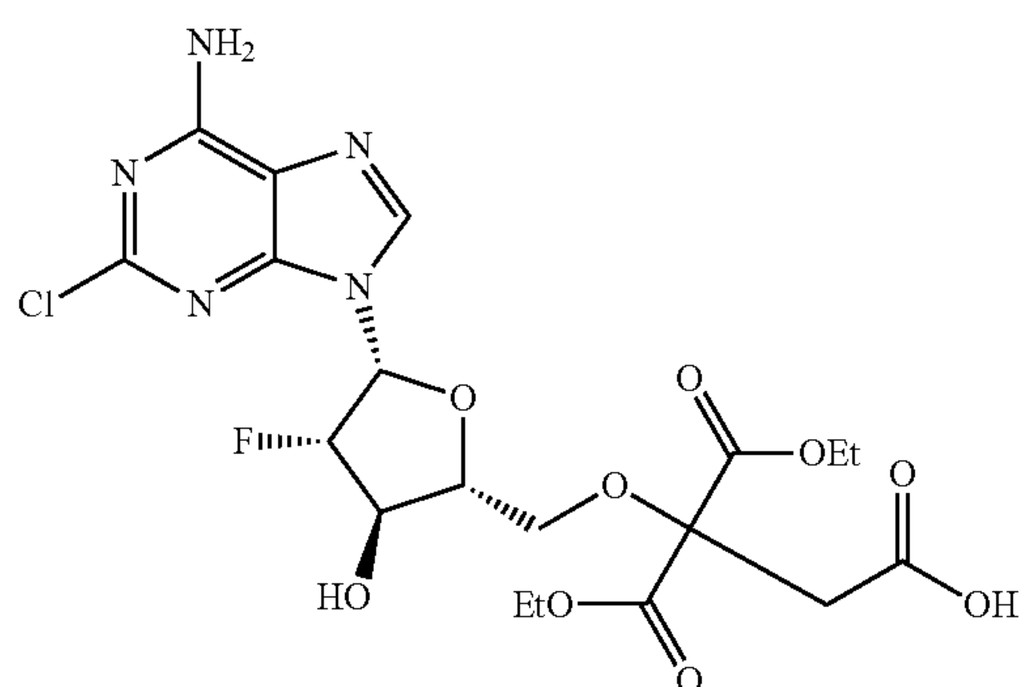
3-(((2R,3R,4S,5R)-5-(6-amino-2-chloro-9H-purin-9-yl)-4-fluoro-3-hydroxytetrahydrofuran-2-yl)methoxy)-4-ethoxy-3-(ethoxycarbonyl)-4-oxobutanoic acid;
