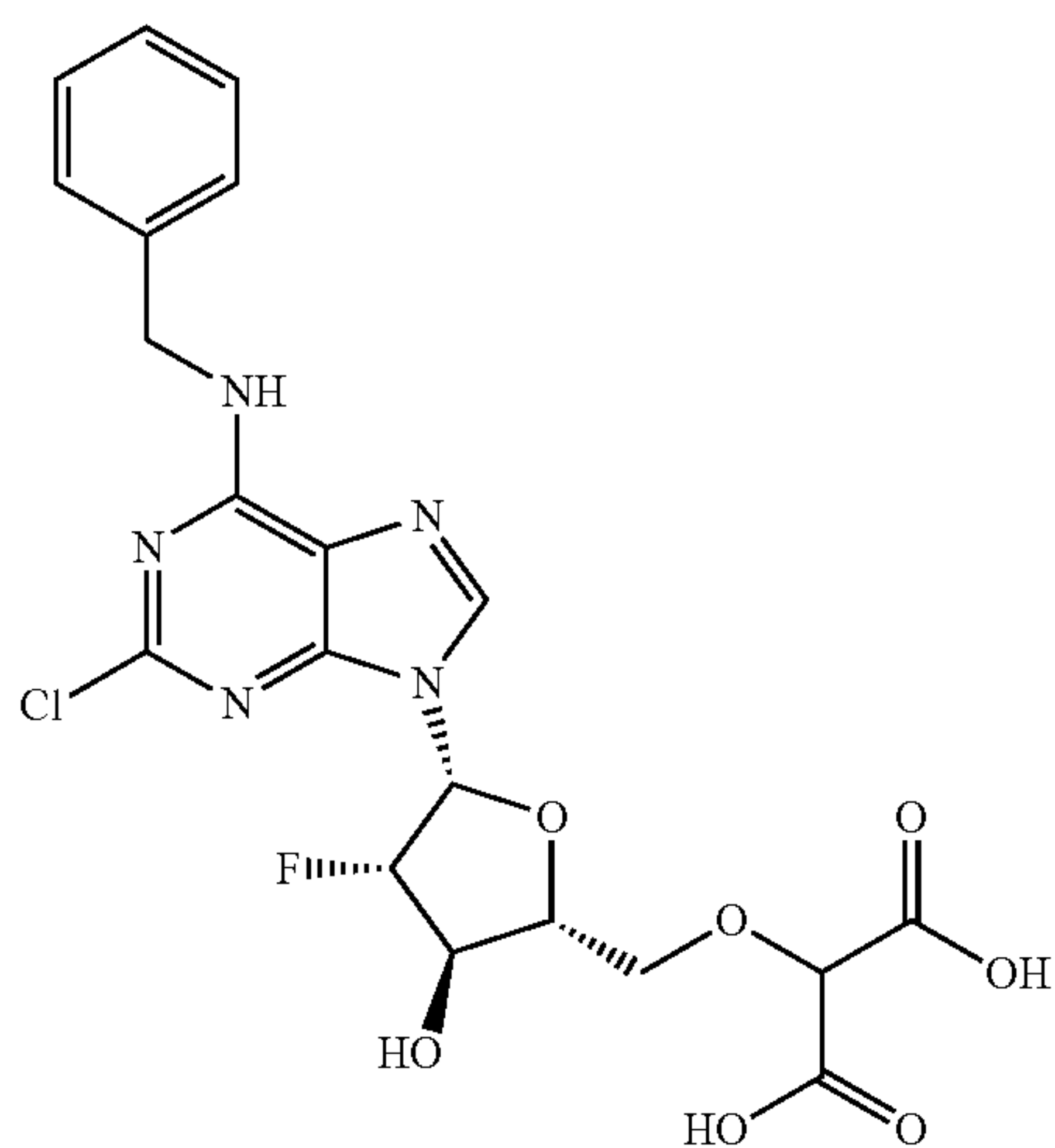
2-(((2R,3R,4S,5R)-5-(6-(benzylamino)-2-chloro-9H-purin-9-yl)-4-fluoro-3-hydroxytetrahydrofuran-2-yl)methoxy)malonic acid;
