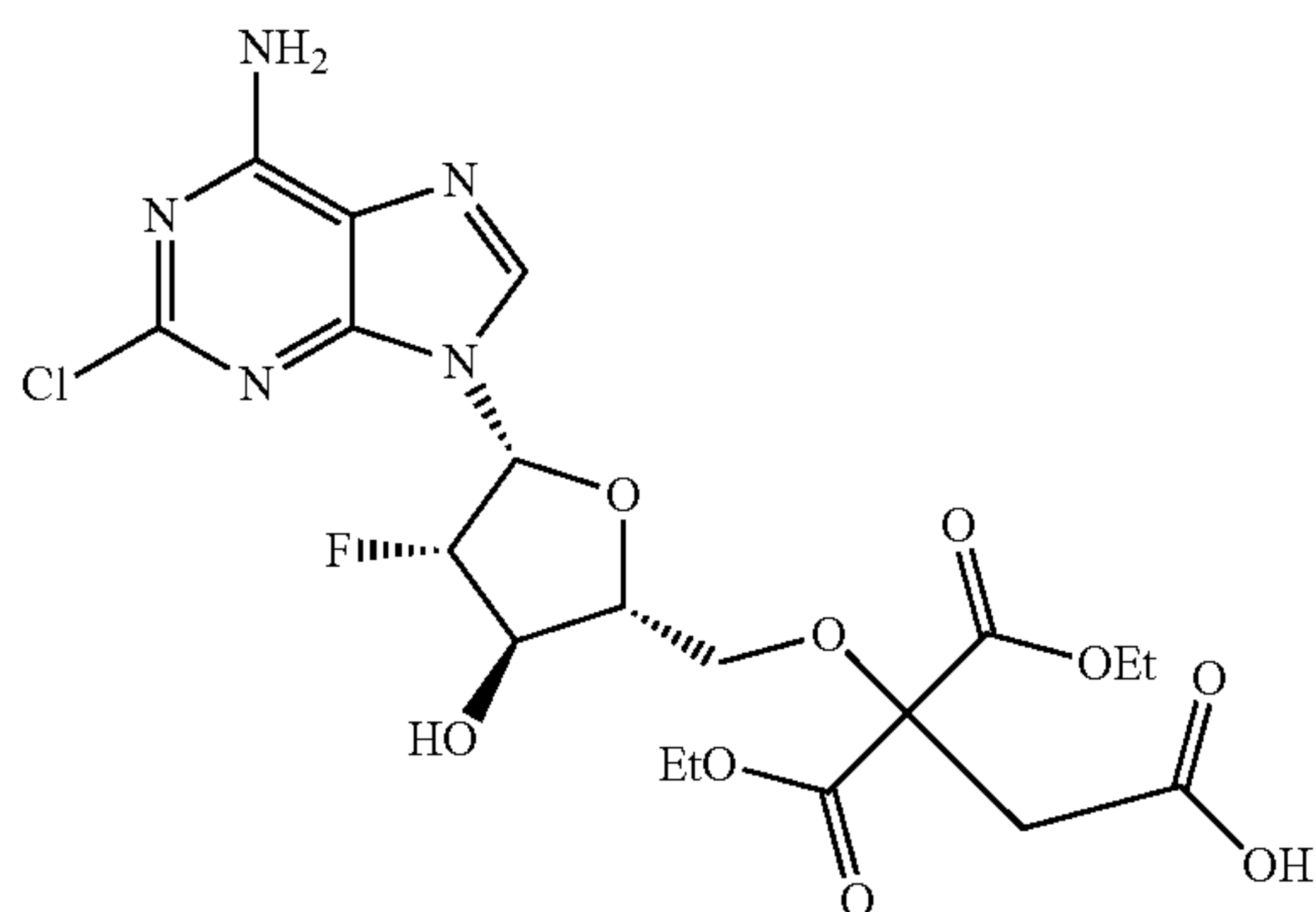
3-(((2R,3R,4S,5R)-5-(6-amino-2-chloro-9H-purin-9-yl)-4-fluoro-3-hydroxytetrahydrofuran-2-yl)methoxy)-4-ethoxy-3-(ethoxycarbonyl)-4-oxobutanoic acid;
