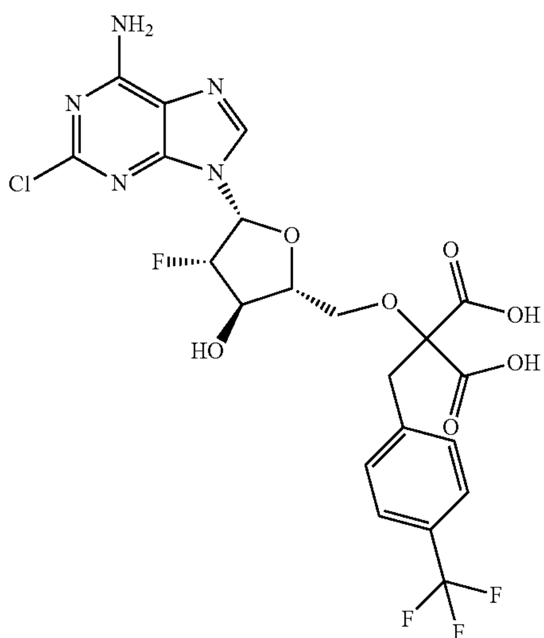
2-(((2R,3R,4S,5R)-5-(6-amino-2-chloro-9H-purin-9-yl)-4-fluoro-3-hydroxytetrahydrofuran-2-yl)methoxy)-2-(4-(trifluoromethyl)benzyl)malonic acid;
