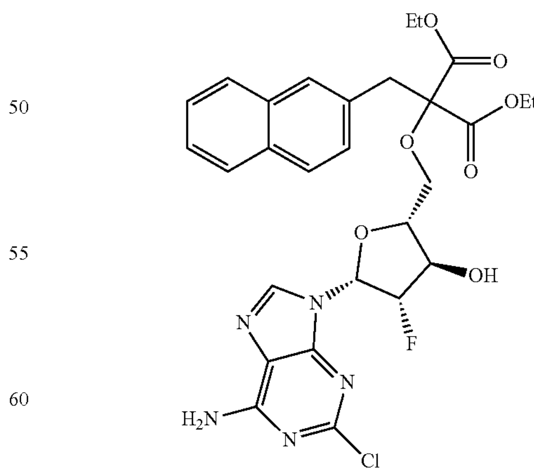
diethyl 2-(((2R,3R,4S,5R)-5-(6-amino-2-chloro-9H-purin-9-yl)-4-fluoro-3-hydroxytetrahydrofuran-2-yl)methoxy)-2-(naphthalen-2-ylmethyl)malonate;
