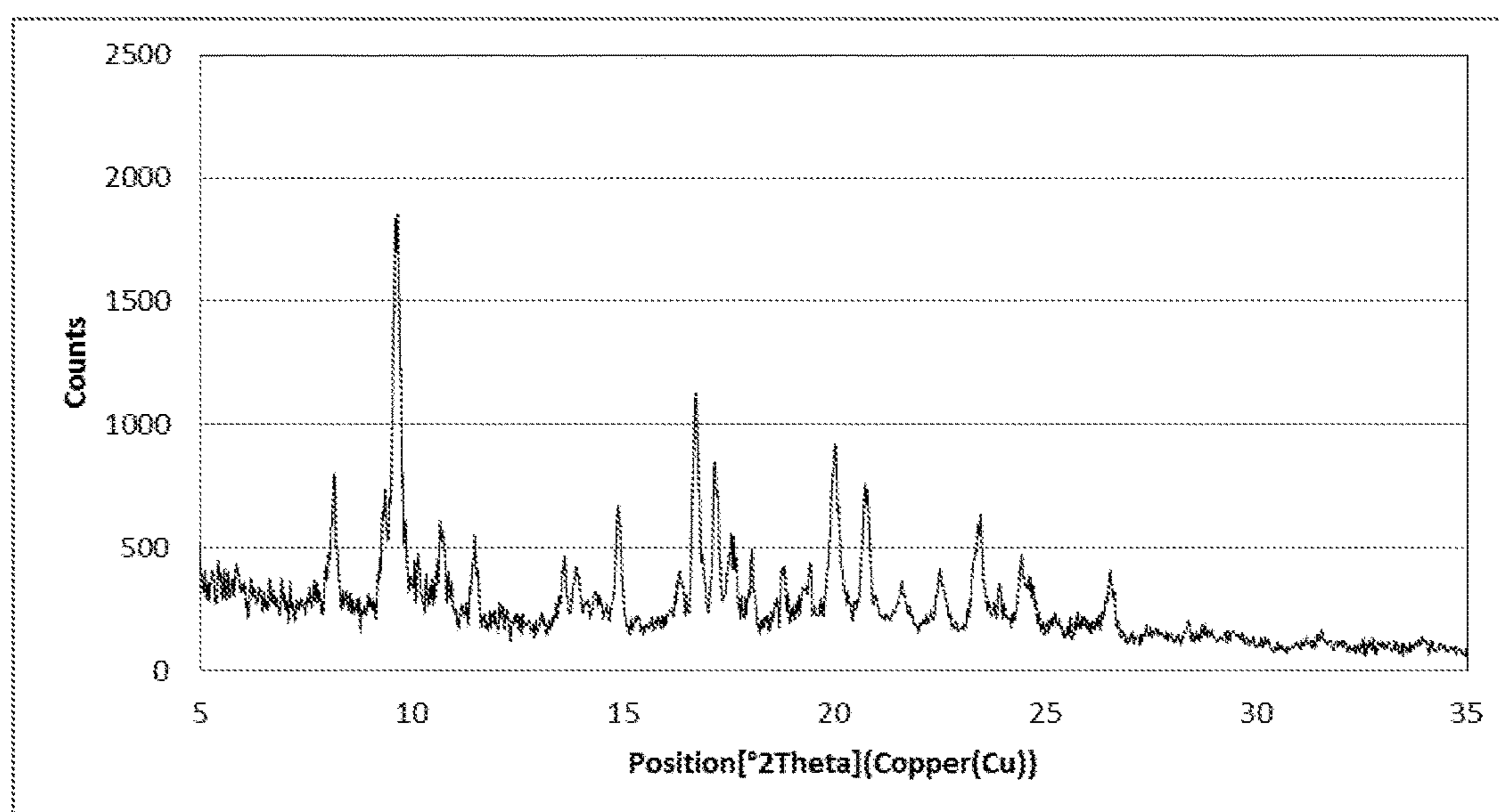
Figure 7. XRPD of (1R,2S)-(E)-2-(3-(4-((cis-2,6-dimethylmorpholino)methyl)styryl)-1H-indazol-6-yl)-5'-methoxyspiro[cyclopropane-1,3'-indolin]-2'-one fumarate form A
