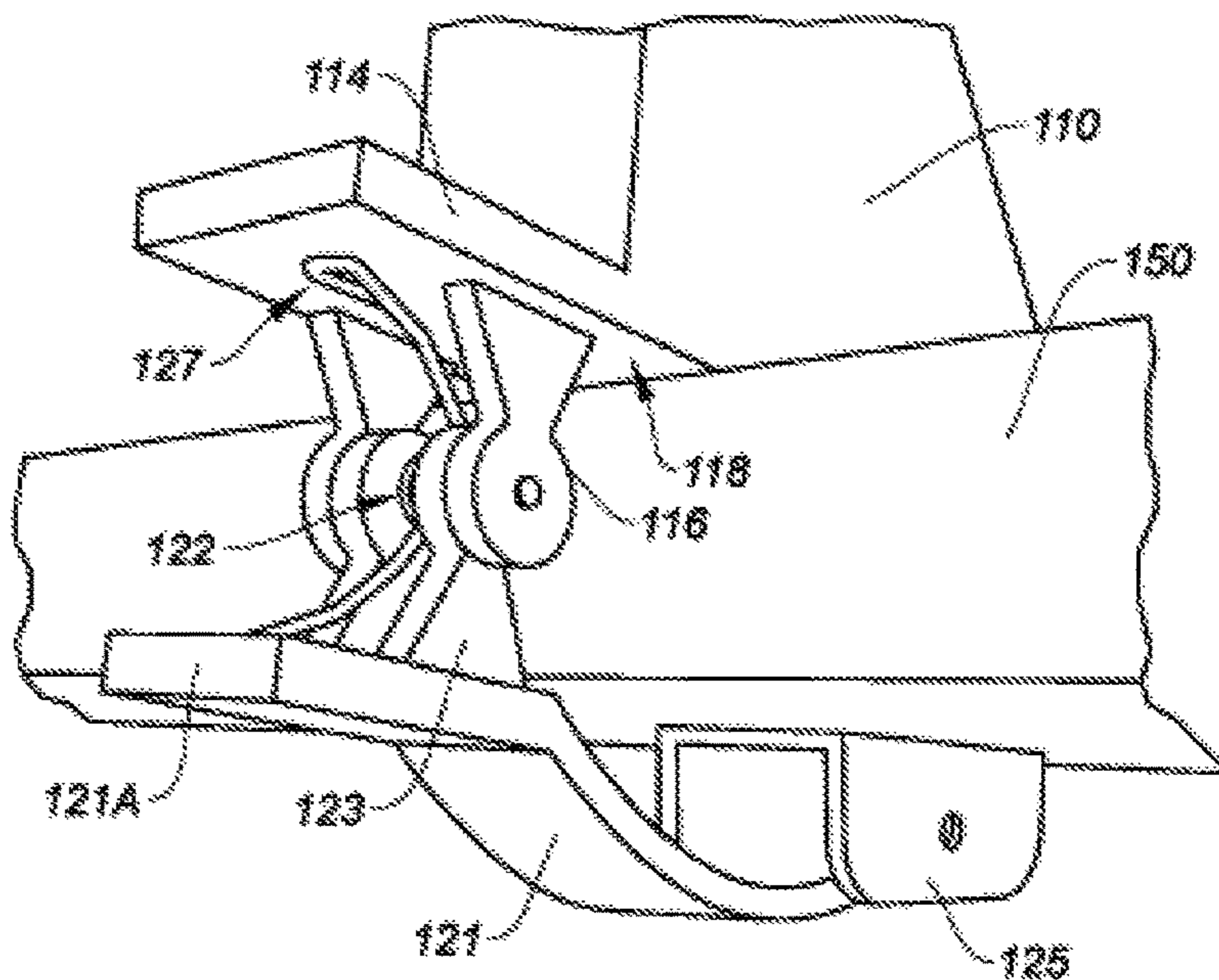
FIG. 4 (CONVENTIONAL ART)
