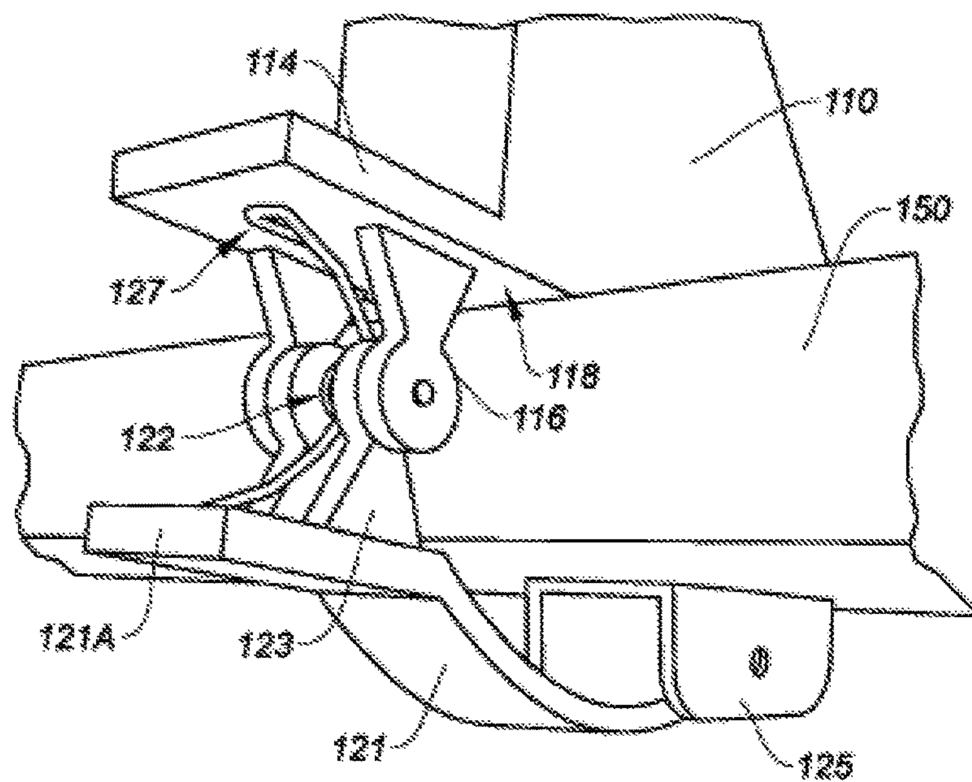
FIG. 4 (CONVENTIONAL ART)
