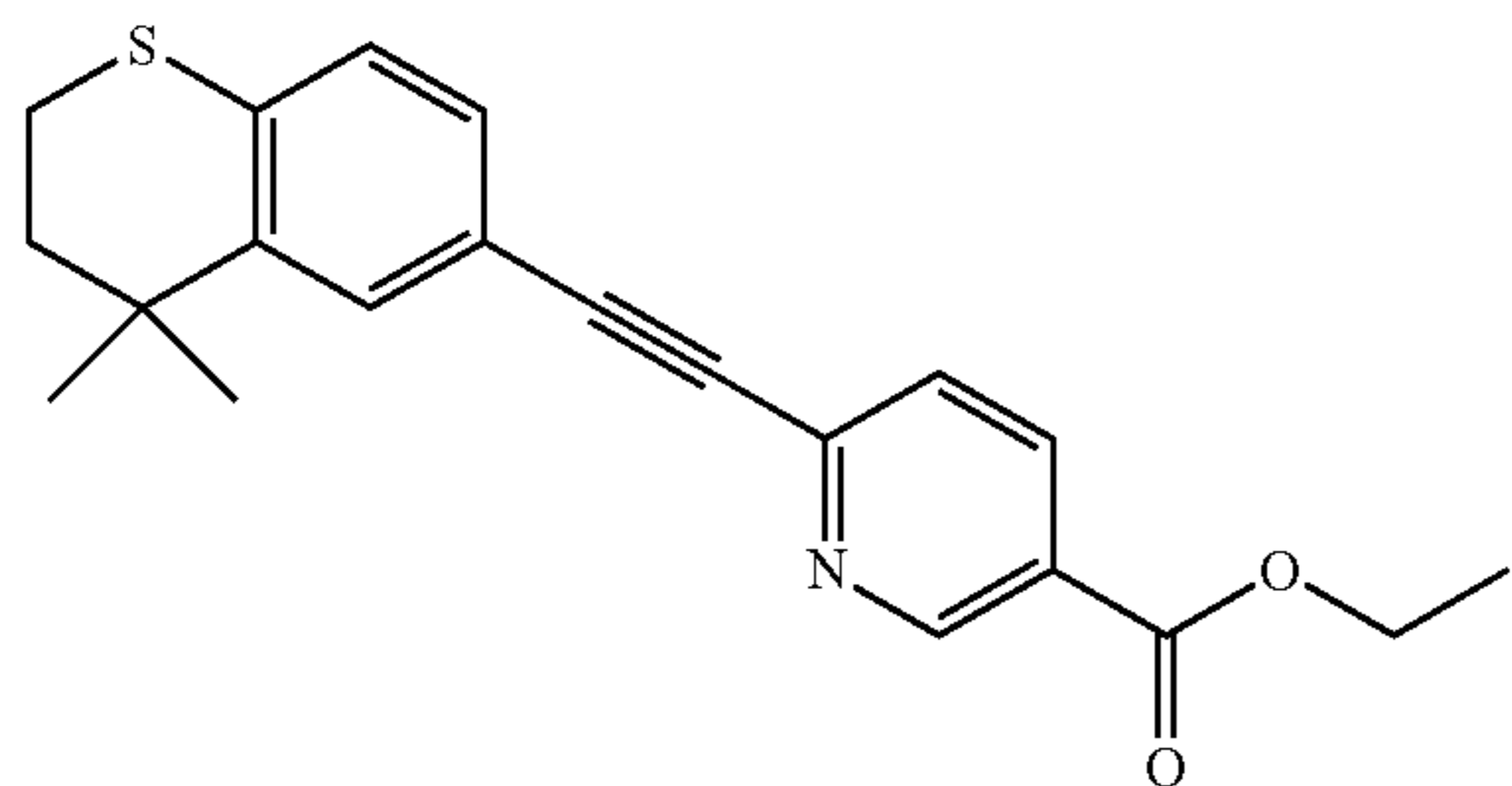
AGN 190168 (Tazarotene)
