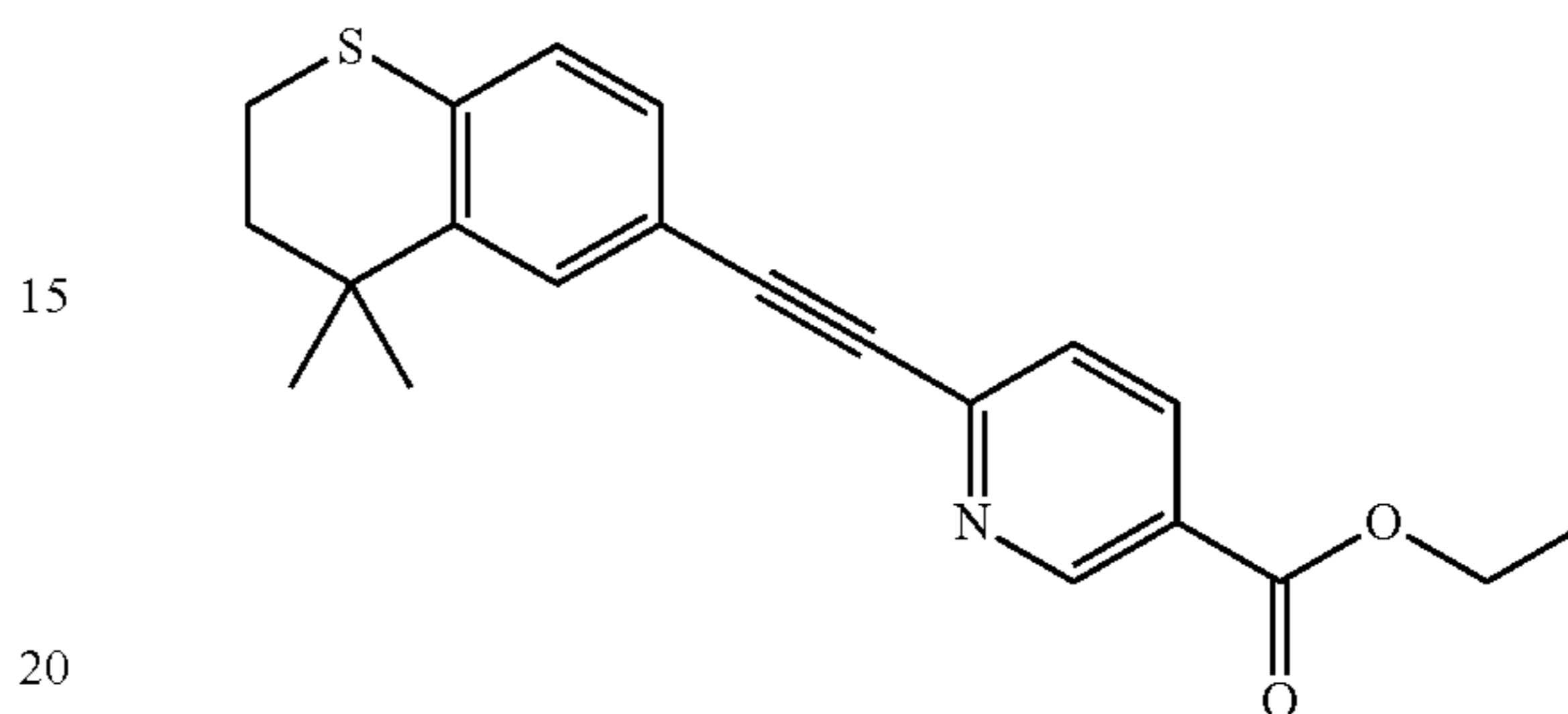
AGN 190168 (Tazarotene)
