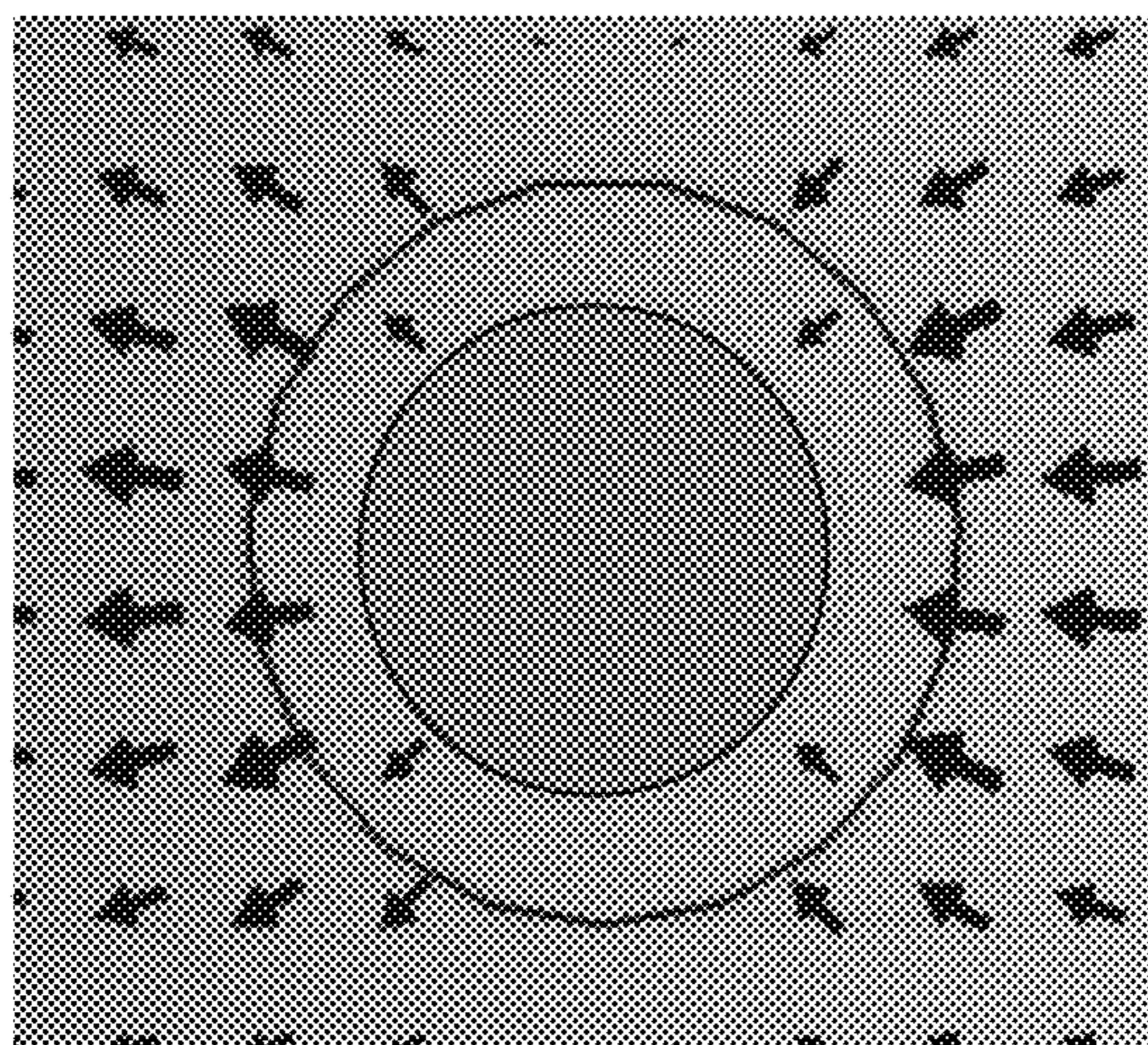
Conductor mode (HE11) 2057
