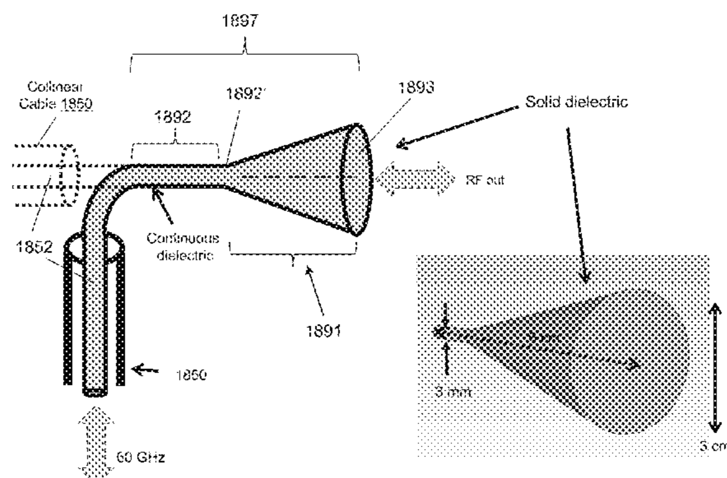
Dielectric Horn Antenna
