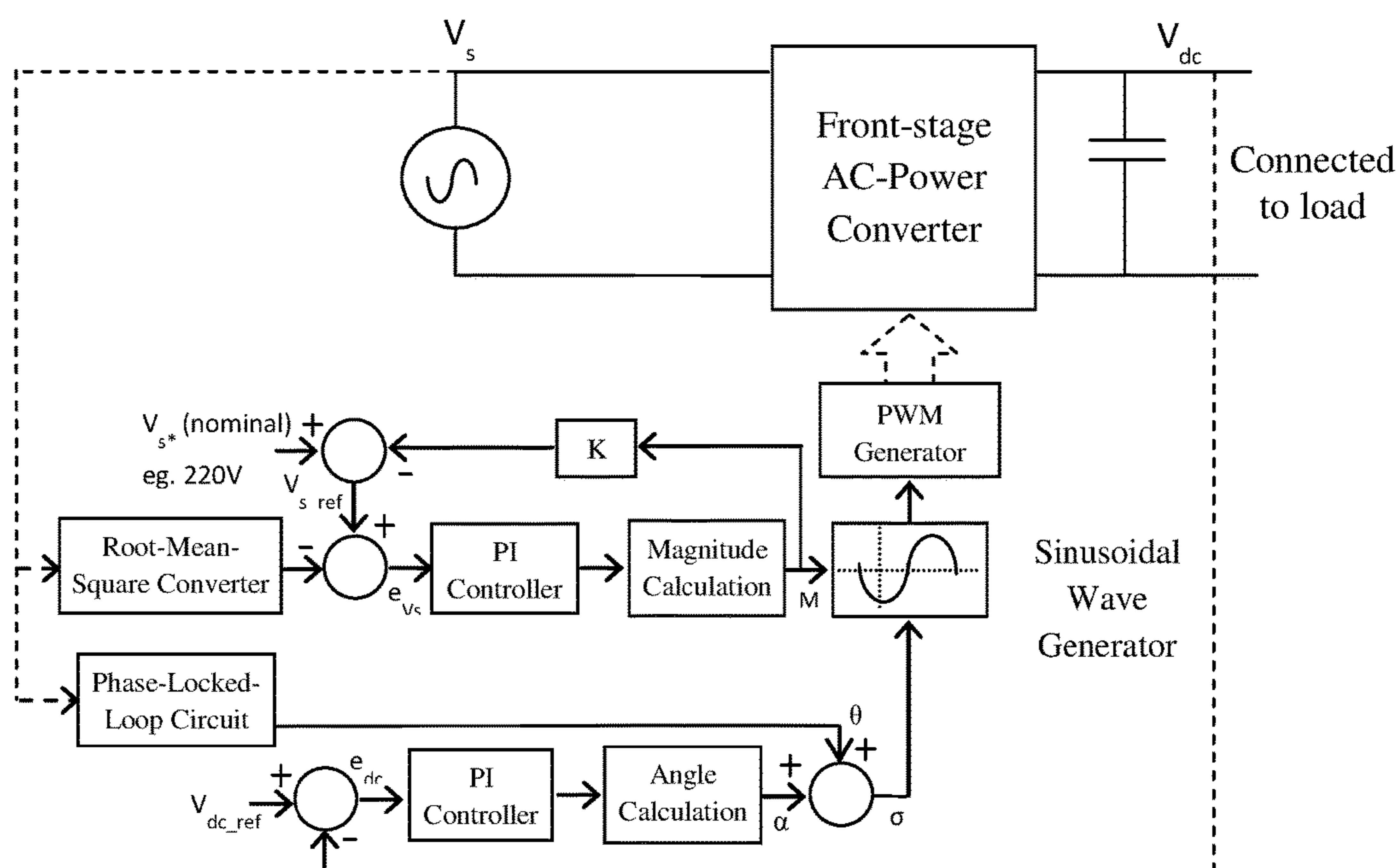
FIG. 3 (Prior Art)
