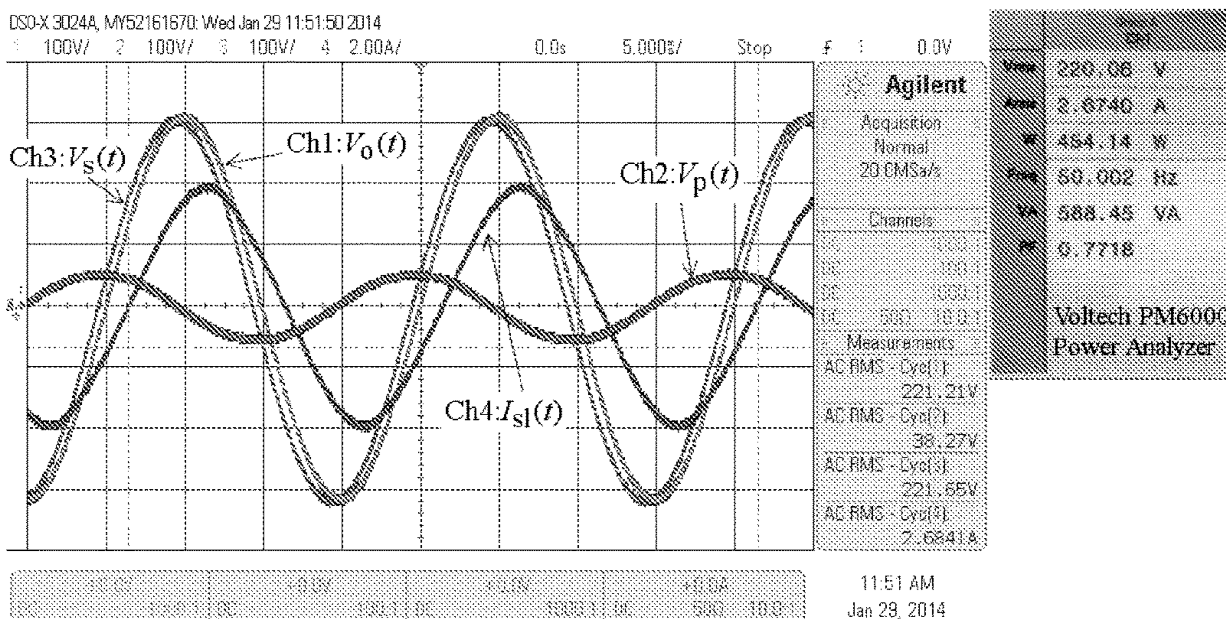
FIG. 13D
