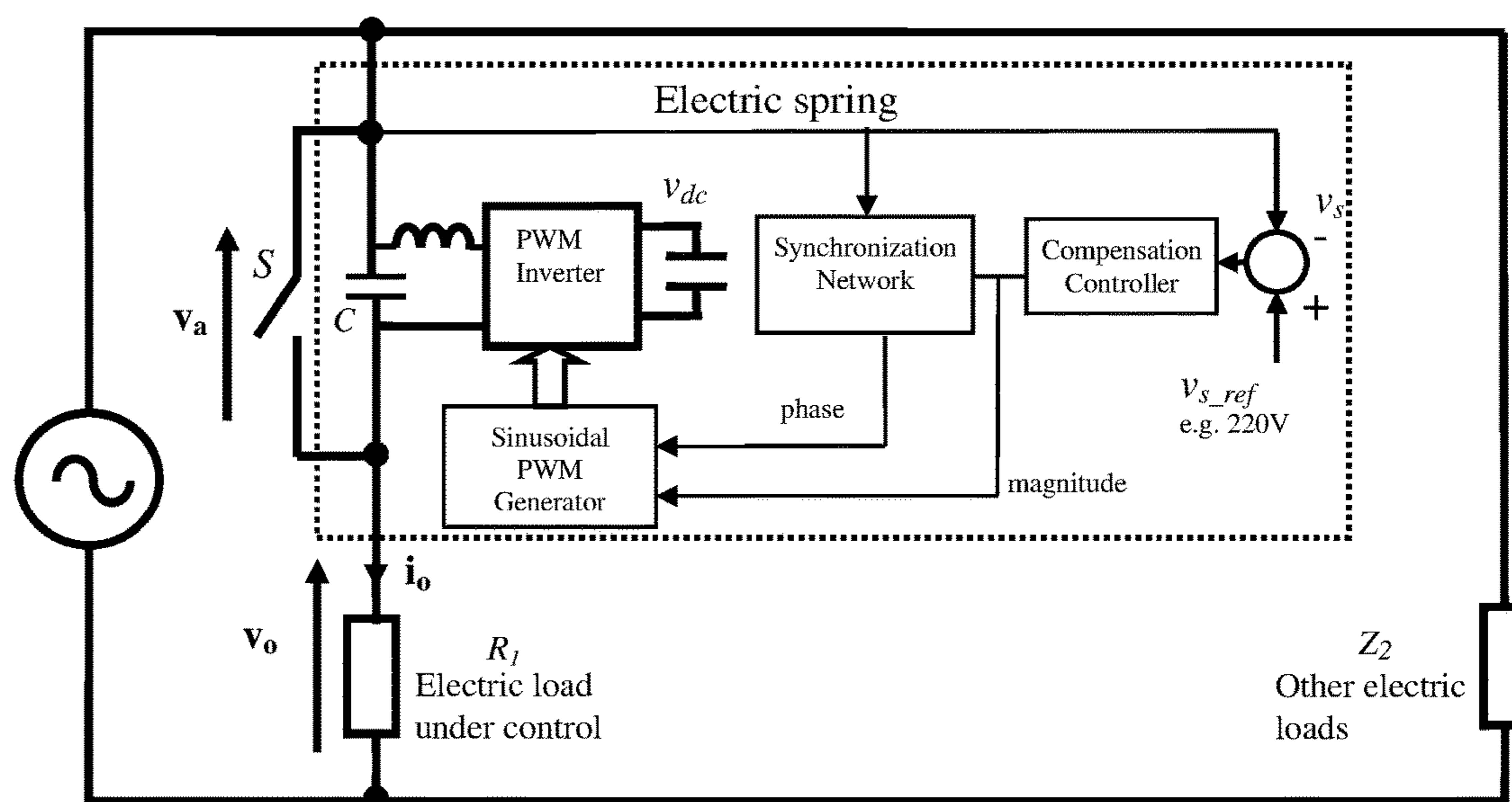
FIG. 1 (Prior Art)
