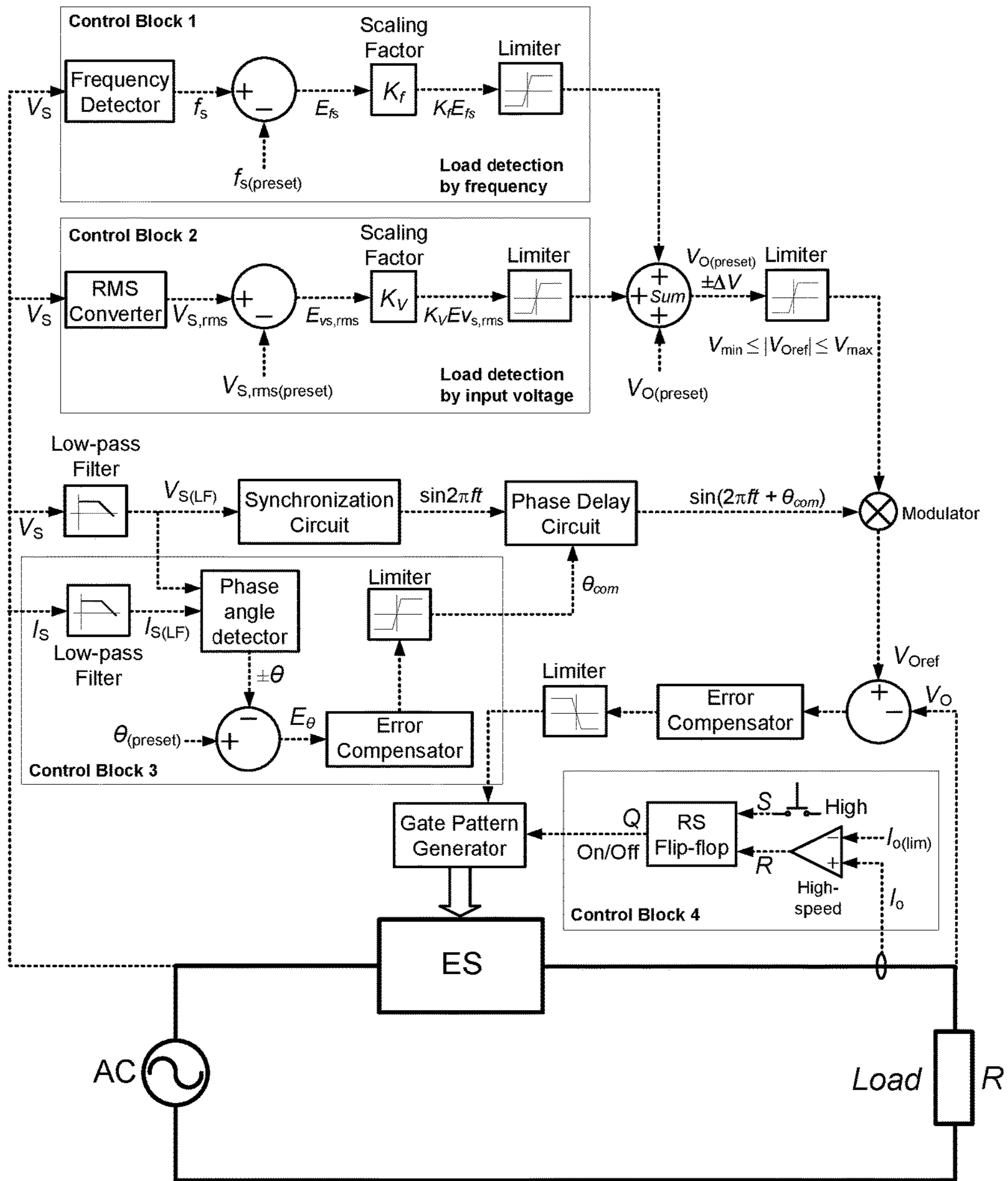
FIG. 5 (Prior Art)
