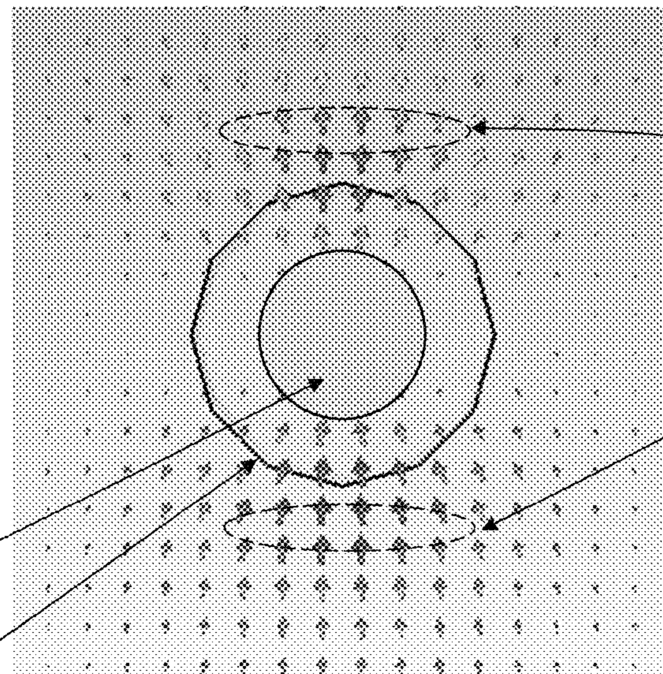
FIG. 20L HE Wave Mode (Large Mode Size)
