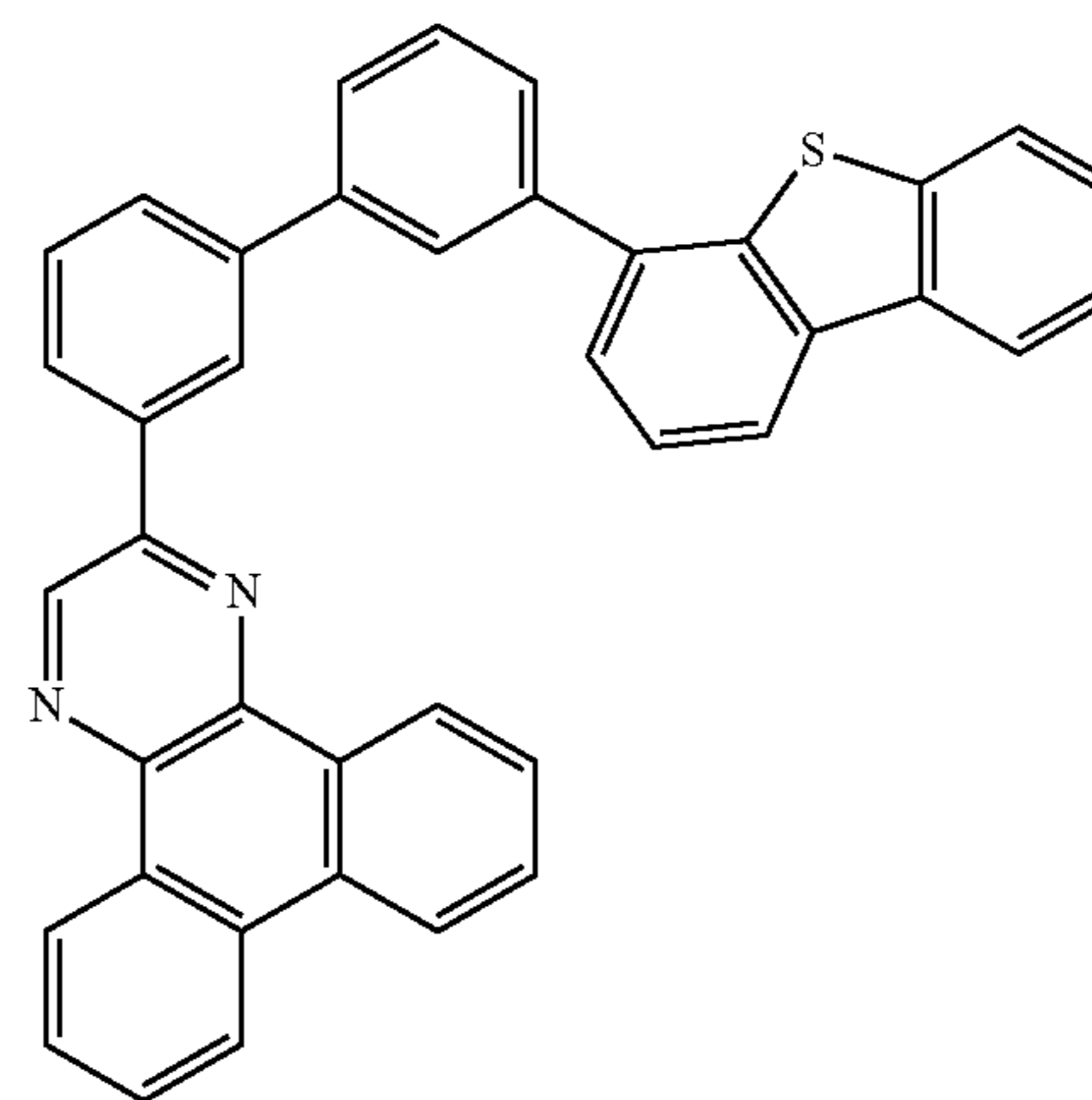
2mDBTBPDBq-II
