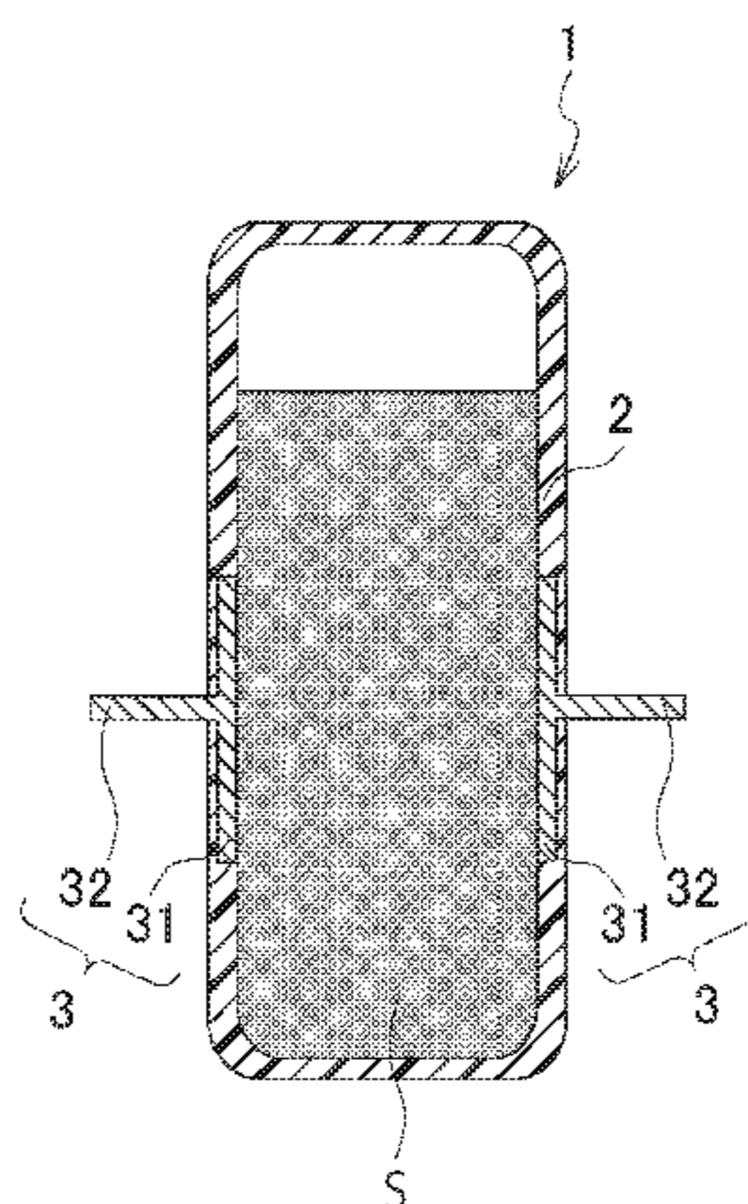
1: ELECTRICAL MEASURING CONTAINER 2: BIOLOGICAL SAMPLE HOLDING SECTION 3: ELECTRICAL CONDUCTIVE SECTION 31: ELECTRODE SECTION 32: CONNECTING SECTION S: BIOLOGICAL SAMPLE
