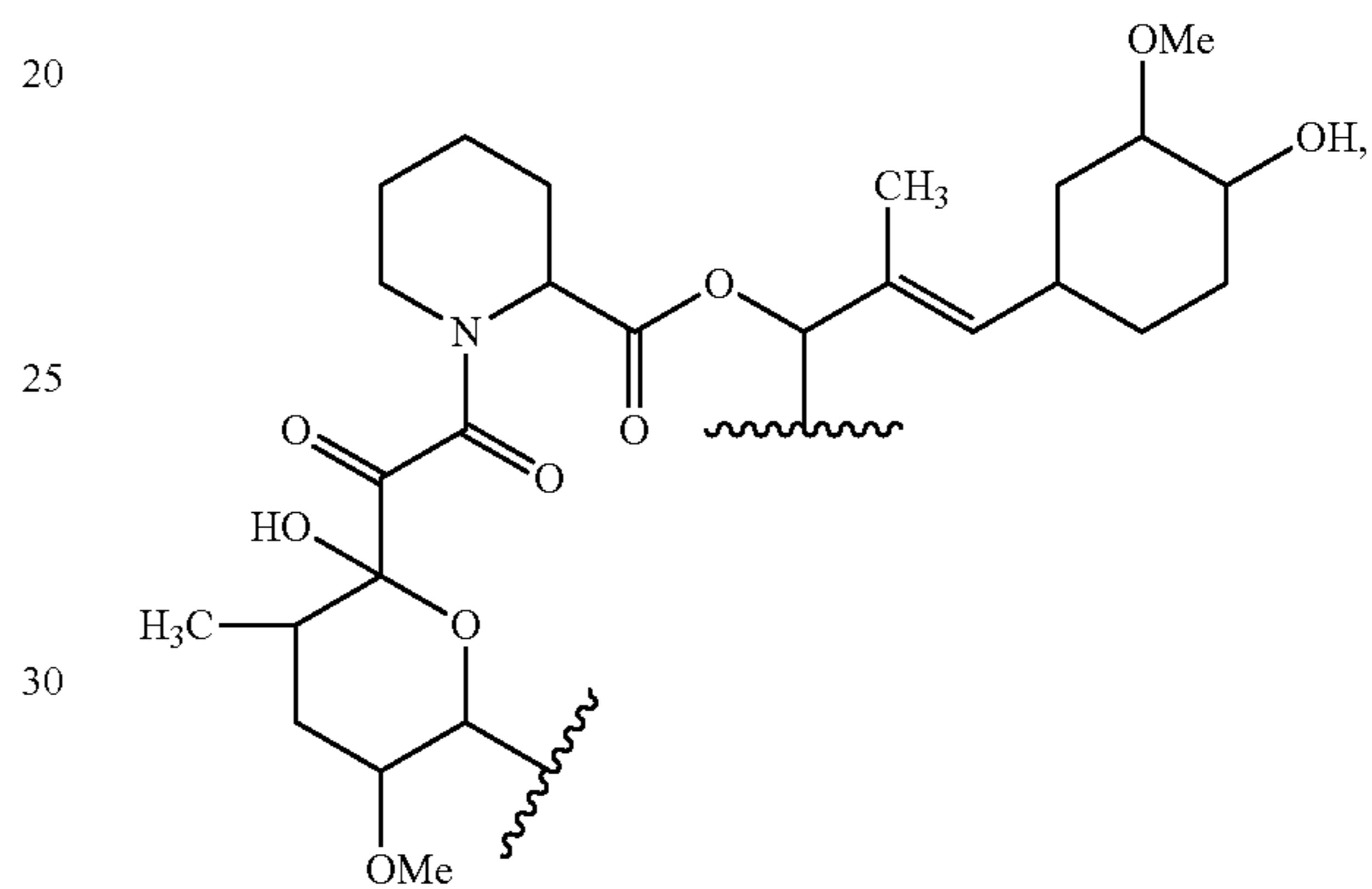
Formula IIa
