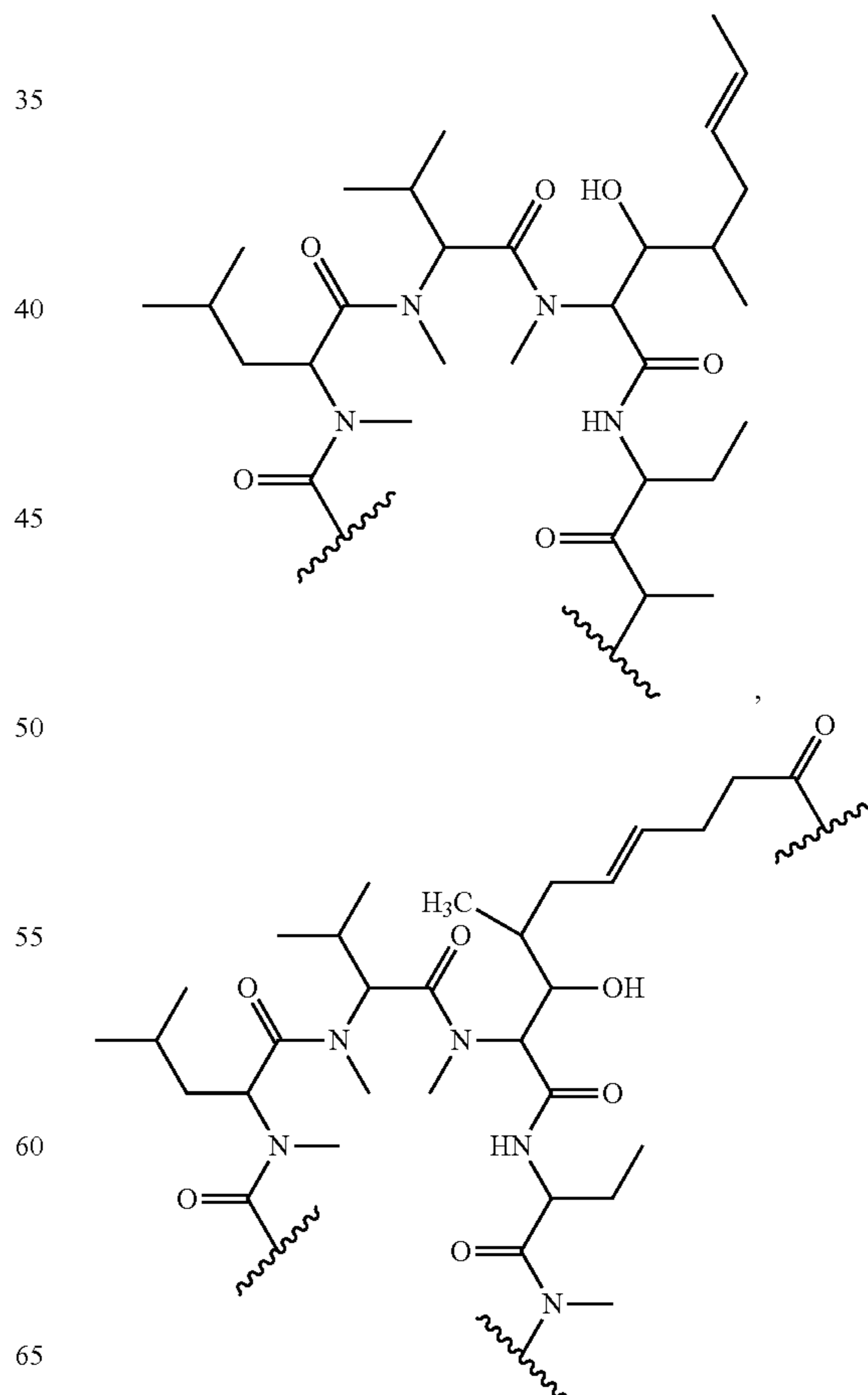
Formula IV
