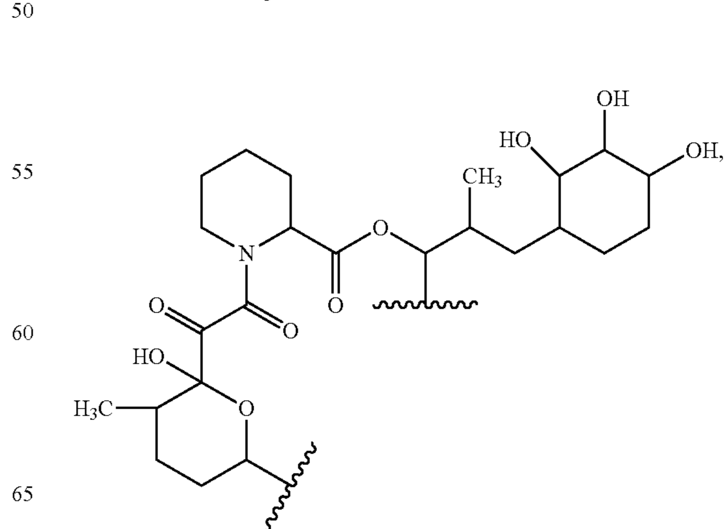
Formula IV
