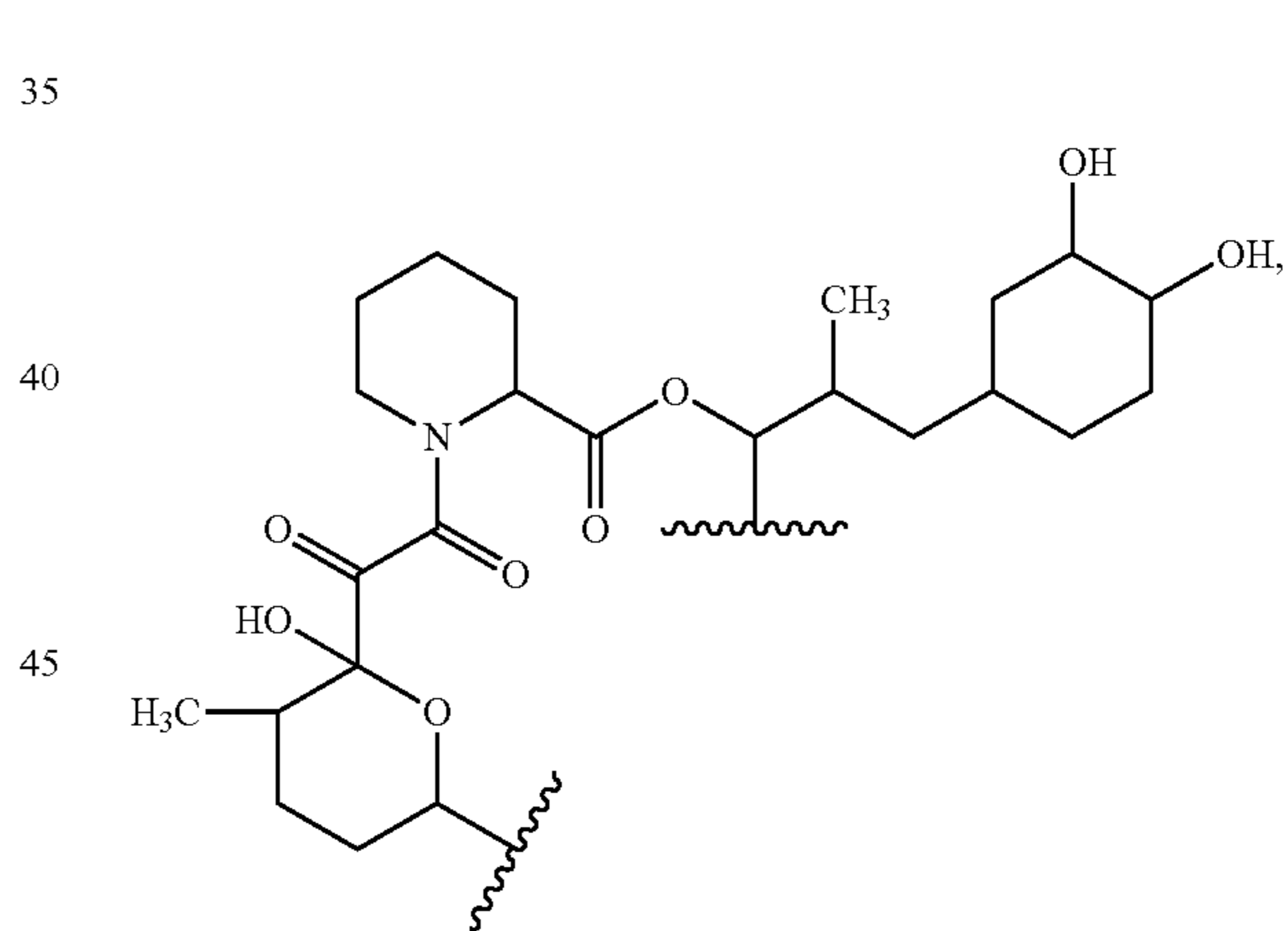
Formula III
