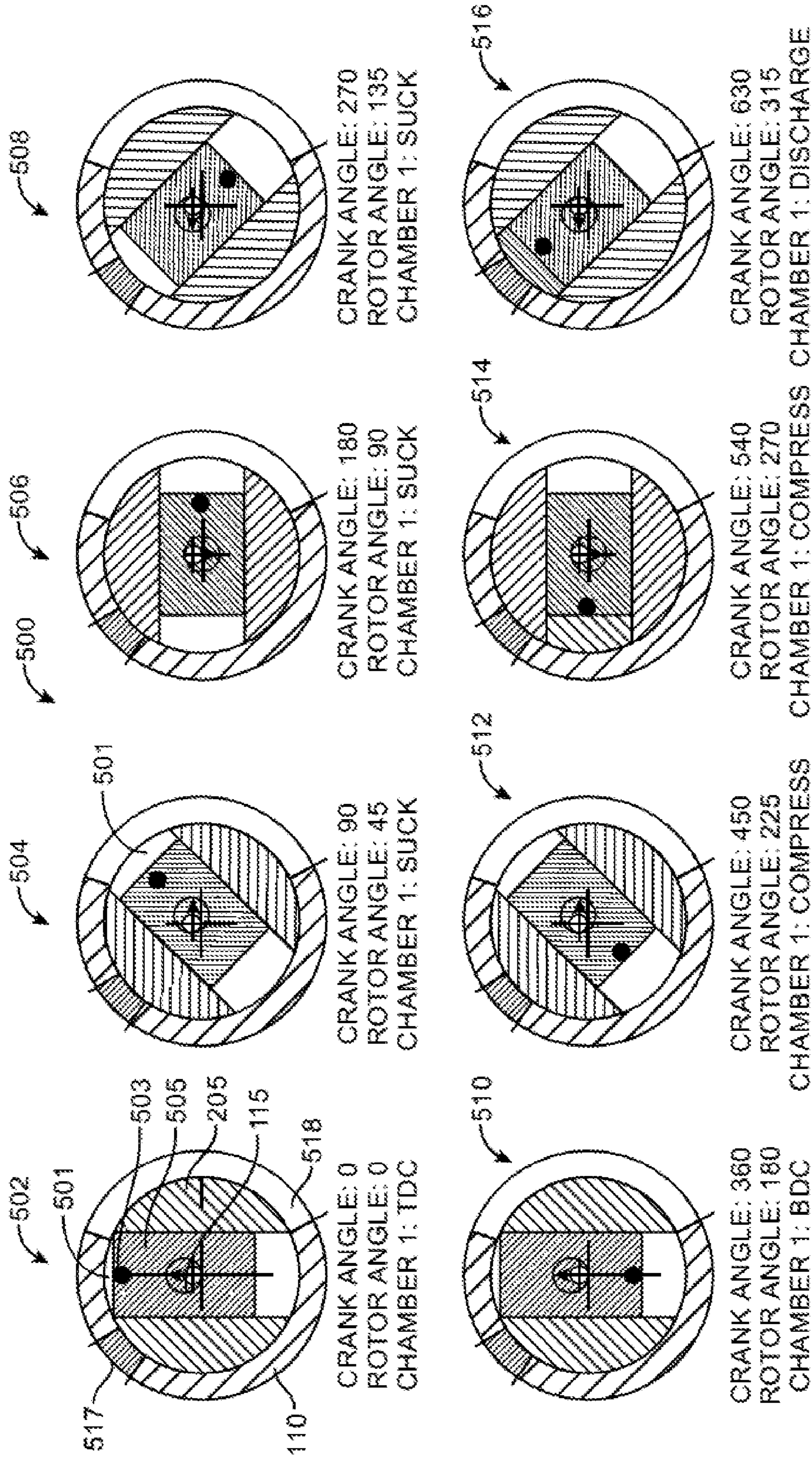
SPUN-EPICYCLIC PUMP-COMPRESSOR
