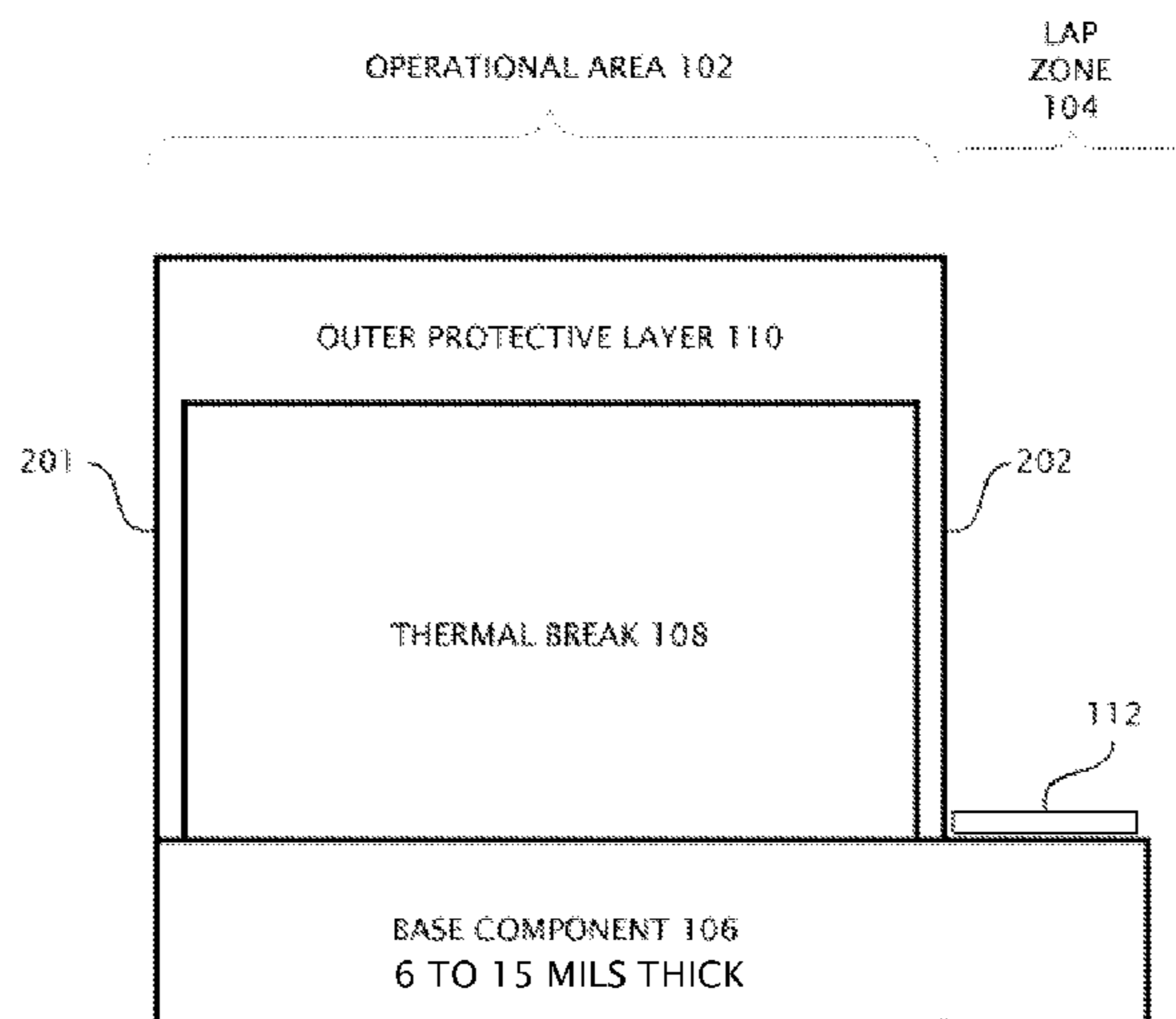
SIDE VIEW OF UNIVERSAL BARRIER COMPONENT 100
