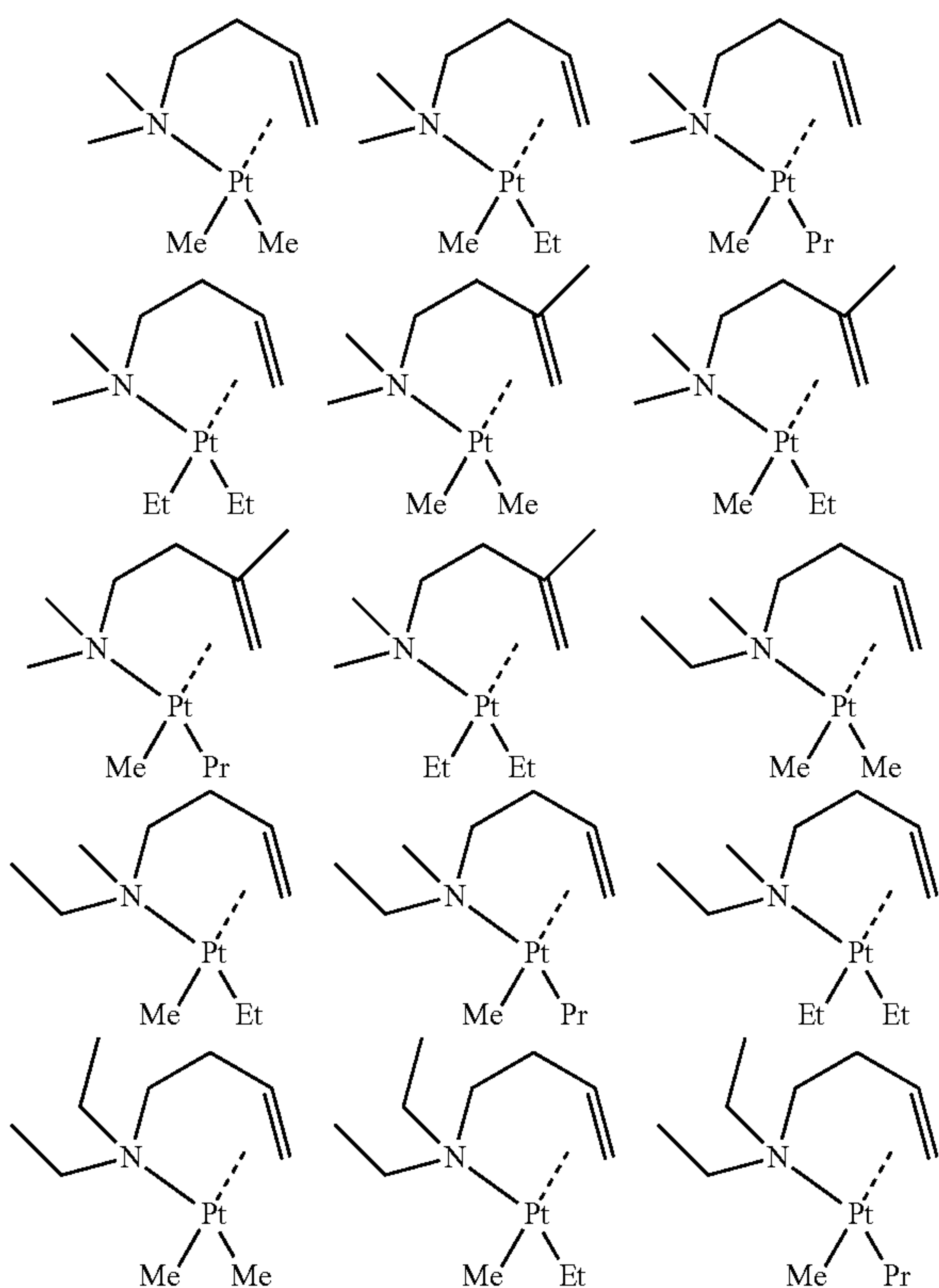
[Chemical Formula 7]
