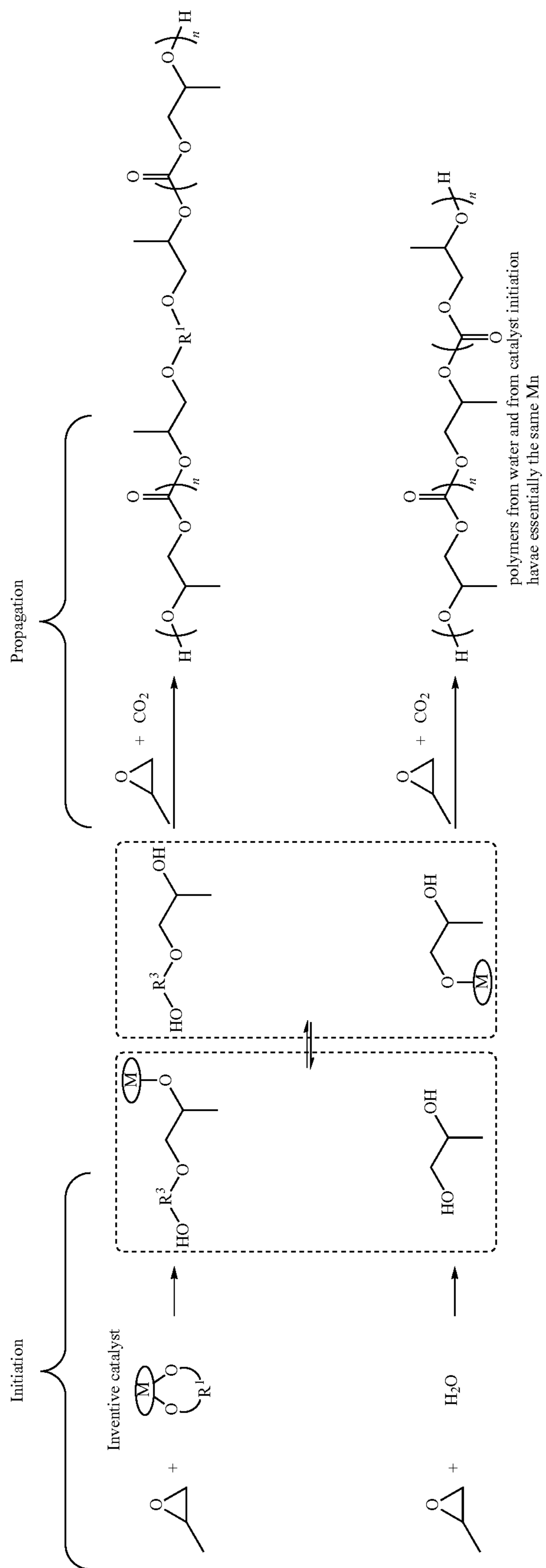
Scheme 2
