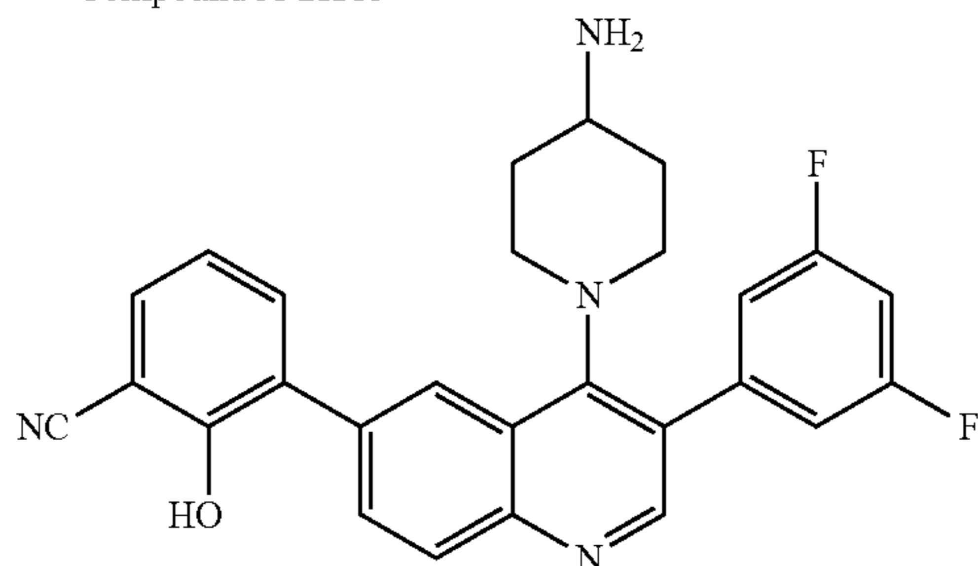
Compound A-2HCl
