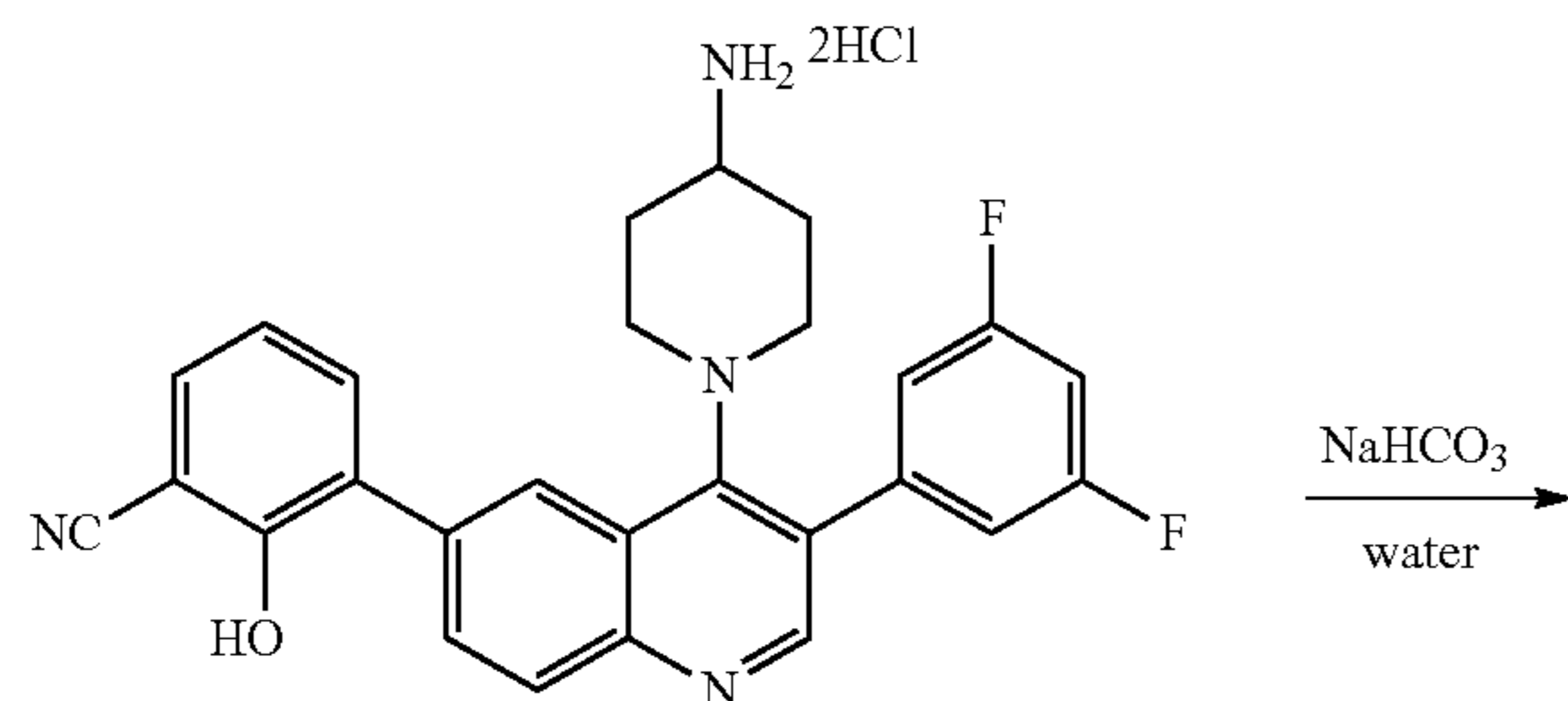
Compound A-2HCl
