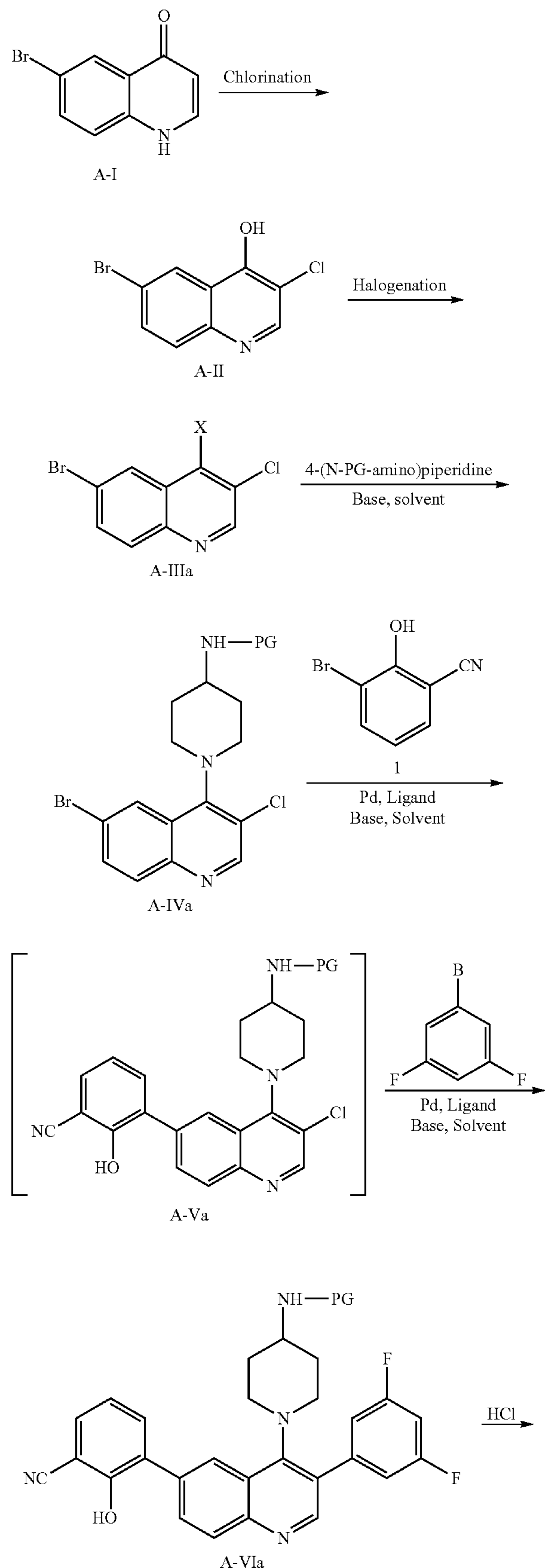
Scheme A
