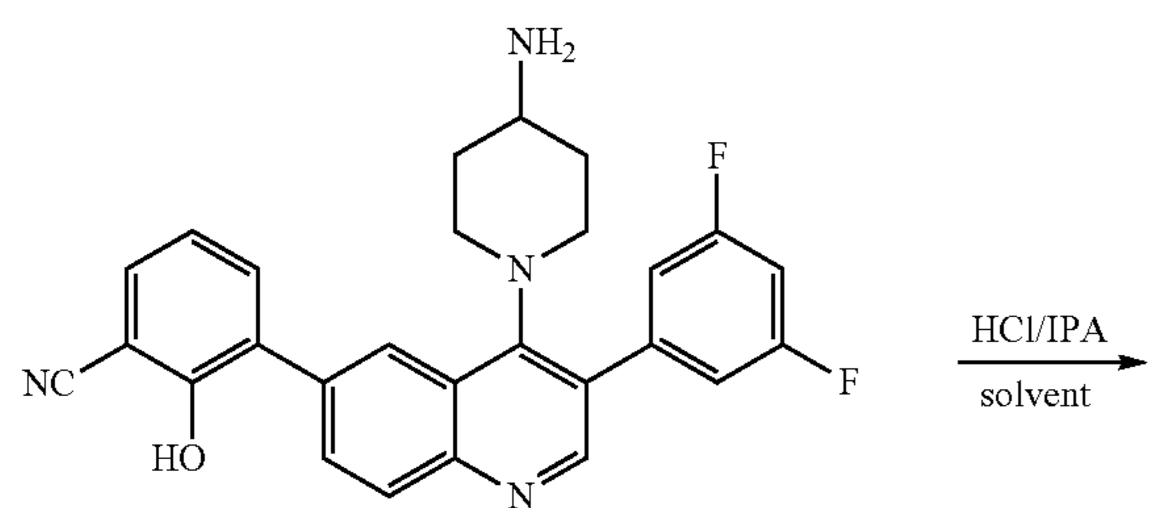
Compound A
