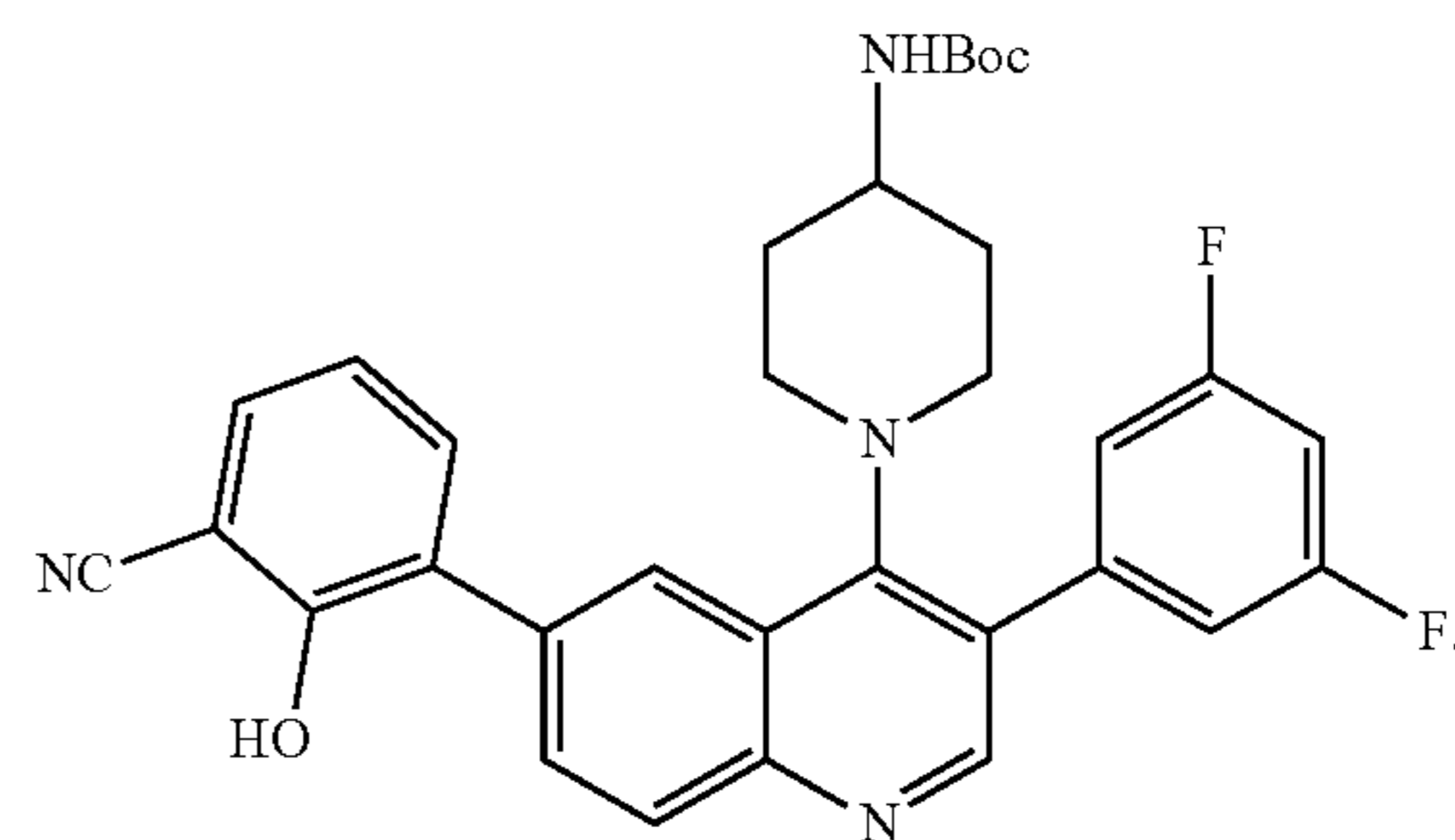
Compound A-VI
