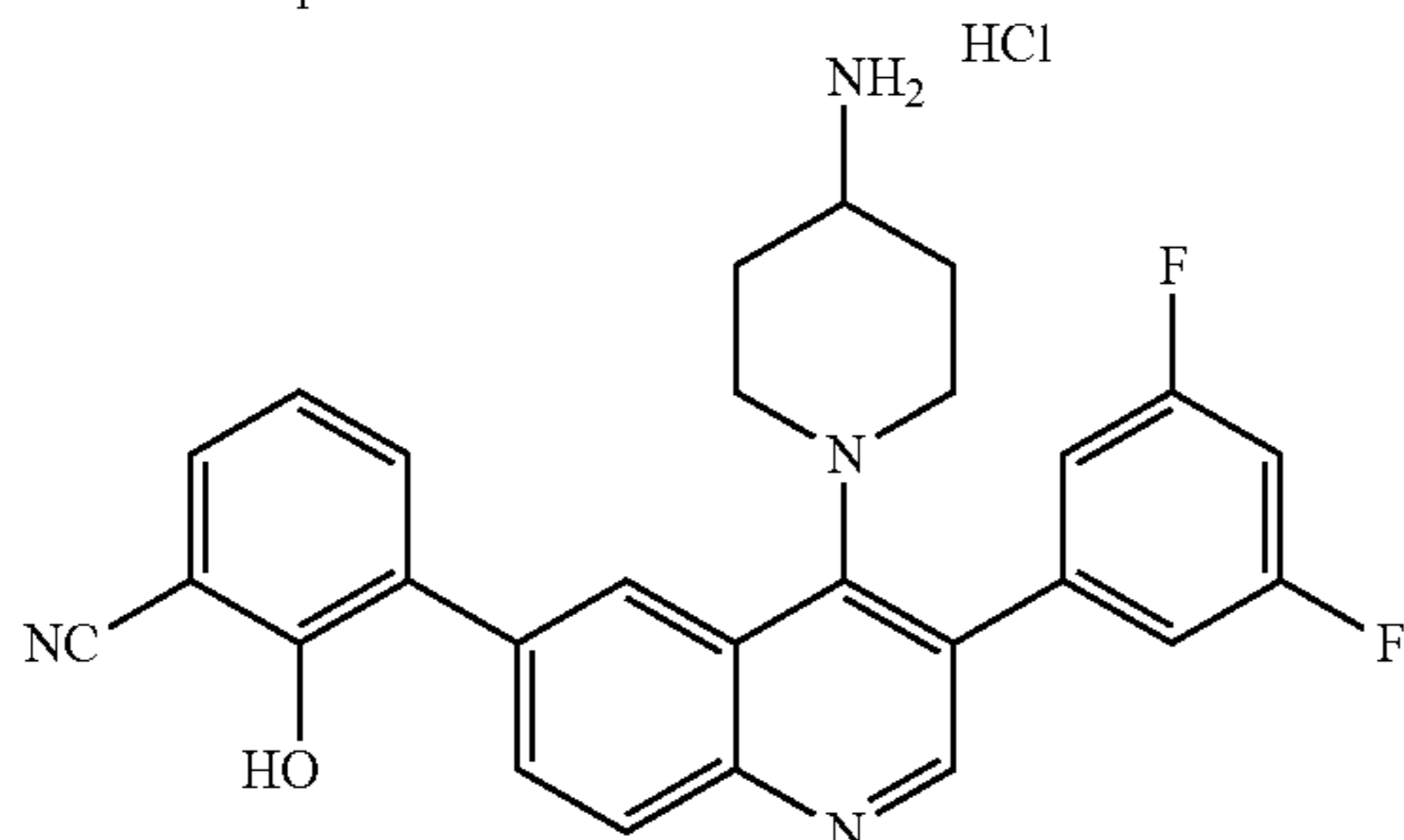
Compound A
